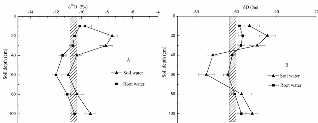
430 Fig.3 Isotope profiles of \delta^{18}O and \delta D (piston-type flow) in soil water and xylem water. Values are meas \pm standard deviation
