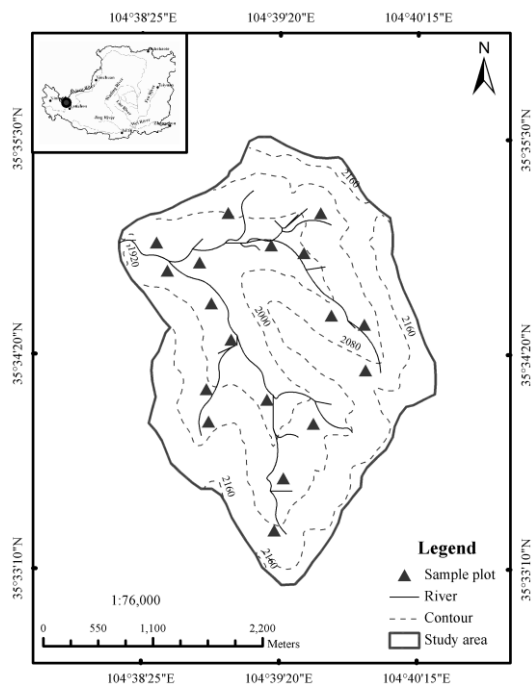
Fig.1 Location of the sampling sites in the study area
