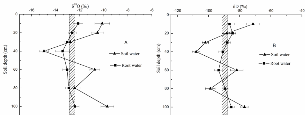
Fig.4 Isotope profiles of \delta^{18}\text{O} and \delta\text{D} (preferential flow) in soil water and xylem water. Values are \text{meas} \pm standard deviation
