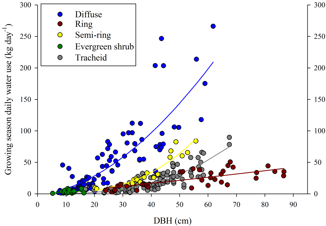
Fig. 6. Growing season dail water use of tree species
