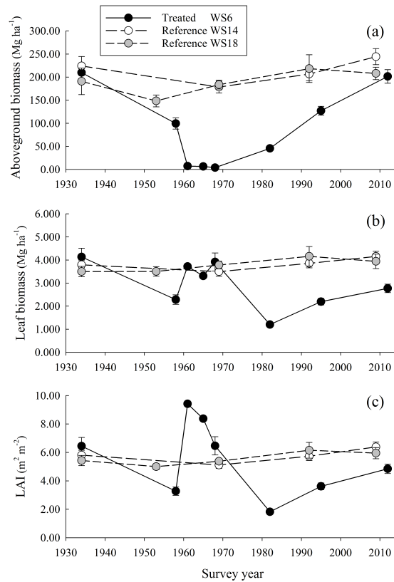
Fig. 2. Mean (a) aboveground biomass, (b) leaf biomass
