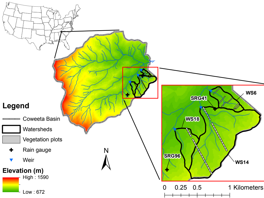
Fig. 1. Map of the Coweeta Basin
