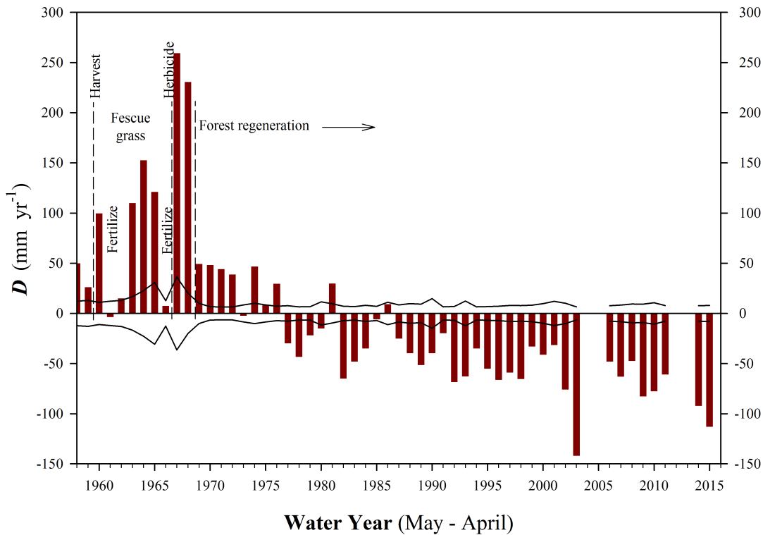
Fig. 4. Changes in water yield
