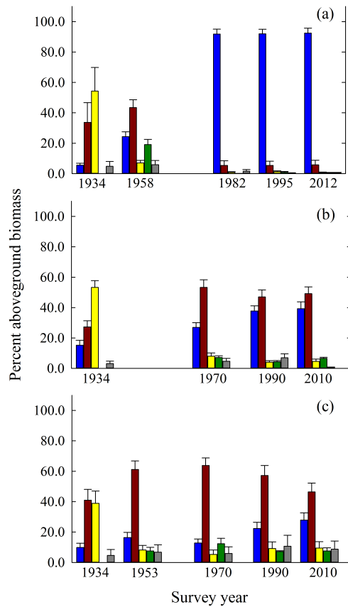
Fig. 3. Percetn aboveground biomass for the xylem
