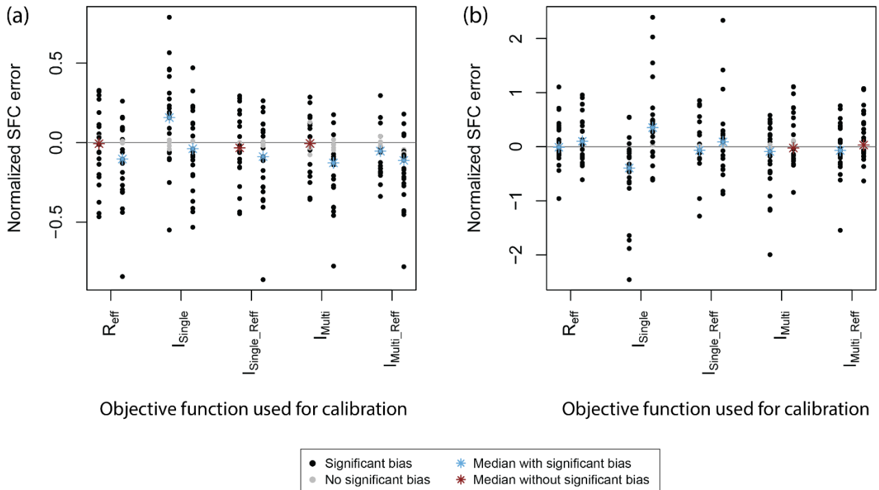
Figure 9. a) Normalized DH16 errors (nSFC) and b) normalized MH10 errors (nSFC) in validation depending on the objective function used in calibration. Normalized SFC errors are shown for all 25 catchments and for both modelling time periods (period 1 (1984 - 1996) on the left side and period 2 (1997 - 2009) on the right side). Colours indicate the significance of the results assessed by a two-sided binomial test at a confidence level of 0.95. Note the difference in the y-axis.
