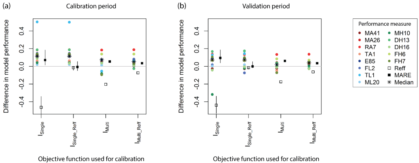
Figure 4. Model performance in a) calibration and b) validation for absolute normalized SFC errors (nSFC) as well as R_{eff} and MARE depending on the objective function used in calibration. Model performance is shown as the difference between a model calibration with R_{eff} and model calibrations with I_{Single} , I_{Single\_Reff} , I_{Multi} or I_{Multi\_Reff} (positive values indicate that model calibration with I_{Single} , I_{Single\_Reff} , I_{Multi} or I_{Multi\_Reff} resulted in better model performance than model calibration with R_{eff} ; negative values indicate that model calibration with I_{Single} , I_{Single\_Reff} , I_{Multi} or I_{Multi\_Reff} resulted in poorer model performance than model calibration with R_{eff} ). Model performance values correspond to the median of the 25 catchments and the mean of both modelling time periods.
