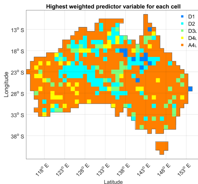
10 Figure 5: The variable with the highest relative weight in the regression for each cell across Australia. A4 is most dominant, however D2 is prominent in distinct areas throughout central Australia. D1, D3 L and D4 L all occur but with little spatial coherence.
