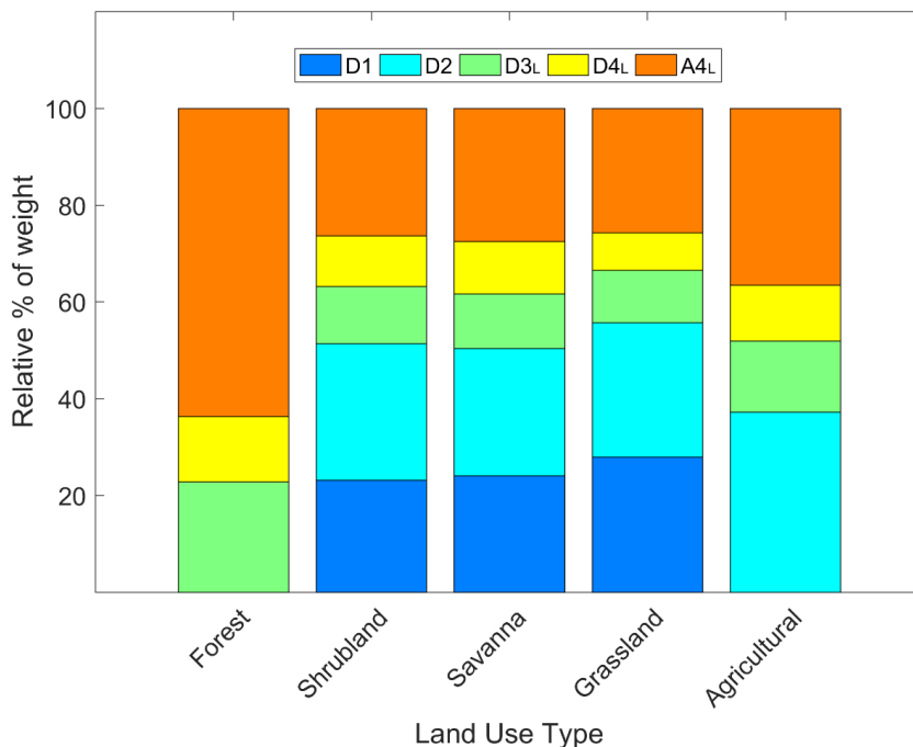
Figure 6: The relative weight of each decomposed TWS* for each land use type. Forests are A4 L dominated, shrublands, savannas and grasslands are very similar with relative equal weights of D1, D2 and A4 L , while agricultural land is dominated by D2 and A4 L .
