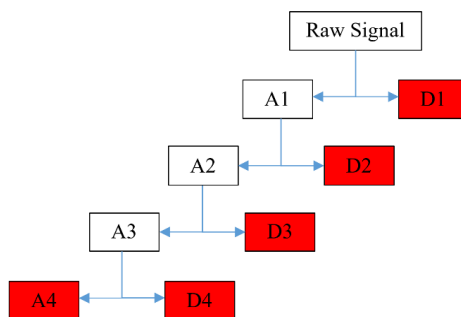
Figure 2: The structure of a wavelet decomposition; decomposition levels used in this study are highlighted in red.
