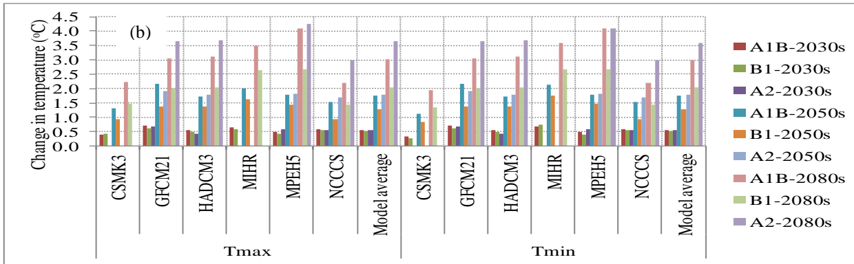
Figure 4: (a) Relative change mean annual precipitation and (b) change in Tmax and Tmin modeled from six GCMs for three time periods of UBNRB as compared from the reference period of 1984-2011 by using LARS-WG
