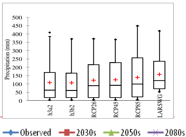
Figure 11: Comparison of climate change scenario a) downscaled using LARS-WG and SDSM from HadCM3 GCM for a2 scenario b) downscaled from different scenarios (LARS-WG using hadCM3 a2 scenario)
