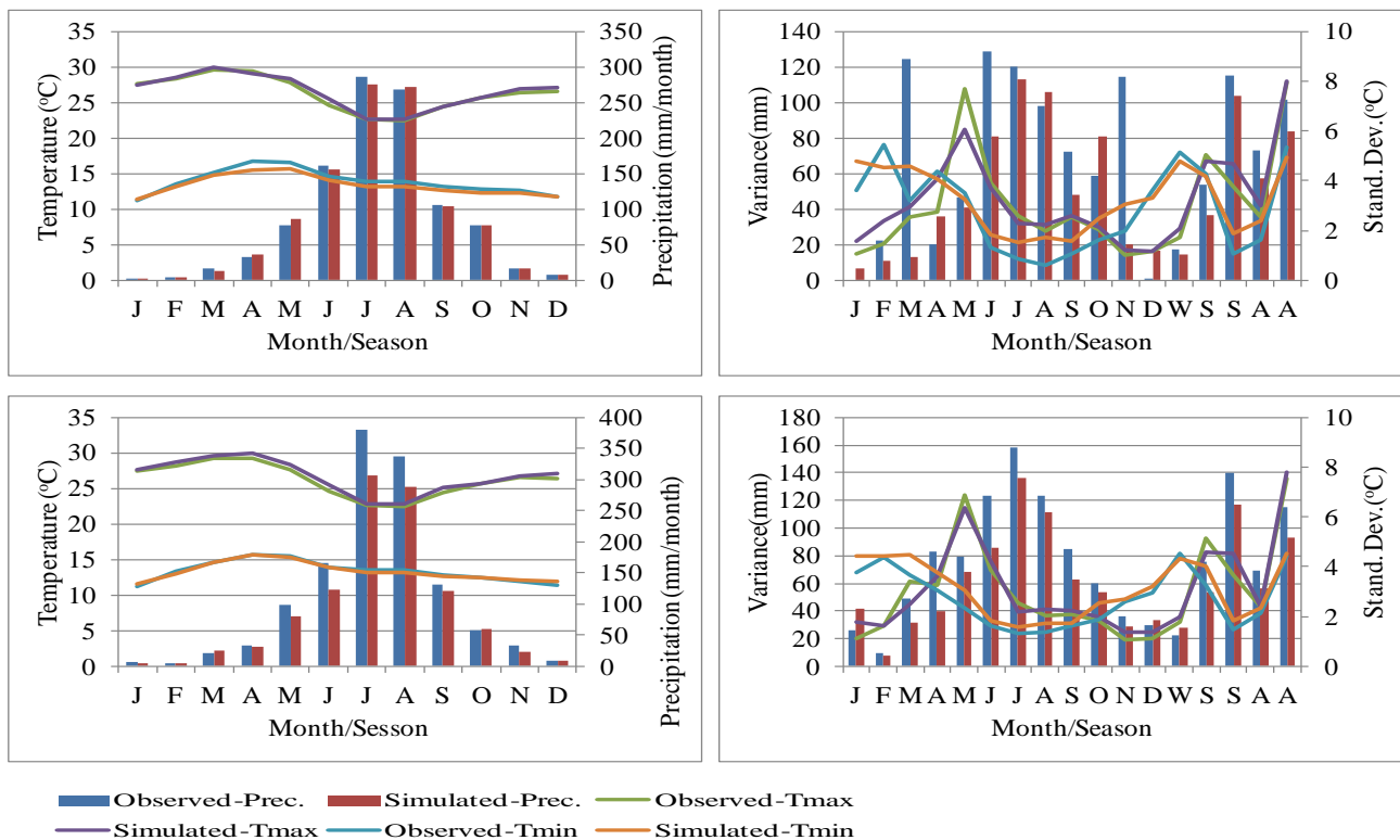
5 Figure 7 : Validation of observed and simulated of precipitation, maximum and minimum temperature for Gondar station using SDSM from canESM2 and HadCM3 from top to bottom respectively
