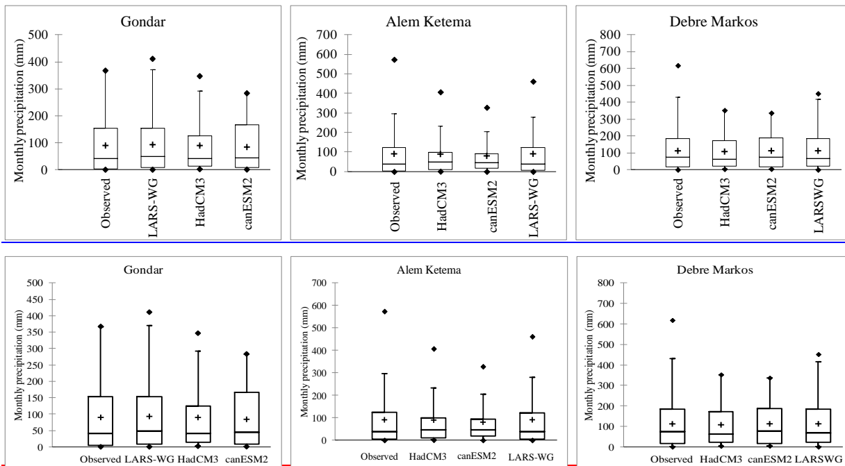
Figure 10 :Box plot showing the model performance at for three stations at monthly basis . Box boundaries indicate the 25 th and 75 th percentiles, the line within the box marks the median, whiskers below and above the box indicate the 10 th and 90 th percentiles, dots indicate the extremes.
