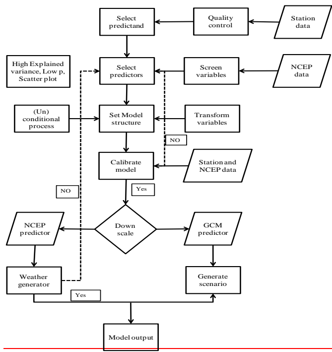
Figure 2: Schematic diagram of a) LARS WG analysis b) SDSM analysis source (Wilby et al. , 2002)
