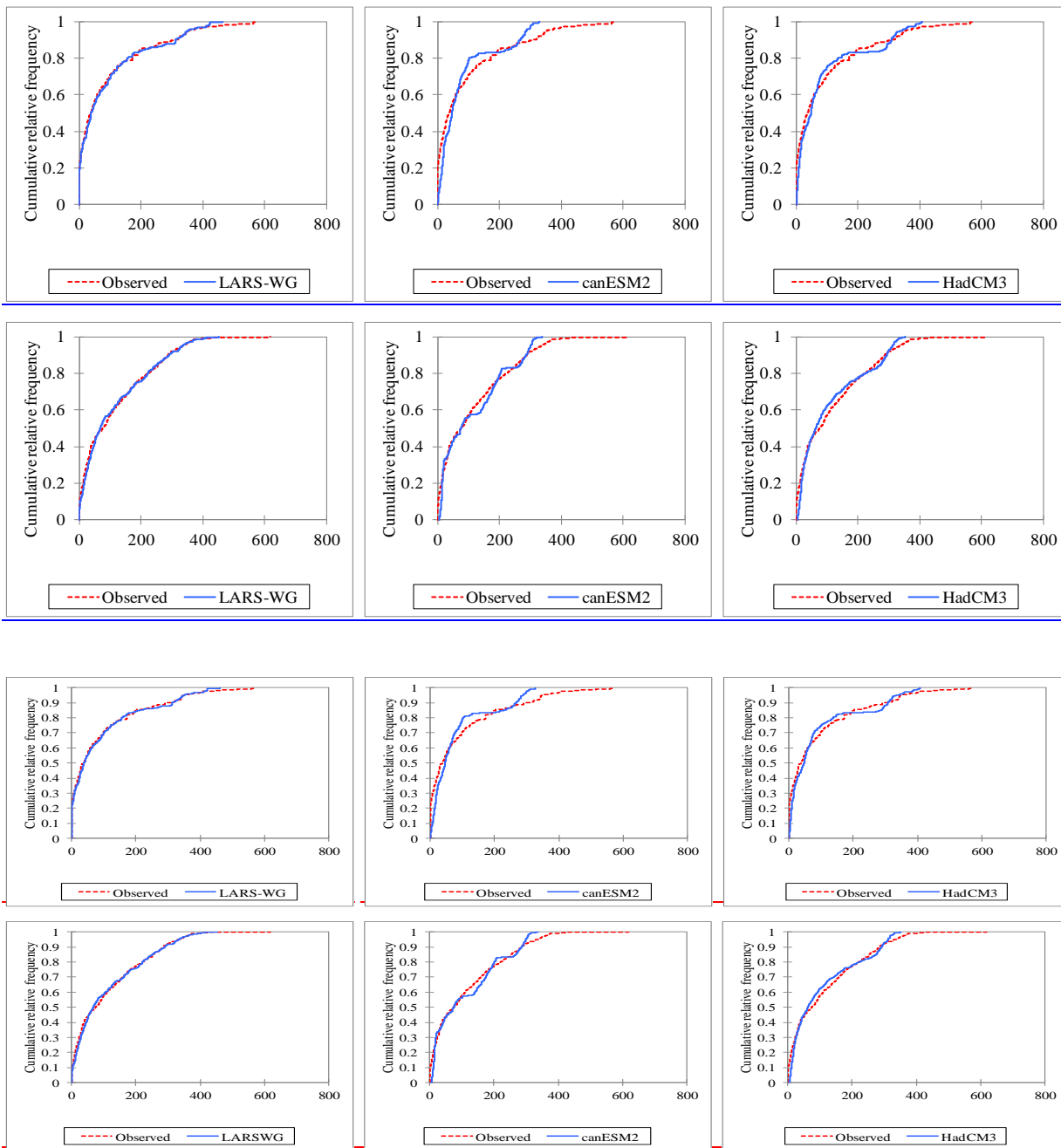
-Figure 9 :Kolmogorov-Smirnov test to compare the skill of the models for the observed precipitation distribution (Upper three Alemketema station, lower three Debre markos station)
