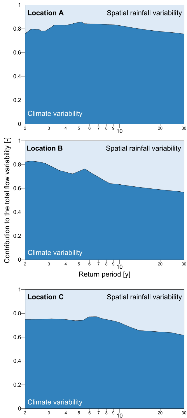
Figure 8. The ratio between the climate variability and the total flow variability for a given return period and for different locations within the urban drainage system is represented in dark blue. The remaining contribution is due to the addition of spatial rainfall variability (light blue).
