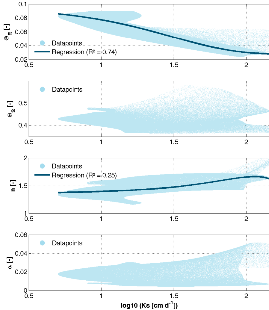
Figure 5. Scatterplots of the van Genuchten parameters ( \Theta_R , \Theta_S , n , \alpha ) in dependency of the saturated hydraulic conductivity ( Ks ). Visualized is database 1 ( \Theta_R - Ks ) and database 2 ( \Theta_S - Ks , n - Ks and \alpha - Ks ). A regression function with a coefficient of determination ( R^2 ) of 0.74 was fitted between \Theta_R and Ks . Furthermore, a regression function with an R^2 of 0.25 was fitted between n and Ks . \Theta_S - Ks as well as \alpha - Ks showed no correlation.
