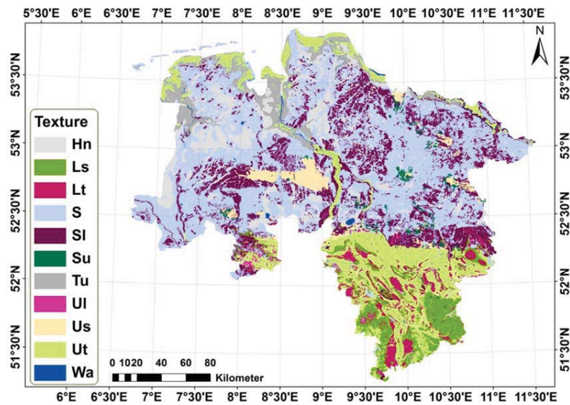
Figure 1. Soil map of Lower Saxony, Germany (Edt.: J. Boess et al., 2004). Ls = sandy loam, Lt = clayey loam, S = sand, Sl = loamy sand, Su = silty sand, Tu = silty clay, Ul = loamy silt, Us = sandy silt, Ut = clayey silt, see Table 1. In addition to that, "Hn" stands for boggy soils and "Wa" stands for water bodies (lakes, rivers).
