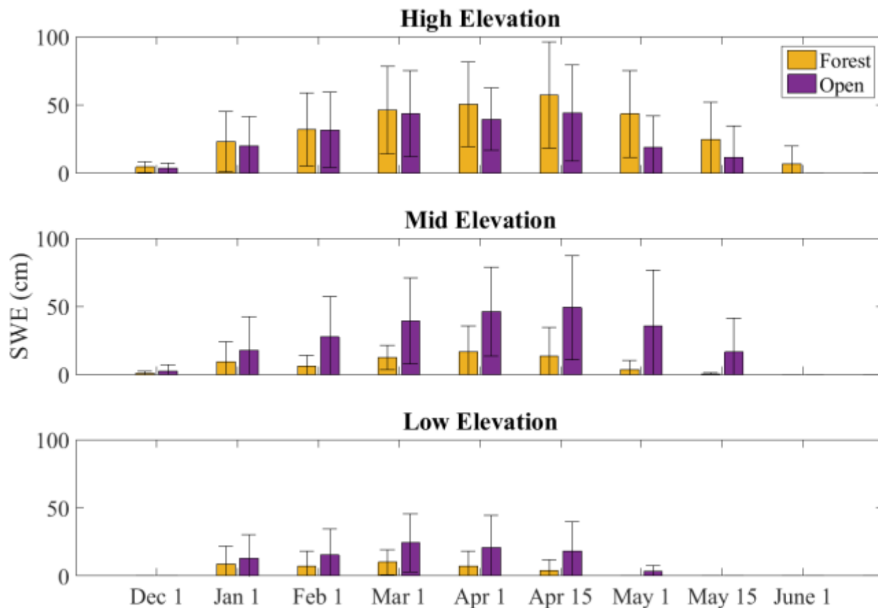
Figure 2: Average snow water equivalent (SWE) for Open and Forest sites within the ForEST network.
