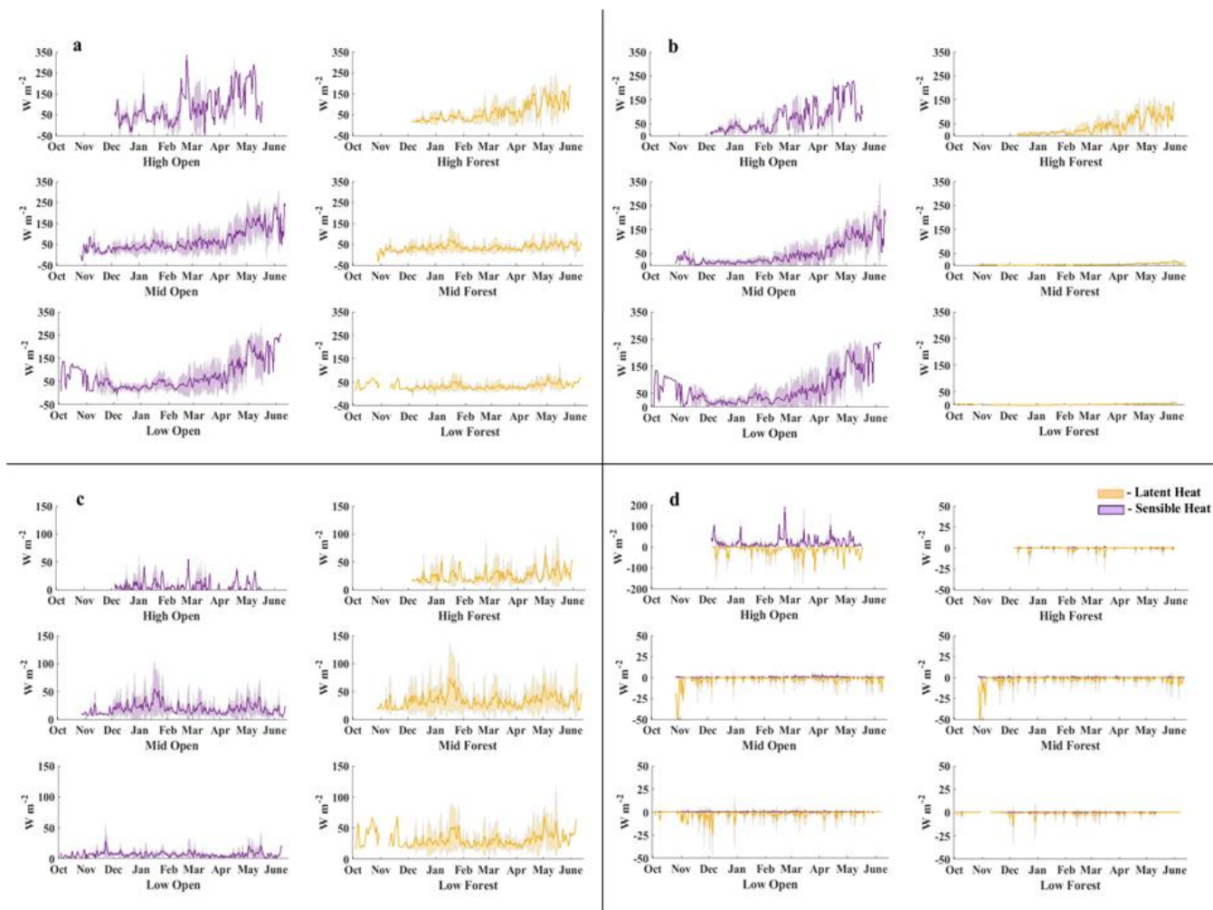
Figure 4: Calculated daily mean energy balance (solid line) and the range of values for the study duration (shaded area) for a) net energy at the snow surface; b) net solar radiation; c) net longwave radiation; and d) net turbulent energy at the snow surface for each site within the ForEST network.
