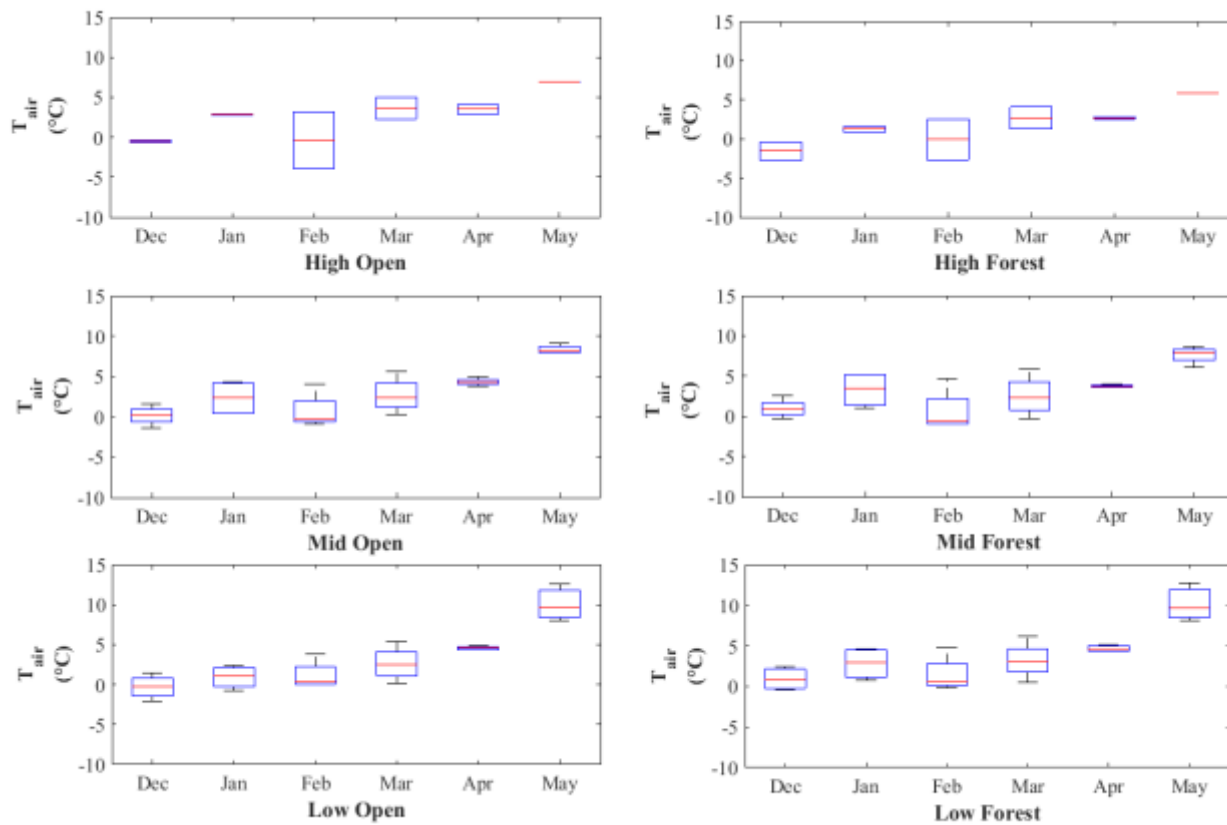
Figure 5: Mean monthly air temperature for each site within the ForEST network.
