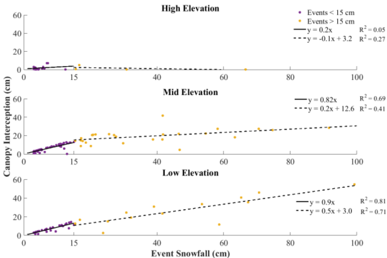
Figure 3: Canopy interception vs. event snowfall within the ForEST network.
