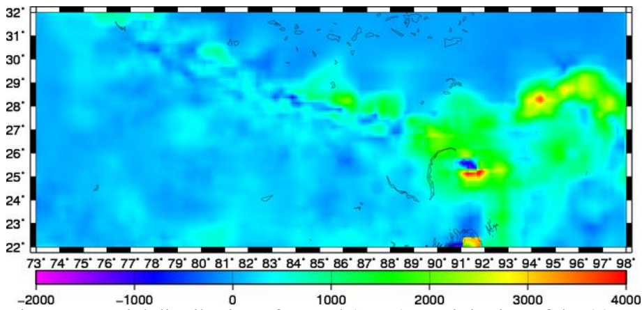
Figure 1 Spatial distribution of annual (1988) precipitation of the (a) WFD and the (b) APHRODITE over entire GBM basin and (c) difference between two data.
