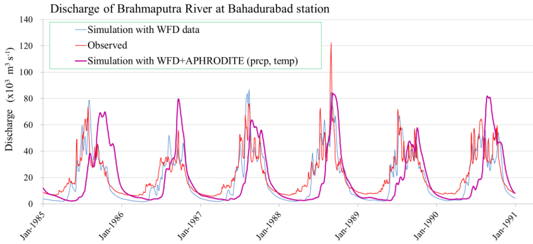
Figure 2 Time series plot of simulated discharge using both (i) complete dataset from the WFD and (ii) combination of precipitation and temperature data from the APHRODITE dataset and other metrological variables from the WFD
