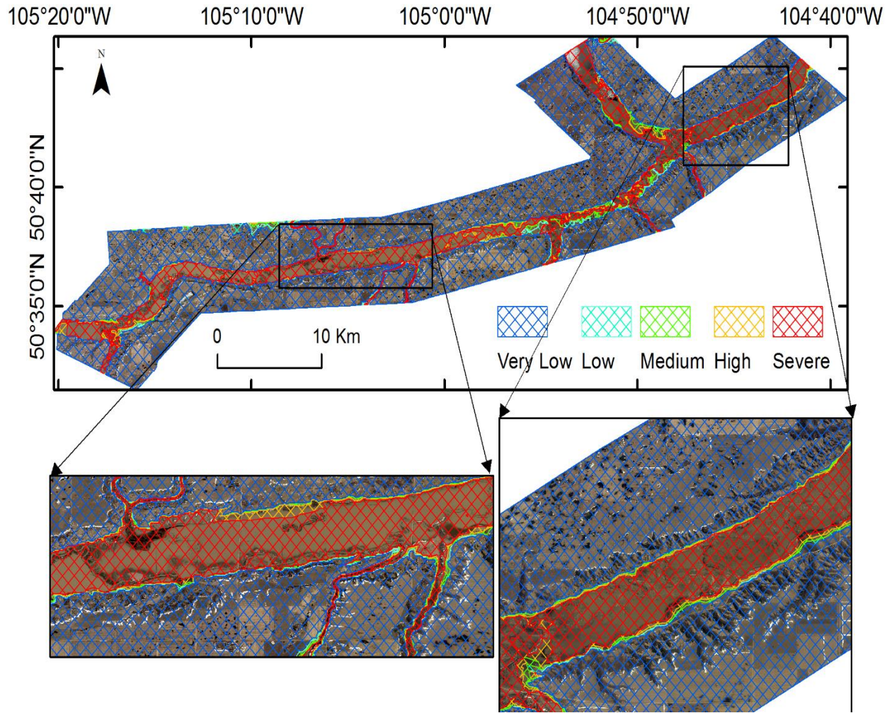
Figure 5: Comparison of hazard map with aerial image of a single flood event on the Qu'Appelle River, Saskatchewan (background). Date of image: 06/05/2013
