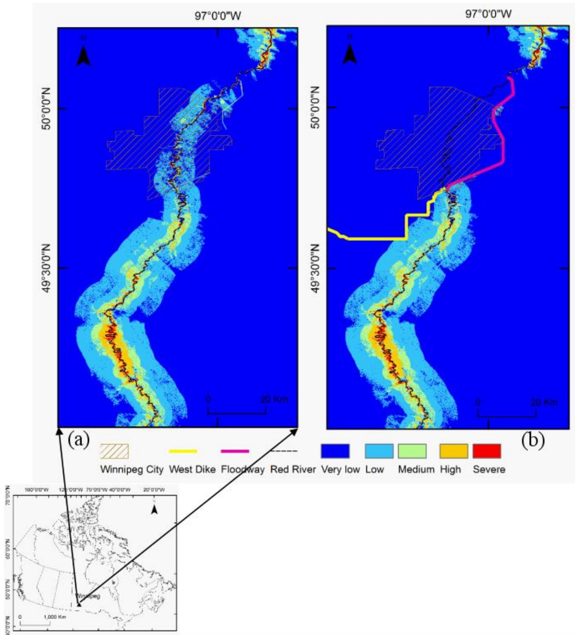
Figure 6. Hazard map for the Red River in Manitoba: (a) without considering flood protection structures in delineating hazard zones and (b) considering flood protection.
