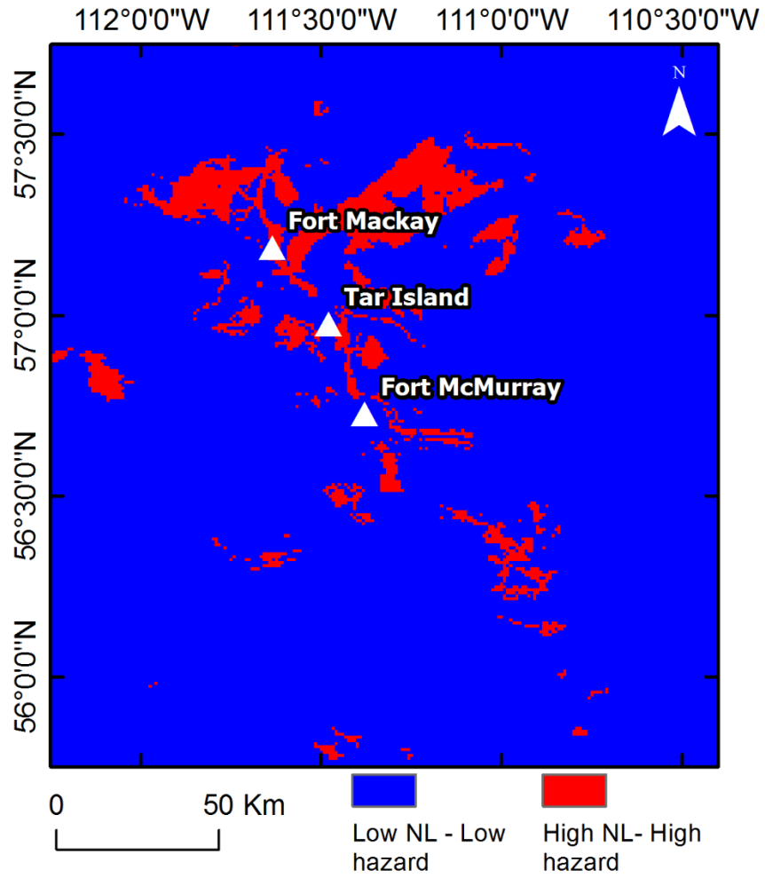
Figure 1: Locations indicating increase in nightlight (NL) activity over high hazard areas between the years 1992 – 2013 ( DN_{2013} - DN_{1992} )
