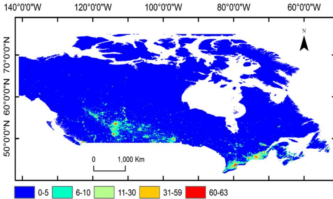
Figure 2: Nightlights over Canada shown as (a) Continuous spectrum and (b) classified as shown in Table 3 into very low luminosity (0-5), low luminosity (6-10), medium luminosity (11-30), high luminosity (31-59), and very high luminosity (60-63).
