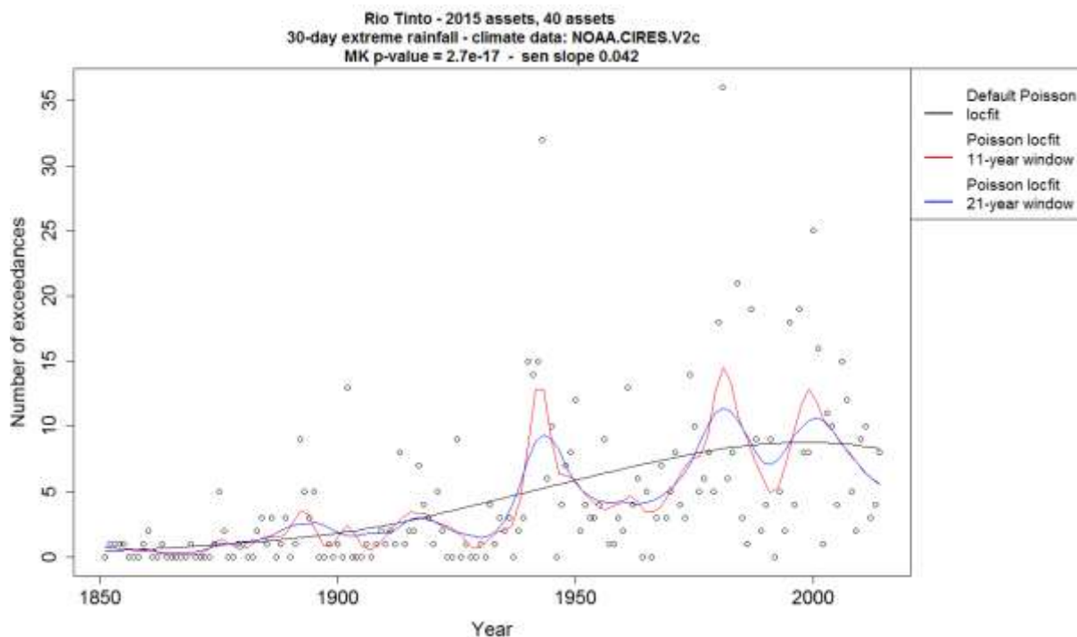
Figure 4: Time series N_t(p) of the yearly number of 30-day extreme rainfall events exceeding the 10 year return level for the Rio Tinto portfolio computed using the NOAA-CIRES 20th Century V2c dataset, using 3 windows (11, 21, and 114 years) to illustrate different aspects of long term variability
