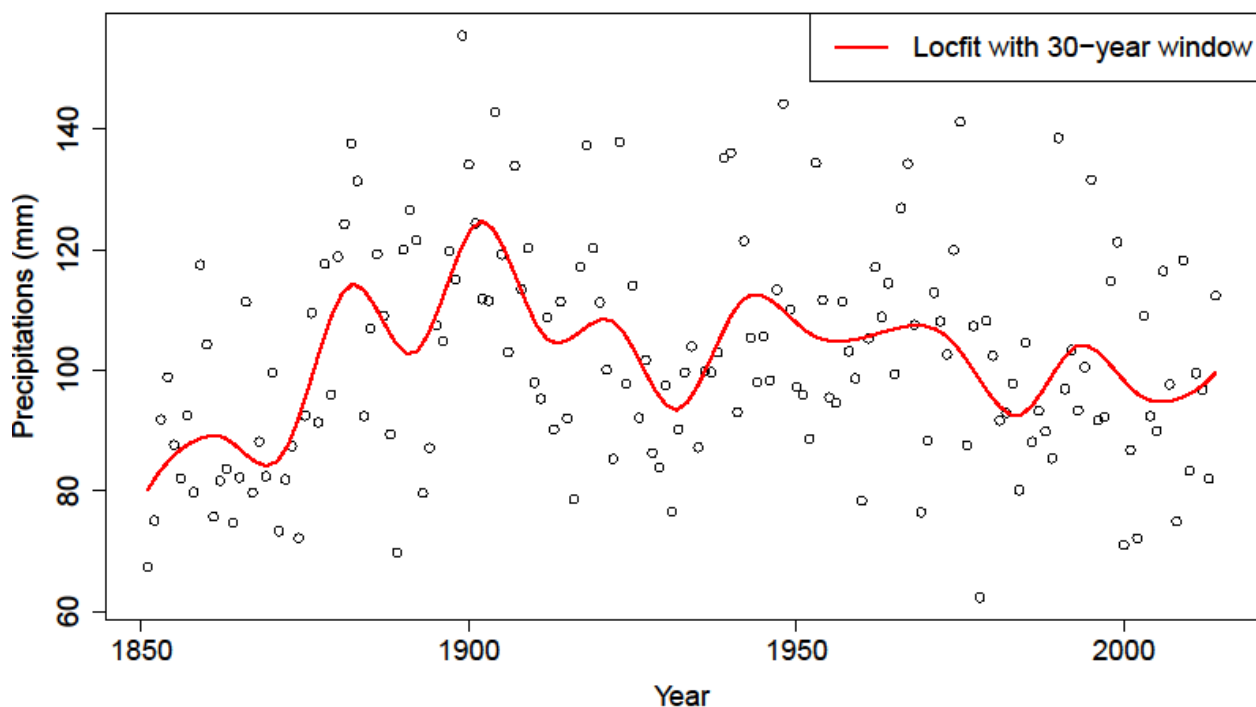
5 Figure 1: Time series of annual maximum 30 day precipitation for the Highland Valley open pit copper mine in British Columbia, at latitude 50.49°N, and longitude 121.05°W, as estimated from the NOAA-CIRES 20th century climate re-analysis. This mine is one of the largest in the region, operating since the early 20th Century. The highest precipitation for any consecutive 30 day period in
