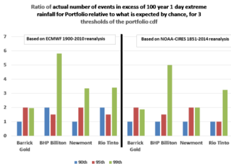
20 Figure 6: Ratio of actual number of events in excess of at site 100 year 1 day extreme rainfall for a portfolio relative to what is expected by chance based on the Poisson distribution, for 3 thresholds of the portfolio cdf
