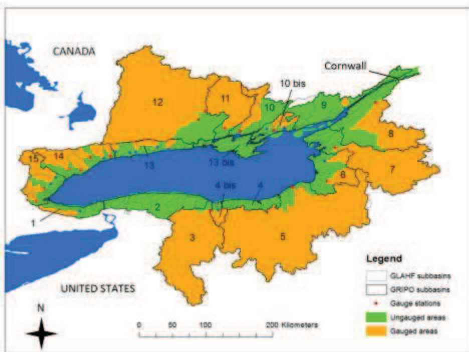
Figure 24: GRIP-O spatial framework: Lake Ontario subbasin delineation (GRIP-O subbasins). GLAHF subbasins are from the Great Lakes Aquatic Habitat Framework (Wang et al., 2015). Dots (blue for natural flow regimes and red for regulated regimes) are the most-downstream flow gauges (i.e., the main tributaries' gauges which are closest to Lake Ontario's shoreline) selected for model calibrations.
