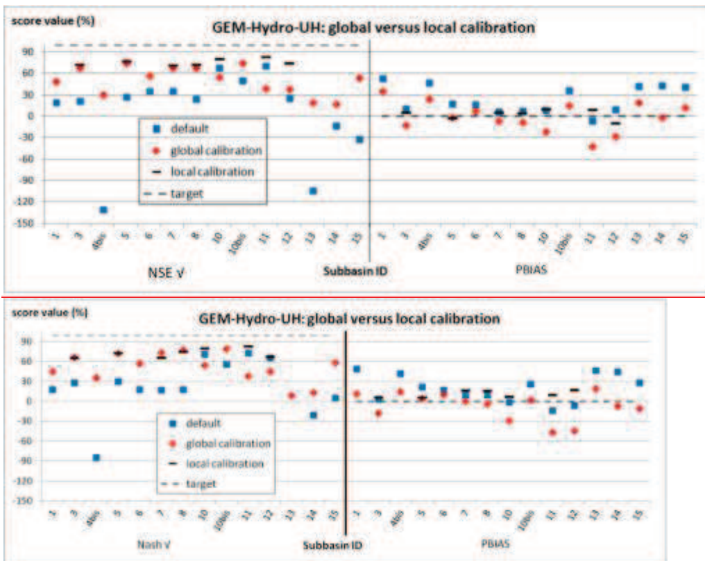
Figure 77: GEM-Hydro-UH performances in validation for the 14 GRIP-O gauged subbasins (Fig. 21) with default, locally, and globally-calibrated parameter values. Perfect scores are shown. Results are presented as NSE \sqrt{} (left) and PBIAS (right).
