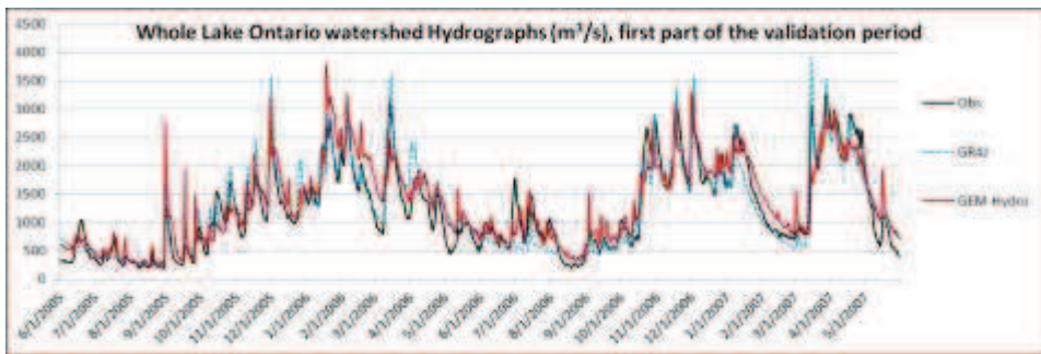
Figure 88: Lake Ontario watershed basin runoff (including its ungauged areas, Fig. 24) for the validation period, comparing GR4J and GEM-Hydro.
