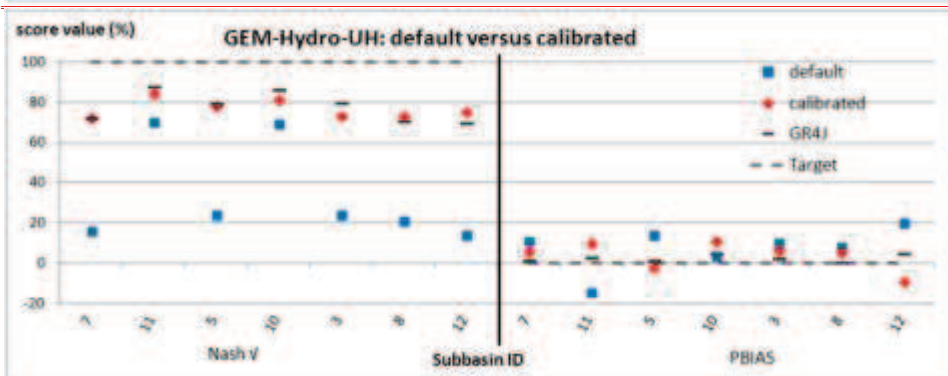
Figure 35: Uncalibrated and calibrated GEM-Hydro-UH performances over the calibration period. Results are presented as NSE \sqrt{} (left) and PBIAS (right), for many GRIP-O subbasins. The grey dashed line shows perfect scores and GR4J reference is displayed with black markers.
