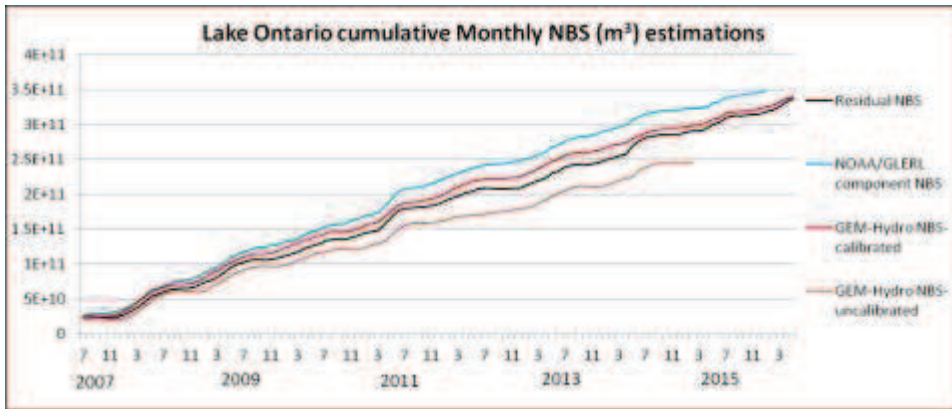
Figure 99: cumulative Lake Ontario NBS (Net Basin Supplies) estimates. Months are shown on the x-axis. See text for further details.
