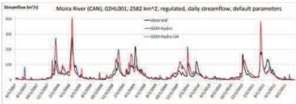
Figure 42: Hydrographs from uncalibrated GEM-Hydro and GEM-Hydro-UH (Moira River - subbasin 11).
