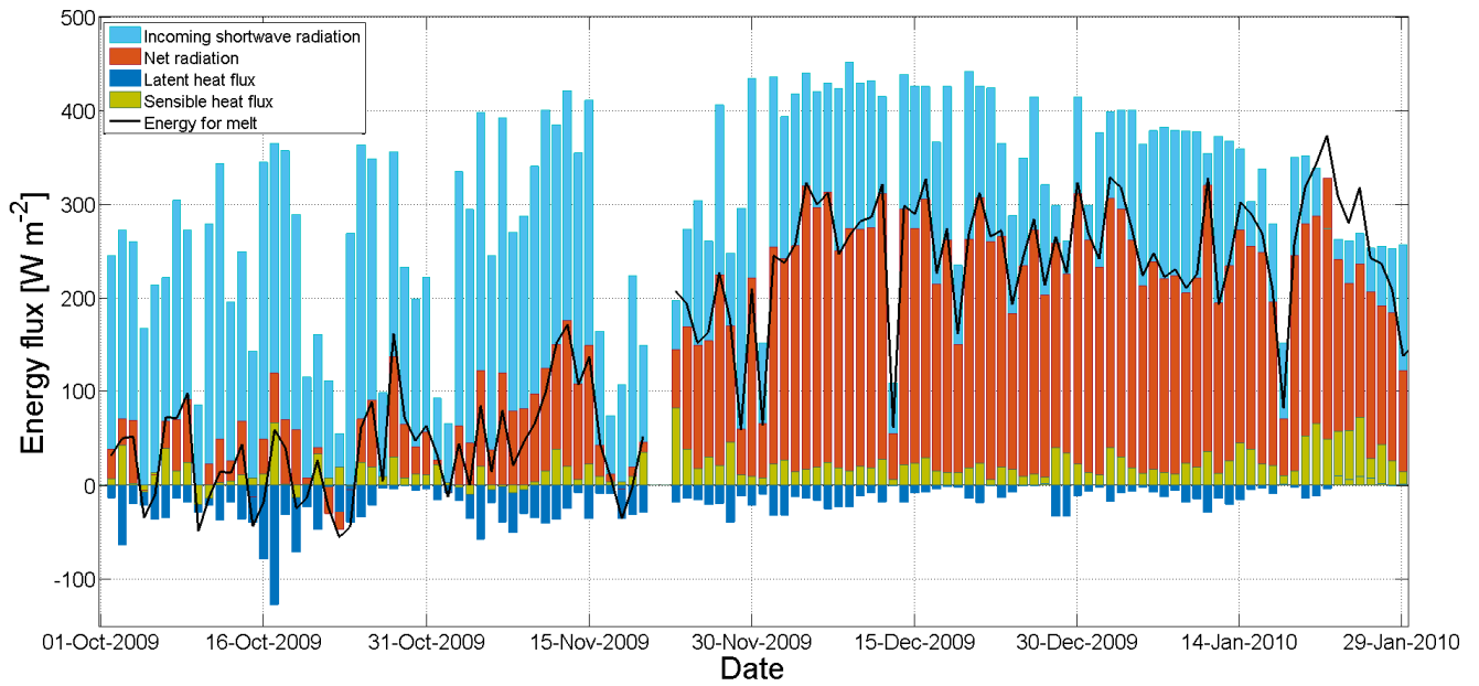
5 Figure 6: Daily mean net radiation, incoming shortwave radiation, latent and sensible heat fluxes and the calculated energy available for melt at AWS1 (2650 m asl). On 21 and 22 November there are no data due to maintenance of AWS1.
