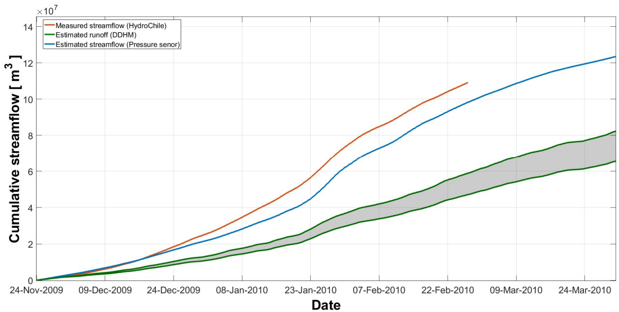
Figure 11: Comparison of cumulative melt calculated with distributed degree-hour model (grey area), and streamflow measurements from the water level sensor data and the HydroChile station.
