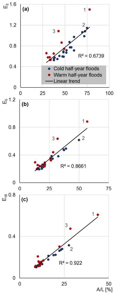
Figure 2: Relationship between the proportion of the affected river length (x-axis) and the flood extremity E (y-axis) according to E_2 (a), E_5 (b) and E_{10} (c). R^2 indicates the value of the coefficient of determination.
