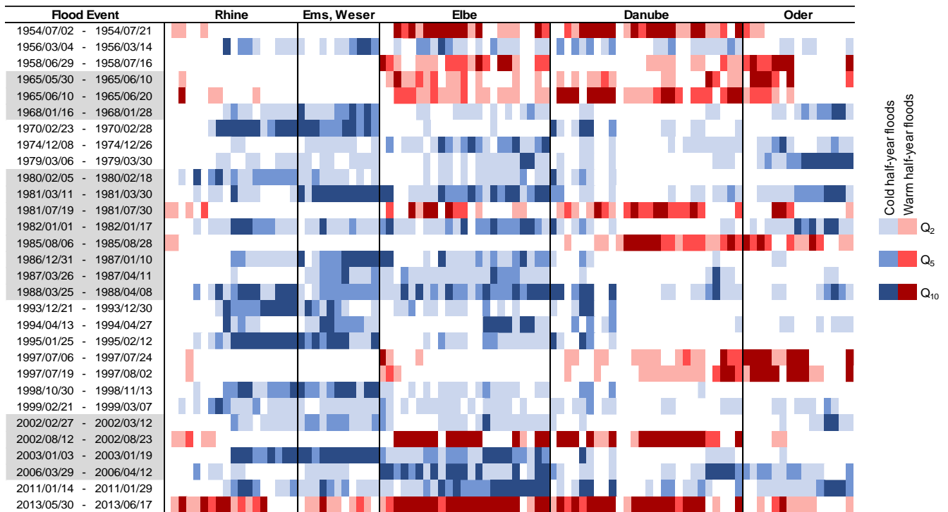
Figure 4: The occurrence of discharges equal to or greater than 2, 5 and 10-year flood at individual stations during each of the 30 maximum floods according to E_2 index. The basins are indicated at the top of the chart; the stations are arranged according to their position downstream.
