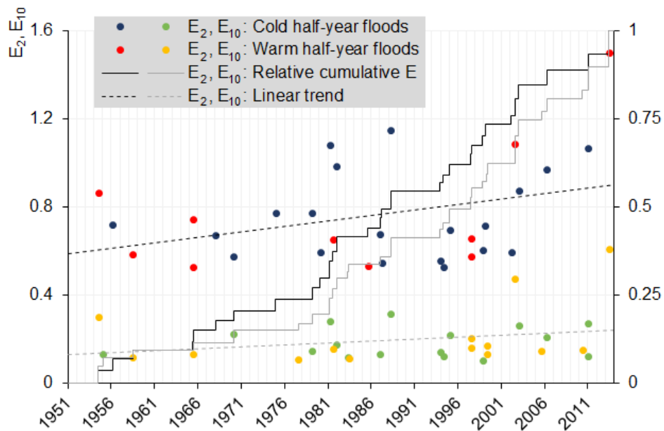
Figure 6: Interannual variability of 30 major floods according to E_2 and E_{10} . The symbols represent the extremity of cold and warm half-year floods with respect to E_2 and E_{10} ; Lines depict linear trends and relative cumulative values of the flood extremity.
