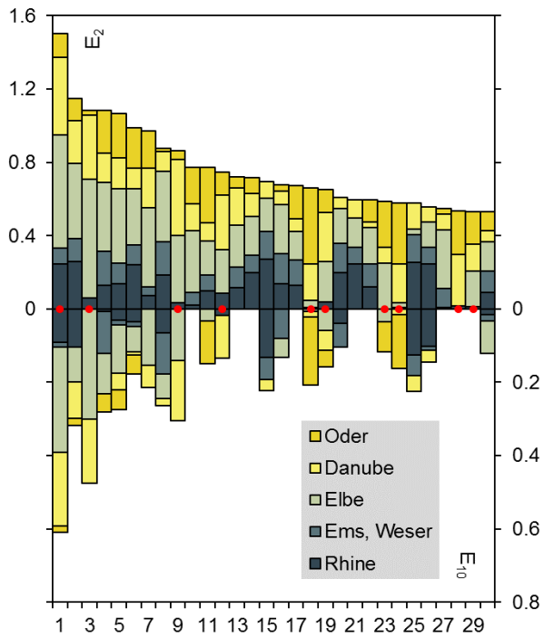
Figure 3: The 30 largest flood events in the study area from 1951 to 2013 according to E_2 and the corresponding events according to E_{10} . Missing bars indicate events which are not included in the set of 30 largest floods compiled by E_{10} . Contributions of individual river basins to the index value are distinguished by color. Red dots indicate warm half-year floods.
