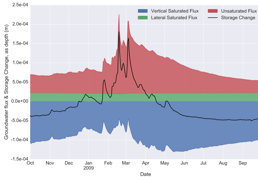
Figure 7: Daily time series of bulk fluxes to/from the simulated Central Valley aquifer system. Positive values indicate a net flow into the aquifer. Negative values indicate net flow out of the aquifer. The balance of inflows and outflows is shown as the change in storage (black line).
