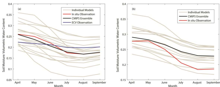
10 Figure 3. Mean monthly soil moisture (2003-2012) during the warm season (April to September) in the 0–10 cm soil layer (a) and in the 0–100 cm soil layer (b). Data are spatially-averaged over CONUS. Figures show the monthly mean soil moisture from the in situ observations (red line), ECV satellite data (blue line), CMIP5 ensemble (black line) and the individual CMIP5 models (grey lines).
