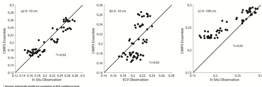
5 Figure 2. Comparison of soil moisture from the CMIP5 ensemble with in situ and satellite-derived (ECV) soil moisture. Each point represents monthly soil moisture data from the warm season (April to September) that has been spatially-averaged over CONUS (2003-2012). (a) CMIP5 ensemble versus in situ observations in the 0–10 cm soil layer. (b) CMIP5 ensemble versus ECV in the 0–10 cm soil layer. (c) CMIP5 ensemble versus in situ observations in the 0–100 cm soil layer during warm season (April to September).
