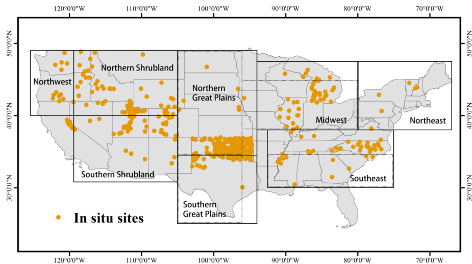
Figure 1: Spatial distribution of in situ soil moisture stations and the boundary of the 8 sub-regions.
