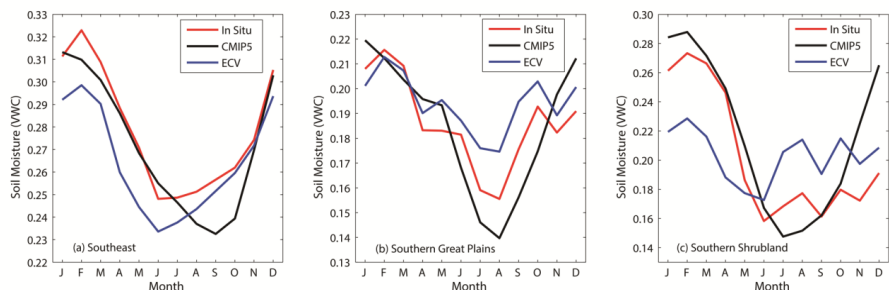
Figure 10. Seasonal variation of mean monthly (2003–2012) soil moisture based on in situ observations (red), CMIP5 ensemble (black) and ECV satellite data (blue) in three regions: (a) Southeast, (b) Southern Great Plains, and (c) Southern Shrubland.
