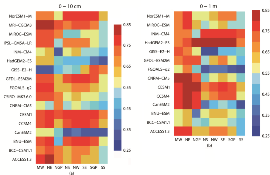
Figure 9. Comparison of CMIP5 models with in situ observations over eight regions based on Taylor's skill scores: (a) 0–10 cm soil moisture, and (b) 0–100 cm soil moisture.
