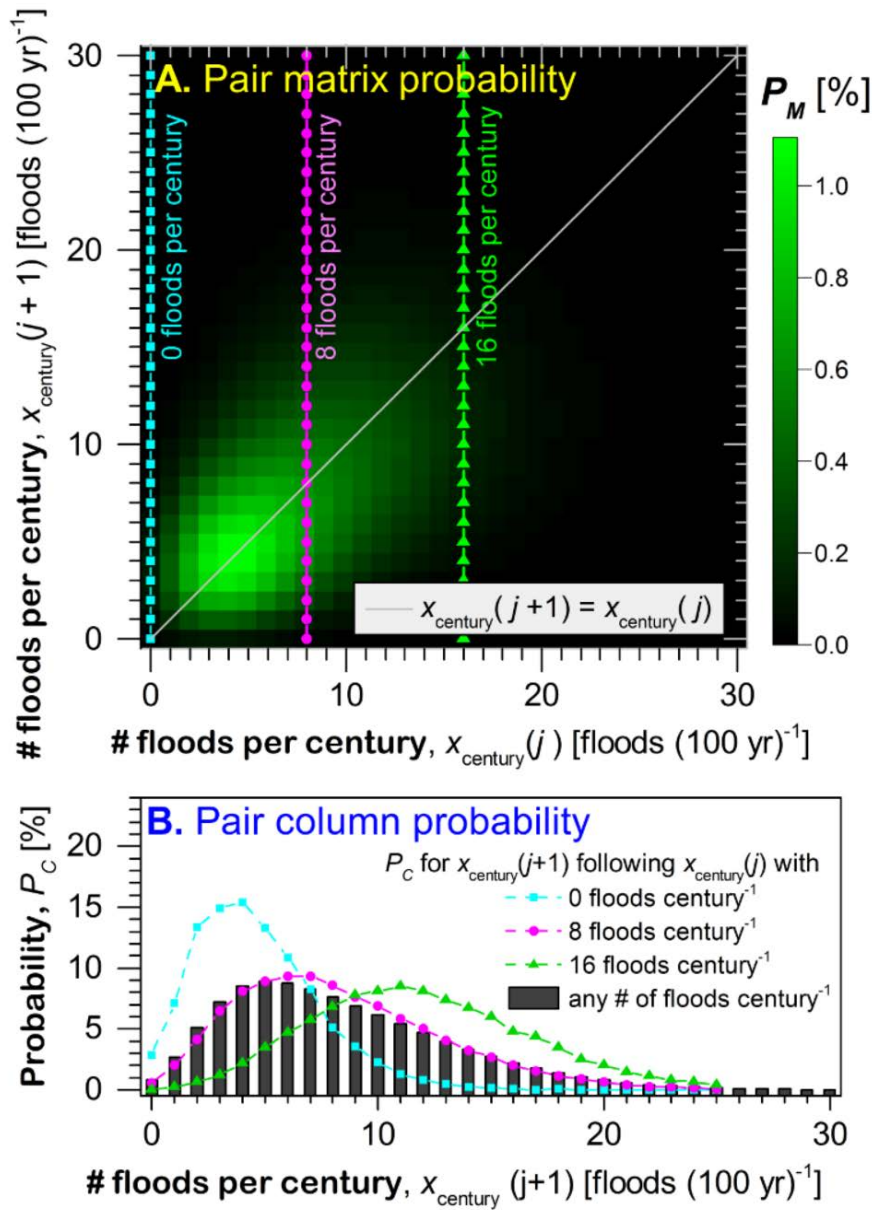
Figure 14: Using the optimized POT FGN+Period model for forecasting the number of floods in one century based on the number of floods in the previous century: Based on the palaeoflood model realizations for one billion (10 9 ) years are shown (A) The 2D probability of the number of floods per century ( x_{\text{century}}(j) ) and the number of floods in the succeeding century ( x_{\text{century}}(j+1) ) (background grid colours, see legend for scale). The solid grey diagonal line represents equality of the number of floods in both centuries ( x_{\text{century}}(j+1) = x_{\text{century}}(j) ). (B) The two-dimensional probability distribution shown in (A) is cut vertically at x_{\text{century}} = 0, 8 and 16 floods century -1 and the corresponding probability densities of floods per centuries after a century with x_{\text{century}} = 0, 8 and 16 floods century -1 are presented as coloured lines (see legend). Also given is the probability density of floods per century of the palaeoflood model.
