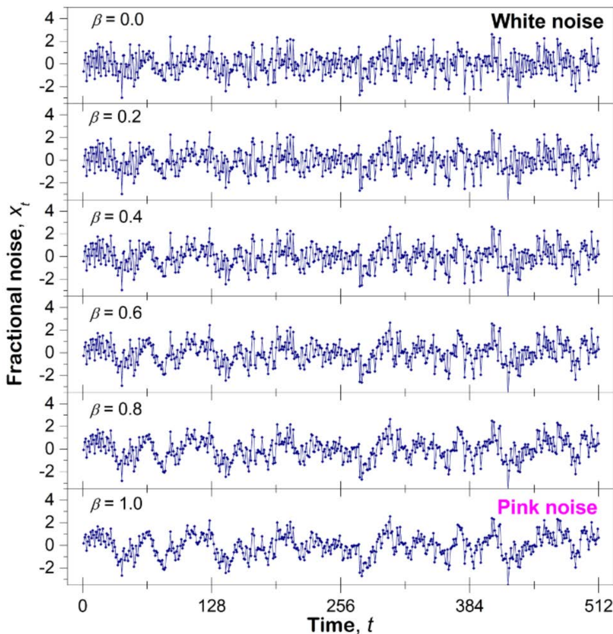
Figure 6: Examples of synthetic fractional Gaussian noises with different modelled strengths of long-range persistence, 0.0 \leq \beta \leq 1.0 . The presented data series, which have 512 elements each, are normalized to have a mean of zero and a standard deviation of one, and were created by Fourier filtering (see Appendices 1 and 2 in Witt and Malamud, 2013 for further details).
