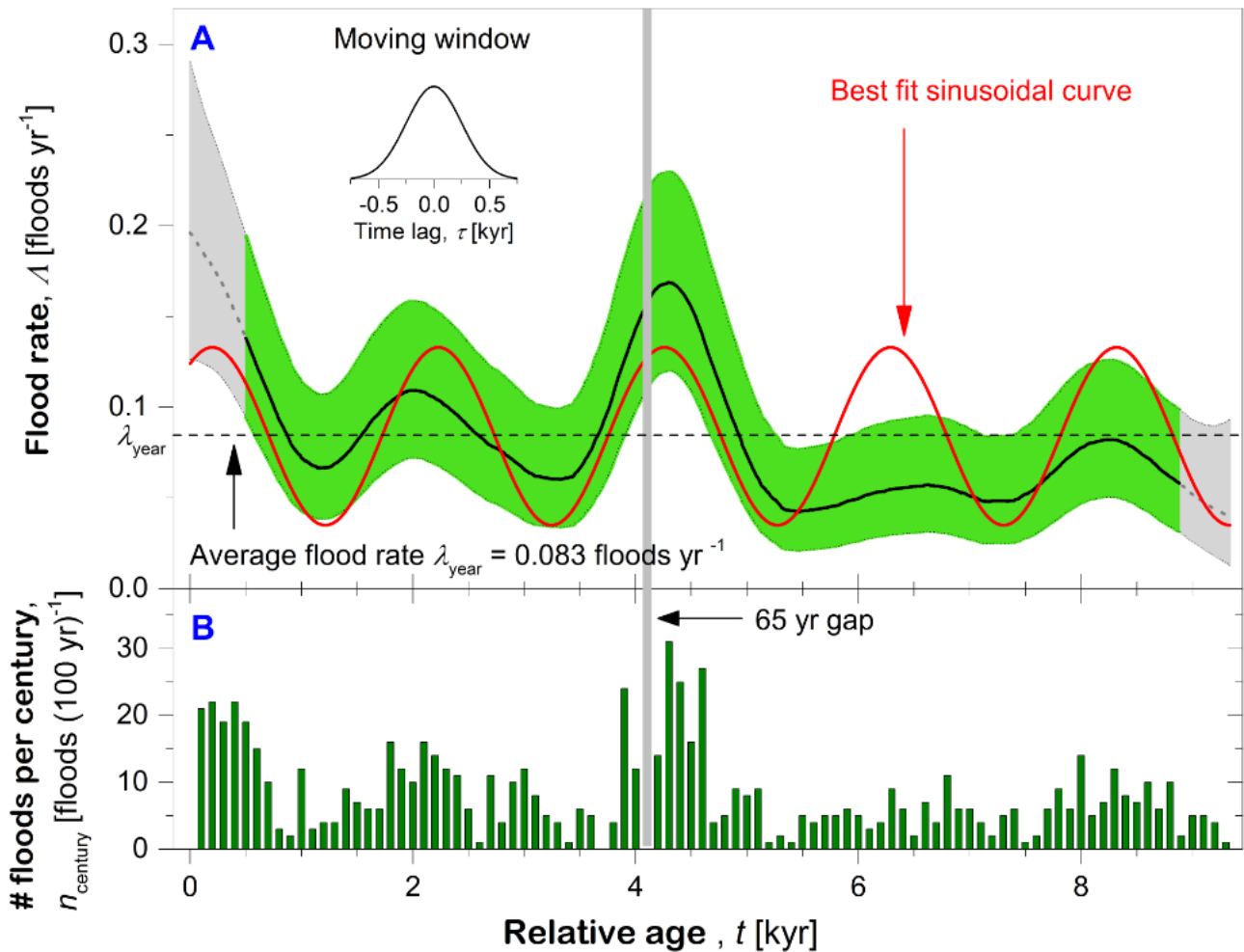
Figure 9: Analysis of flood rate fluctuations: (A) Shown is the time dependent flood rate \Lambda (black line) and its 95% confidence bands (green bands) as a function of the relative age t = 1 to 9336 yr for the palaeoflood data set shown in Fig. 3A which was computed by using a kernel density estimator. The grey colour indicates results that might be affected by boundary effects. The estimator is based on a Gaussian kernel with a width of \pm 3\sigma , where \sigma = 250 yr (Appendix B), shown in the inset figure. Also shown is the mean flood rate (dashed blue line) of \lambda_{\text{year}} = 0.83 \text{ floods yr}^{-1} . (B) For a comparison the number of floods per century n_{\text{century}} (green bars) is presented. The grey vertical bar indicates the gap in the data set.
