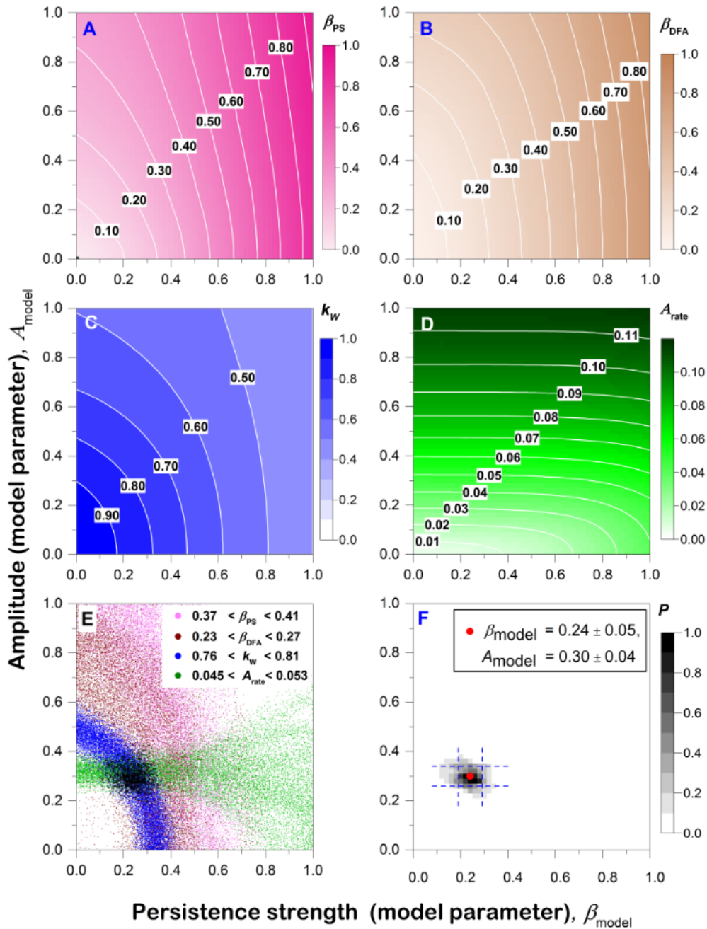
Figure 12: Analysis of model realisations of the POT FGN+Period model with different pairs of parameters for persistence strength and amplitude of the periodic component. Given for all six panels are the two model parameters of the POT FGN+Period : (i) strength of long-range persistence of the underlining fractional Gaussian noise \beta_{\text{model}} = 0.00 to 1.00 (step size 0.02 ) on the x -axis and (ii) the amplitude of the superimposed periodic component (period T = 2030 yr), A_{\text{model}} = 0.00 to 1.00 (step size 0.02 ) on the y -axis. For each of the 51 \times 51 = 2601 pairs of model parameters ( \beta_{\text{model}}, A_{\text{model}} ) 1000 realisations were produced. Each realisation is a synthetic floods per year series which is constructed as described in Sect. 4.1 and illustrated in Fig. 10. In A to D are given the mean of the measured \beta_{\text{PS}}, \beta_{\text{DFA}}, k_{\text{W}} and A_{\text{rate}} (see
