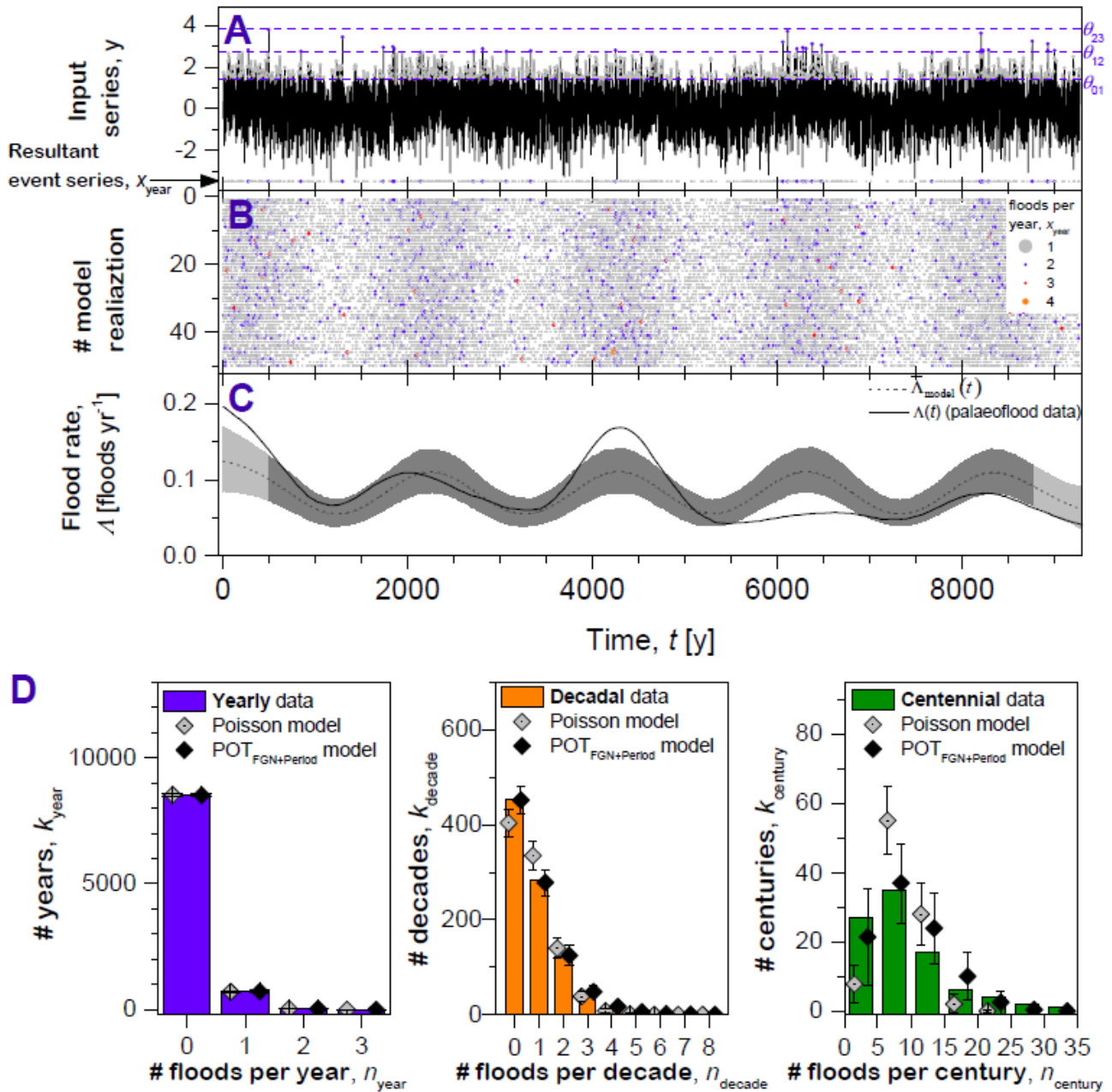
Figure 13: POT FGN+Period model with optimized parameters: (A) Shown (black time series) is a realisation of a fractional Gaussian noise (FGN) with a long-range persistence strength of \beta_{\text{model}} = 0.24 (normalized to a mean = 0.0 and variance = 1.0) that is superimposed with a periodic component (period: T = 2030 yr, amplitude A = 0.30 ). This synthetic time series is given a time resolution of \Delta t = 1 yr and the length N_{\text{year}} = 9270 yr. Peaks over thresholds (POT) are considered (as in Fig. 10) for five thresholds (three shown here) \theta_{01} , \theta_{12} , etc. where input (FGN+period) values < \theta_{01} translate to x_{\text{year}} = 0 flood \text{yr}^{-1} , input values between \theta_{01} and \theta_{12} result in x_{\text{year}} = 1 flood \text{yr}^{-1} , etc. The resultant model series of the number of floods per year (grey and blue circles) for 9270 years is constructed to have a Poissonian one-point distribution and is shown at the bottom of the panel A. (B) Shown are 50 more model realisations of the POT FGN+Period model as number of floods per year (see legend for the colour code), with maximum x_{\text{year}} = 4 floods \text{yr}^{-1} . (C) Time dependent flood rate \lambda(t) given as a function of time t
