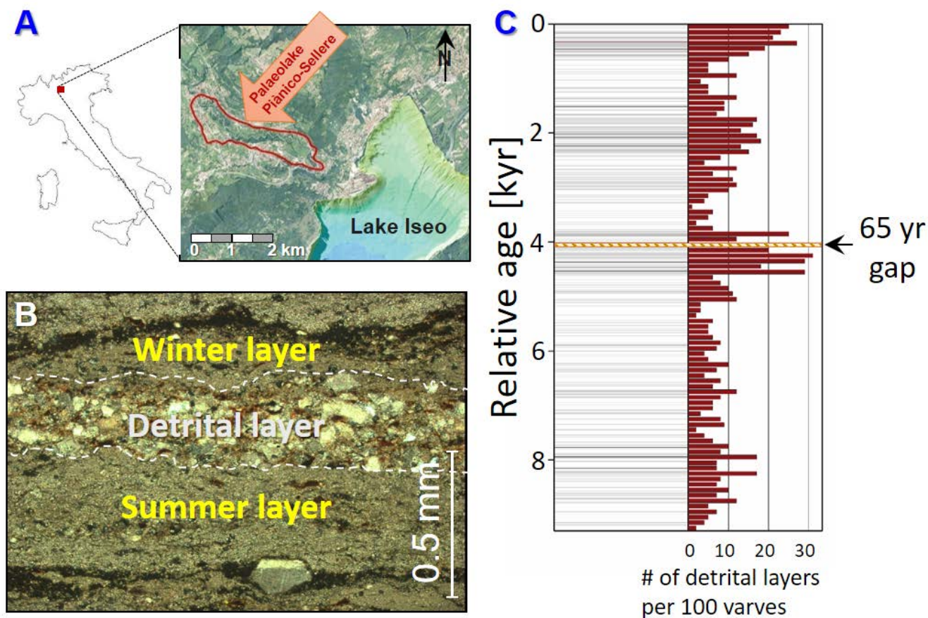
Figure 2: Site, sediment outcrop and data. (A) Location of the Palaeolake Piànico-Sèllere, Italy. (B) Detail of the 9.5 m sediment outcrop containing a winter and a summer layer with, shown here, a detrital layer in-between, that is interpreted to be a flood event. (C) Graphical representation of the sediment outcrop with the grey horizontal lines indicating detrital layers and the striped bar showing a 65 yr gap (see Fig. 3, for more detailed time series). The relative age represents years before the top of the stratigraphic section examined, with actual age estimated to be anywhere from 390 to 780 ka (see text).
