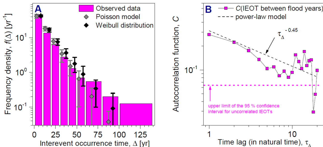
Figure 5: Frequency-size and autocorrelation analysis of the interevent occurrence times (IEOTs) and comparison to the Poisson model. (A) Frequency density of the IEOTs between the flood years given as a function of IEOTs in yr (pink vertical bars, semi-logarithmic scale), the corresponding best-fit Poisson model (grey diamonds) which was considered in Fig. 3B and the best-fit Weibull distribution (black diamonds), both with 95% confidence intervals. (B) Autocorrelation function of the IEOTs between flood years (those years with n \geq 1 flood). Also given is the best fitting power-law model (dashed black line) and the upper limit of the 95% significance for the autocorrelation function of a non-correlated time series with the same one-point probability distribution (horizontal dotted line, pink).
