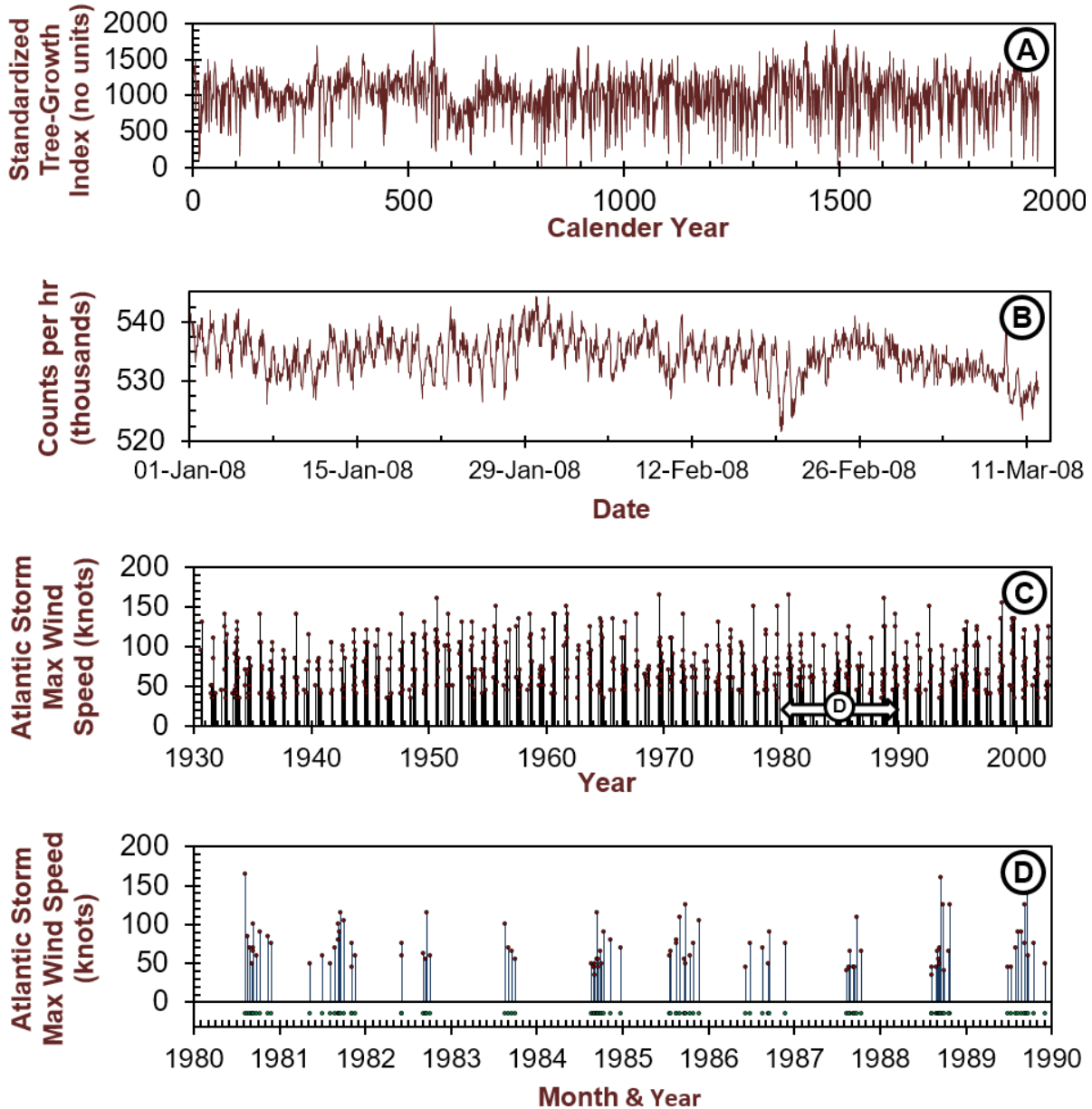
Figure 1. Example of correlations, clustering and cyclicity (figure after Witt et al., 2010). (A) Tree ring standardized growth index for Bristlecone pine, White Mountain, California, USA, for the years AD 0–1962 (Ferguson et al., 1994). (B) Cosmic ray neutron counts per hour, Beijing, China, 1 January to 11 March 2008 (NGDC, 2008). In (A) and (B) successive values in each both series are positively correlated with one another, and are examples of persistent time series. (C) The maximum wind speed in knots is plotted as a function of date, for 730 Atlantic Basin named and unnamed severe storms and hurricanes, 1930–2003 (NOAA, 2003); only storms with maximum wind speed \geq 35 knot are included. (D) The same data as in C, but focussing in on 1980–1990, with minor tick marks representing months. The value of maximum wind speed for each storm event is projected to the x -axis (wind speed = 0 knot). Below this is shown (green dots) all events over the threshold of 35 knot along one line, an example of a data series that is strongly clustered in time. Clustering is due to (i) seasonal effects (cyclicity) and (ii) fewer Atlantic Basin events occurring (on average) during El Niño years (e.g. April 1986–March 1988) and more events occurring (on average) during La Niña years (e.g. April 1988–June 1989).
