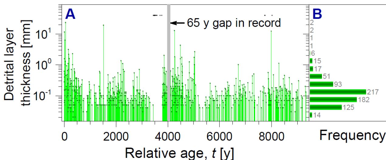
Figure A1. Detrital layer thickness: (A) Thickness and temporal location of the detrital layers in the varved sediment. 771 layers are located within the 9271 varves. The x-axis represents relative age, with 0 yr representing the most recent varve and increasing values indicating further back in time. The grey bar represents a sediment gap of 65 yr. The varve thickness (green vertical bars), shown on a logarithmic scale, ranges from 0.002 to 23 mm, some layers are just reported and not measured (black dots). The detrital layers are unequally distributed over time. A histogram of the layer thickness is given in (B)
