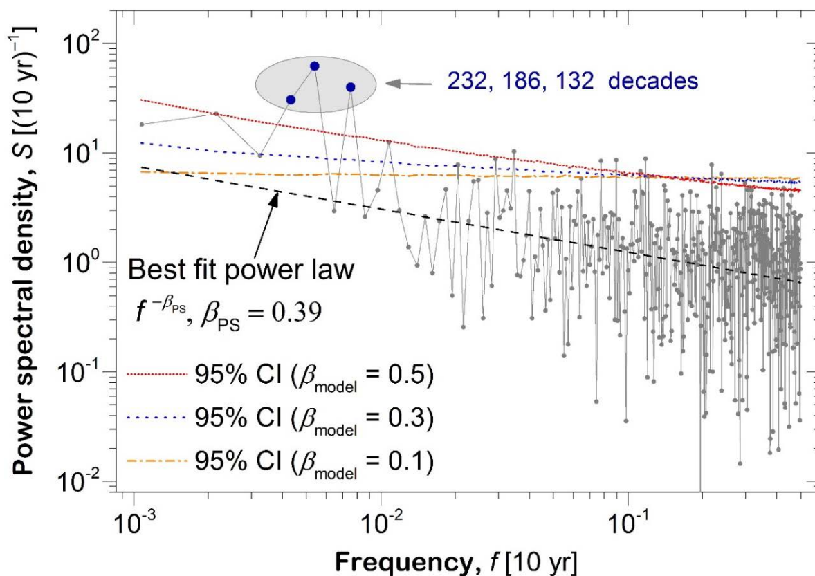
5 Figure 8: Power spectral analysis: The power spectral density (periodogram) is presented as a function of the frequency (measured per decade) for the number of floods per decade. Also given is the best fitting power-law function and the corresponding power-law exponent. Additionally, presented are the 95th percentiles of the power spectra created for synthetic data based on peaks over thresholds of fractional noises (see Sect. 4.1) for different strength of persistence (see legend, and description in text). Highlighted are the three values of the power spectral density that exceed all of these 95% percentiles, the corresponding cycle lengths are given.
