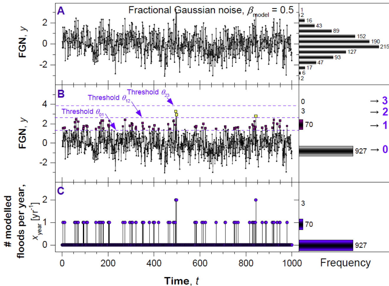
Figure 10: Schematic of the \text{POT}_{\text{FGN}+\text{Period}} model: (A) Shown is a fractional Gaussian noise with a persistence strength of \beta_{\text{model}} = 0.5 . The time resolution is \Delta t = 1 y. (B) Three thresholds are set (dashed horizontal lines). All noise values that are below the threshold \theta_{01} are considered as years with zero floods, all noise values between the thresholds \theta_{01} and \theta_{12} [ \theta_{12} and \theta_{23} ] are considered as years with one [two] floods, and all noise values that exceed the threshold \theta_{23} are considered years with 3 floods. The thresholds \theta_{01} , \theta_{12} and \theta_{23} are chosen such that the resultant one-point probability distribution is the same as our flood series (C) Time series of the modelled number of floods per year (blue circles) for 1000 years. For parts (A), (B) and (C) are also shown the histogram of the number of values at a given size.
