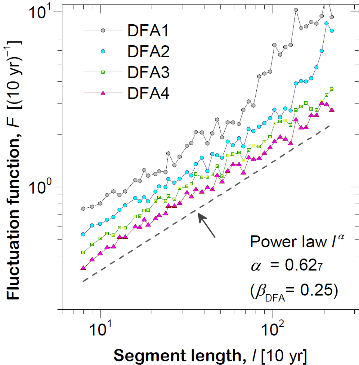
Figure 7. Detrended Fluctuation Analysis (DFA) of the 9271 yr Piànico-Sèllere, Italy palaeoflood record: The fluctuation function F for the number of floods per decade shown as a function of the segment length l and for different orders of the detrending (see legend) on a double logarithmic scale. Segments containing parts of or the entire gap were excluded. Also shown are best fitting power-law function for DFA3 and the corresponding power-law exponent \alpha and its corresponding value of \beta_{\text{DFA}} = 2\alpha - 1 .
