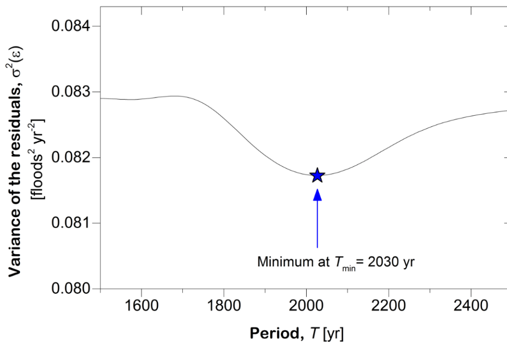
Figure C1. Shown is the variance of the residuals ( \sigma^2(\epsilon) ) for fitting a sinusoidal function to the floods per year series n_{\text{year}} as a function of the period T of this periodic function. The function for the variance of the residuals has a minimum at T_{\text{min}} = 2030 yr (shown as a star in the figure).
