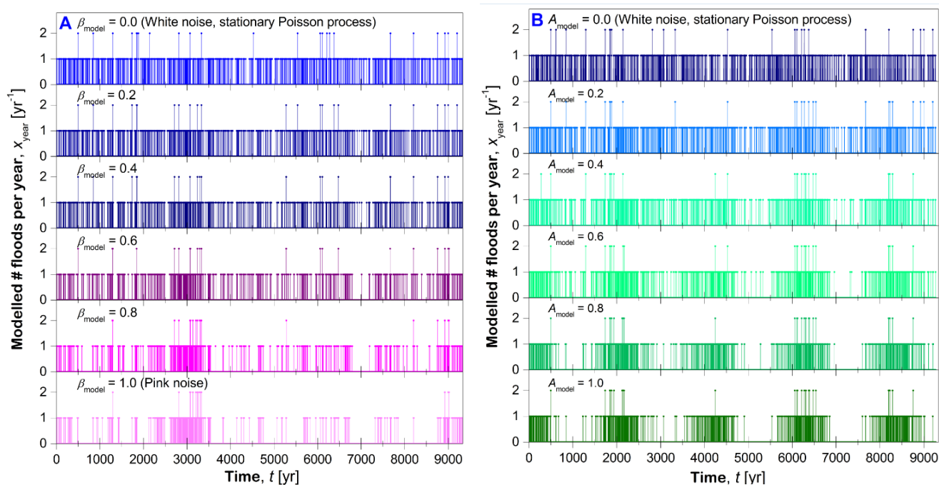
Figure 11: POT FGN+Period model realisations: Shown are (A) long-range persistent flood time series that are modelled with the proposed POT FGN+Period model (see Fig. 10) as peaks over thresholds (POT) of a fractional Gaussian noise (illustrated in Fig. 6) with different persistence strengths \beta_{\text{model}} = 0.0, 0.2, 0.4, 0.6, 1.0 , and (B) flood time series x_{\text{year}} with a long-term periodic cyclicity which are modelled as peaks over thresholds (POT) of a Gaussian white noise ( \beta_{\text{model}} = 0.0 ) superimposed with a sine wave ( T = 2000 yr) with different sine wave amplitudes A_{\text{model}} = 0.0, 0.2, 0.4, 0.6, 1.0 .
