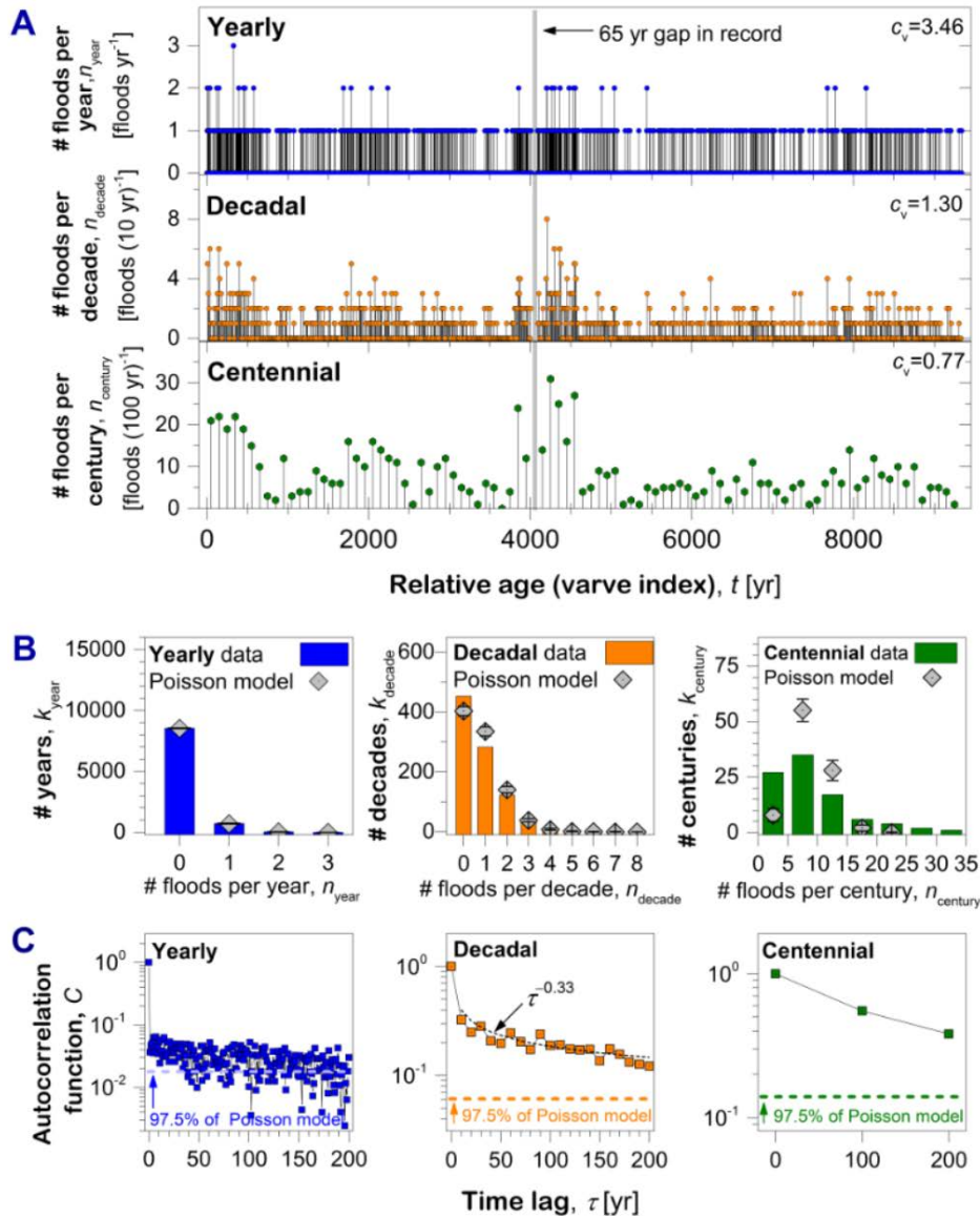
Figure 3: Temporal succession, histograms and autocorrelation of the detrital layers of the 9336 yr Piànico-Sèllere, Italy palaeoflood record. (A) The number of observed detrital (flood) layers per year (blue dots, 0 \leq n_{\text{year}} \leq 3 floods yr -1 ), decade (orange dots, 0 \leq n_{\text{decade}} \leq 8 floods decade -1 ) and century (green dots, 0 \leq n_{\text{century}} \leq 31 floods century -1 ) are presented over the 9336 yr of record examined. The x -axis represents relative age, with 0 yr the most recent varve and increasing values indicating further back in time. The grey bar represents a sediment gap of 65 yr (leaving 9271 yr of record examined over the 9336 yr). In addition, for each time resolution is given (upper right) the coefficient of variation c_v = \sigma/\mu , where \sigma is the standard deviation and \mu is the mean of the given time series. (B) Histogram of the number floods per year (blue bars), decade (orange bars) and century (green bars), with each compared to the Poisson model with respective rate parameters \lambda_{\text{year}} = 0.083 floods yr -1 , \lambda_{\text{decade}} = 0.83 floods decade -1 , \lambda_{\text{century}} = 8.3 floods century -1 . Diamonds represent the mean Poisson model value over 100 realisations, and the error bars the standard deviation of the realisations. (C) Autocorrelation function (ACF) of the number of floods per year (blue squares), decade (orange squares) and century (green squares). Also shown for the ACF of the number of floods per decade, is the best-fitting power-law model to the ACF (black dotted line). Also shown are the 97.5 percentile, i.e., the upper bound of the 95% confidence interval of the ACF (for lags \tau > 0 ) of an uncorrelated signal with the same one-point probability distribution.
