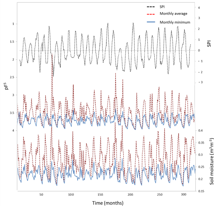
Figure 1.1: Time series of the SPI, the simulated monthly minimum soil water pressure and monthly average soil water pressure, and the monthly minimum soil moisture and monthly average soil moisture in 5 cm depth in Cairns. Note: average and minimum soil moistures are also included to this figure aligned with the reviewer #3 comments.
