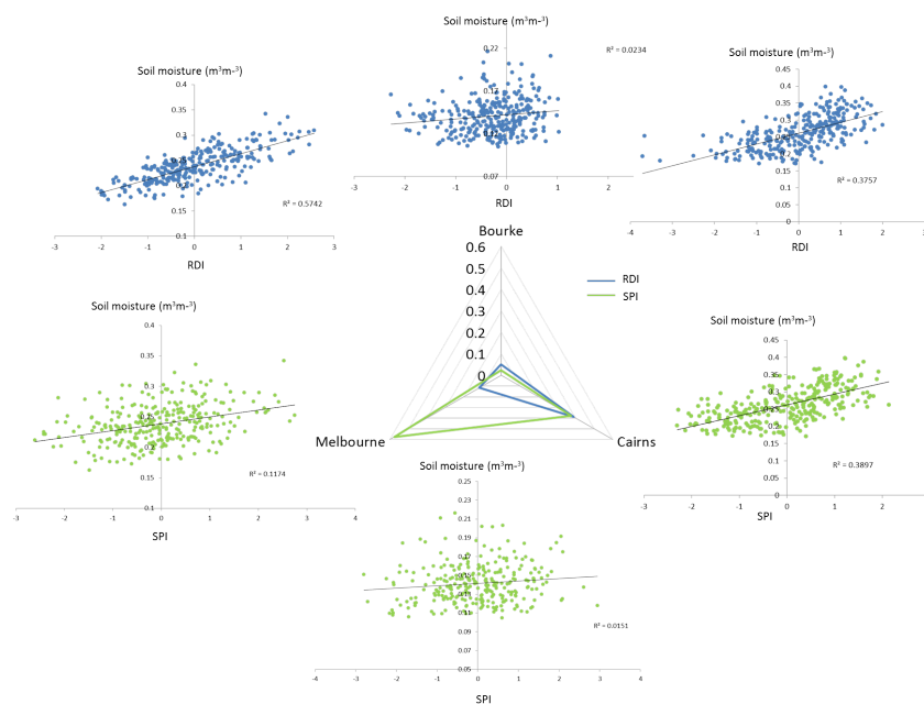
Fig. 1. Correlations between simulated monthly minimum soil moisture in 5 cm soil depth vs SPI and RDI. The scatter plots represent the correlation for each location.
