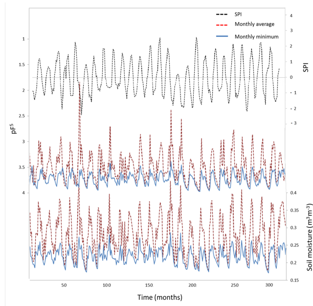
Figure 2.1: Time series of the SPI, the simulated monthly minimum soil water pressure and monthly average soil water pressure, and the monthly minimum soil moisture and monthly average soil moisture in 5 cm depth in Cairns. Note: average and minimum soil moistures are also included to this figure aligned with the reviewer #3 comments.
