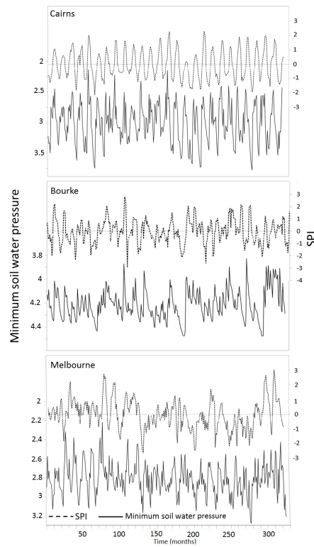
Fig. 1. Simulated monthly minimum soil water pressure in 5 cm depth and SPI for Cairns, Bourke and Melbourne.
