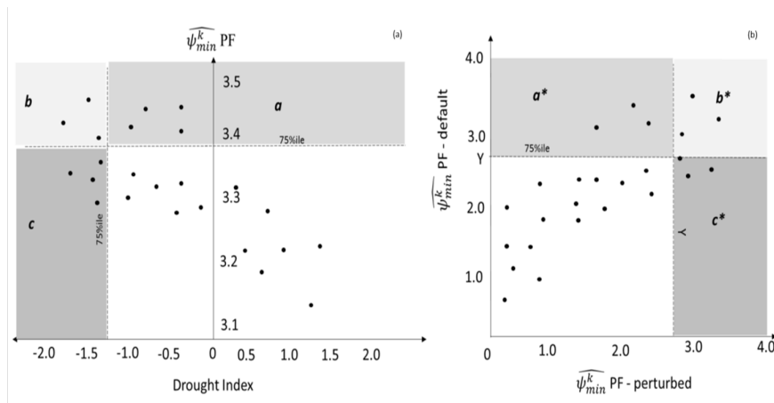
Figure 2: (a) Conceptual schematic of periods of the simulated soil water pressures in relation to the calculated drought index. The threshold values (dashed lines) divide the schematic into four segments, upon which the failure rate (FR) and false alarm rate (FAR) are based on (Section 2, step 3). The segments represent the simulated low soil water pressure events that are not (a) or are (b) detected by the drought index, and the drought events detected by the drought index that do not (c) or do (not labelled) correspond to periods of low simulated soil water pressure. (b): Conceptual schematic of periods of the perturbed Hydrus parameters in relation to the default Hydrus parameters. The threshold values (dashed lines) for default is 75 th percentile and the threshold value for perturbed is the soil water pressure value of 75 th percentile of default ( y ).
