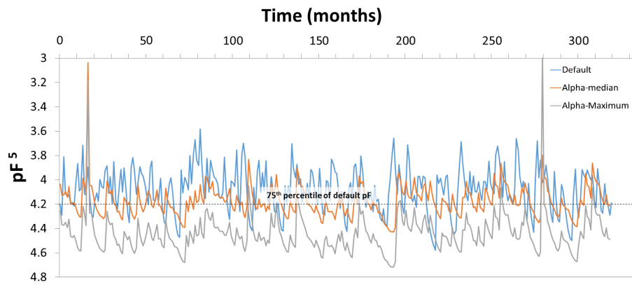
Fig. 3. Default and perturbed (median and maximums for parameter alpha) monthly minimum soil water pressure in 5 cm depth for Bourke.
