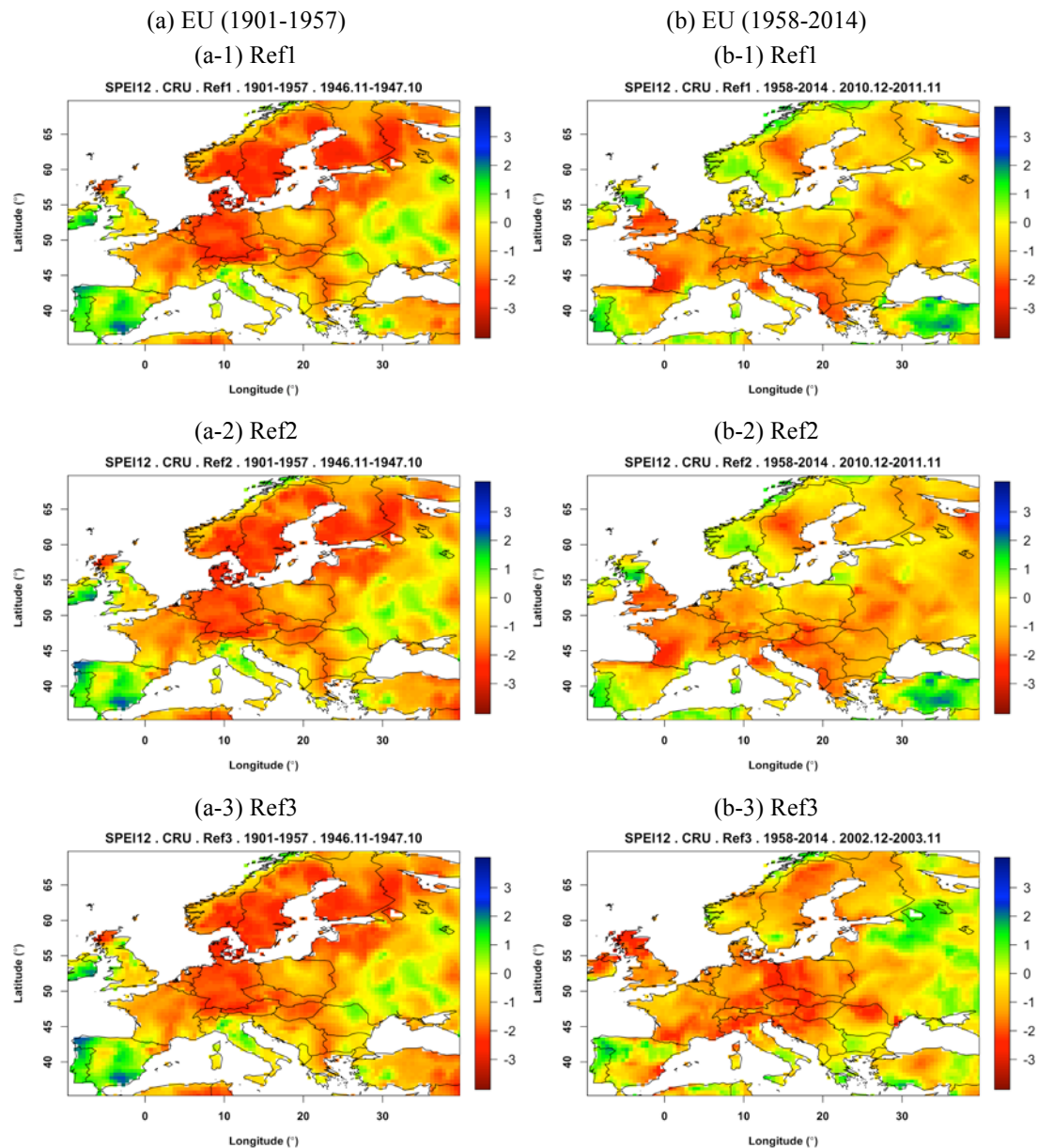
Figure R1. Spatial distribution of SPEI-12 for the case listed in Table R1 (i.e., severest regional averaged SPEI-12 with the 1 month moving window for (a) 1901-1957 and (b) 1958-2014 in EU with CRU).
