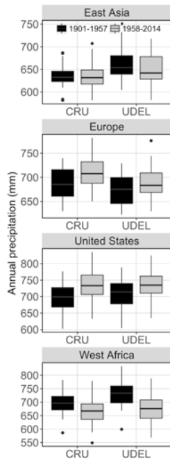
Figure 3. Temporal variations in annual precipitation (mm), PET (mm) and surplus or deficit (D) (mm) based on two datasets (CRU and UDEL) and periods (1901-1957 and 1958-2014). In the box plots, the center line represents the median value; the top and bottom of each box represent the 25 th and 75 th percentile of the data, respectively; and the dots represent outliers.
