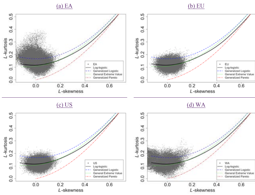
L-moment ratio diagrams for D in Eq. (1) with a 12-month timescale based on CRU for each region for 1901-2014 and 1901-1957.
