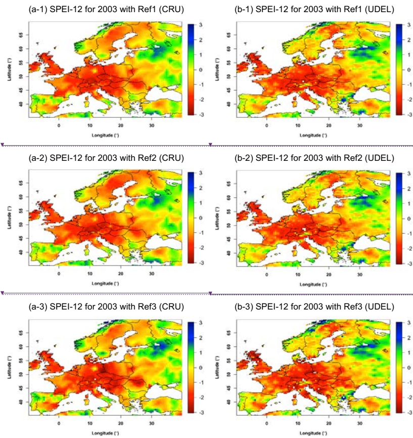
Figure J4. Spatial distribution of SPEI-12 for three different reference periods (Ref1, Ref2 and Ref3 in Table 2) based on the (a) CRU and (b) UDEL datasets in Europe in 2003 as an example.
