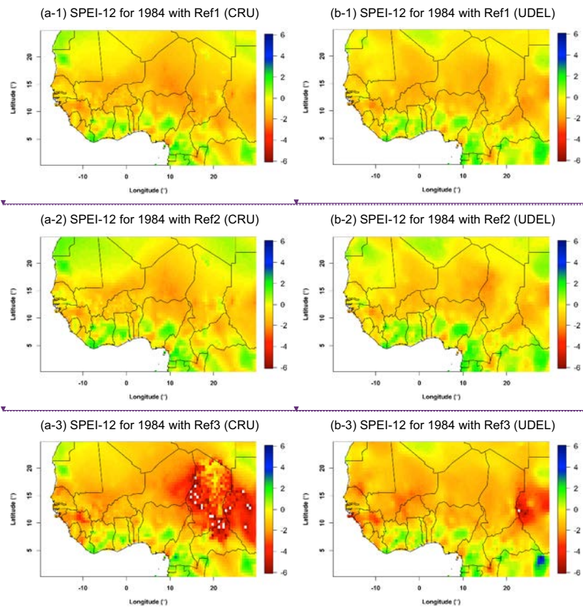
Figure J6. Spatial distribution of SPEI-12 for three different reference periods (Ref1, Ref2 and Ref3 in Table 2) based on the (a) CRU and (b) UDEL datasets in West Africa in 1984 as an example.
