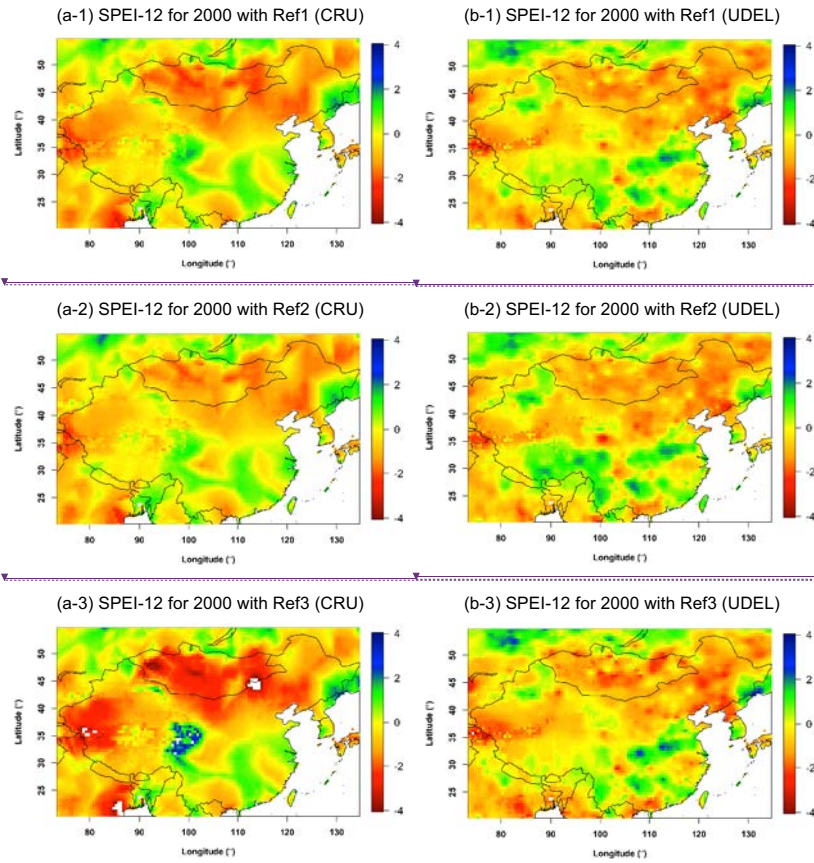
Figure J3. Spatial distribution of SPEI-12 for three different reference periods (Ref1, Ref2 and Ref3 in Table 2) based on the (a) CRU and (b) UDEL datasets in East Asia in 2000 as an example.
