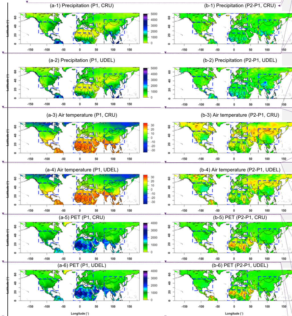
Figure 2. Annual precipitation (mm), annual average temperature (°C) and annual potential evapotranspiration (PET) (mm) based on the datasets of the Climate Research Unit (CRU) and the University of Delaware (UDEL) for the period 1901-1957 (P1) and the difference between P1 and 1958-2014 (P2) (i.e., P2-P1).
