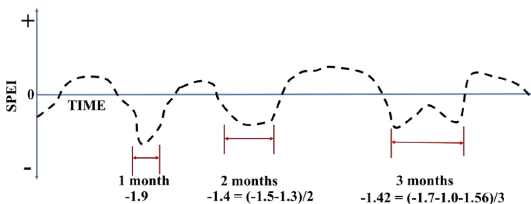
Figure R2. Conceptual explanation how to estimate the severest SPEI-12 for different window sizes.
