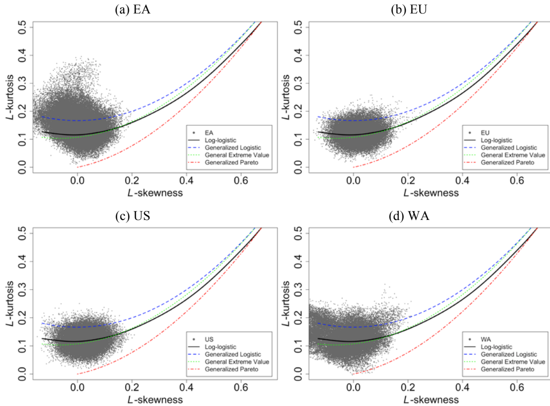
Figure 5. L-moment ratio diagrams for D in Eq. (1) with a 12-month timescale based on CRU for each region for 1901-2014, 1901-1957.
