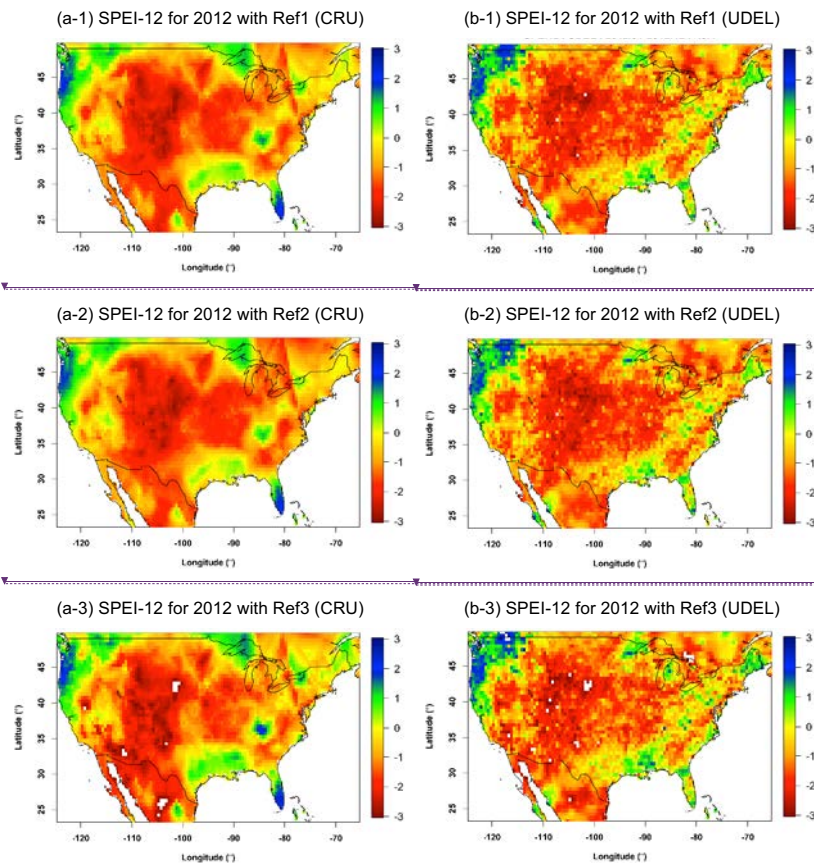
Figure J5. Spatial distribution of SPEI-12 for three different reference periods (Ref1, Ref2 and Ref3 in Table 2) based on the (a) CRU and (b) UDEL datasets in the United States in 2012 as an example.
