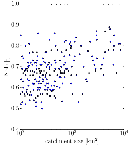
Figure 3: Relation of model performance and catchment area for the 222 basins.
