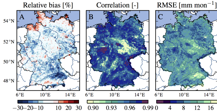
Figure 2: Comparison of monthly estimates of evapotranspiration from mHM and MODIS in the period 2001-2010. The ensemble is represented by the ensemble mean of 100 evapotranspiration estimates. The comparison is based on three statistical assessments: A) relative bias, B) Pearson correlation coefficient, and C) root mean squared error (RMSE). The respective units are given in brackets.
