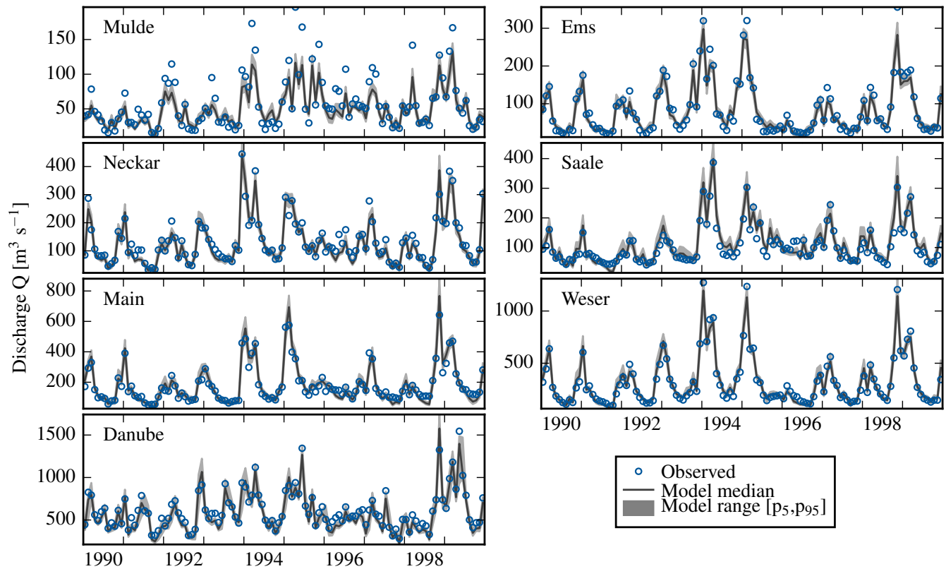
Figure 3. Observed and modeled monthly discharge streamflow for the seven catchment basins, which were used for parameter inference. The figure shows one decade (1990-1999) of the evaluation period. The solid dark gray line depicts the median model results and the light gray band depicts the range between the 5 th and 95 th percentile of the 100 ensemble simulations.
