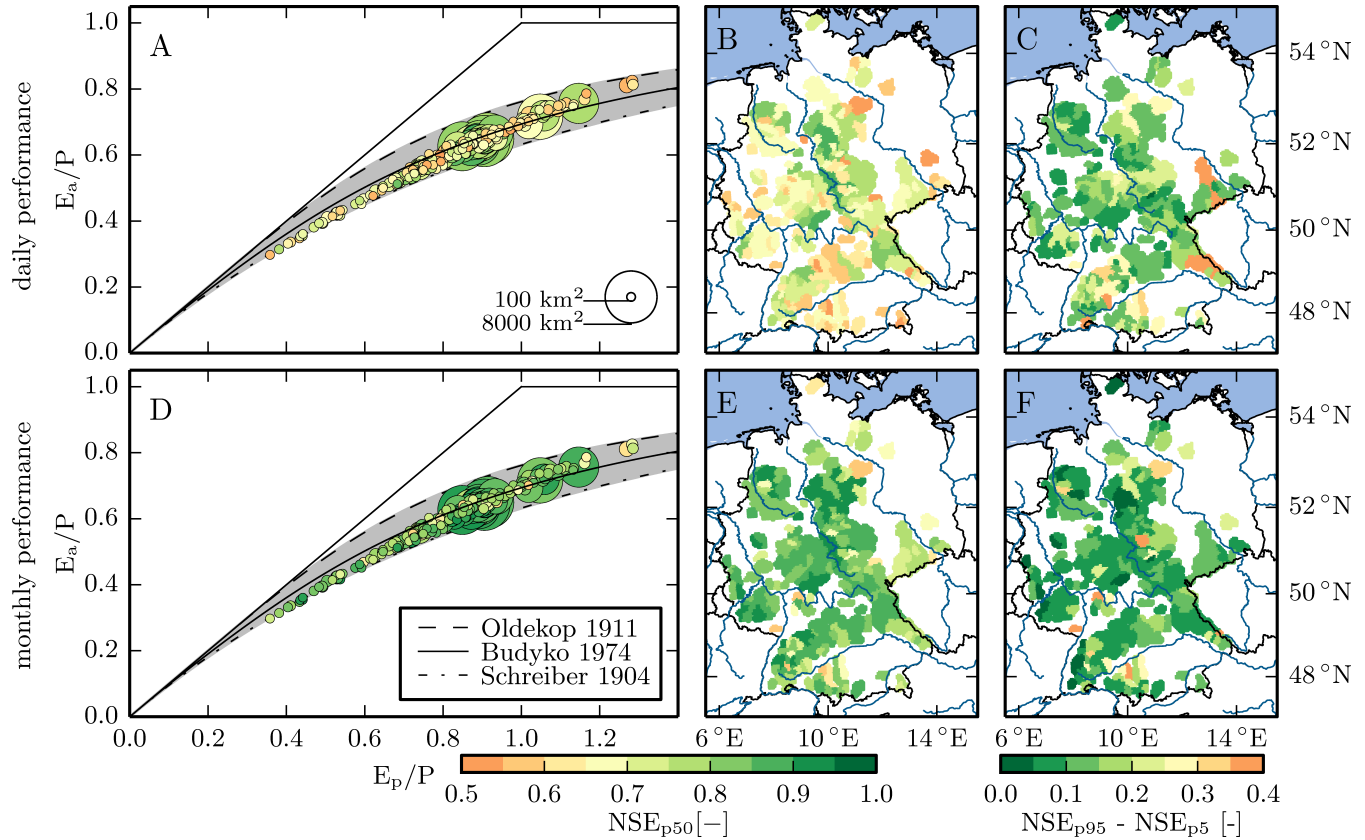
Figure 4. Budyko plot and performance maps for 100 ensemble parameter sets at 222 catchments-basins spread over Germany. The upper row depicts evaluations based on daily values (panels A, B, and C), whereas the lower row depicts monthly discharge-streamflow evaluations (panels D, E, and F). In the first column the catchments-basins are presented as Budyko plots (panels A and D), which are color-coded based on the ensemble median NSE for daily (panel A) and monthly (panel D) discharge-streamflow values. The gray band envelops different estimations of the Budyko curve (Schreiber, 1904; Ol’dekop, 1911; Budyko, 1974). A separation to energy- ( E_p/P < 1 ) and water-limited basins ( E_p/P > 1 ) can be made based on the x-axis. The center column depicts the location of the 222 catchments-basins shown in the Budyko plots using the same color code (panels B and E). The right column shows the range of the 5 th and 95 th ensemble percentiles for the NSE on daily (panel C) and monthly (panel F) basis. Panels A, B, D, and E share the left color bar, and panels C and F share the right color bar. The simulation period is adopted according to the available discharge-streamflow observations but is at least 10 years (average=42 years).
