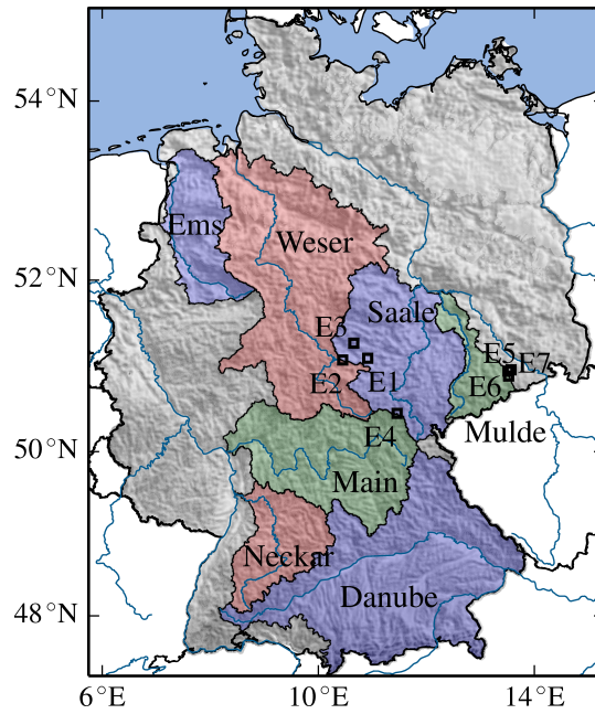
Figure 1. Study area showing the seven catchments-basins used for estimation of common-the ensemble parameter sets for Germany. The different colors are making the basins better distinguishable. The points E1-E7 denote eddy covariance stations which are used for the evaluation of evapotranspiration and soil moisture.
