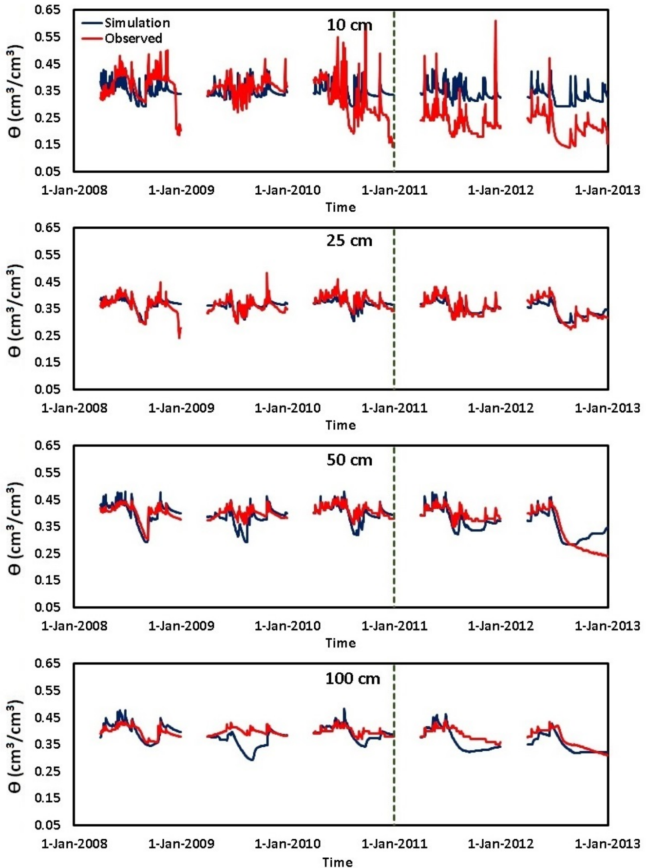
Figure S2. Daily observed and simulated SWC ( \theta ) during the calibration (2008–2010) and validation (2011–2012) periods at TP 3 location.
