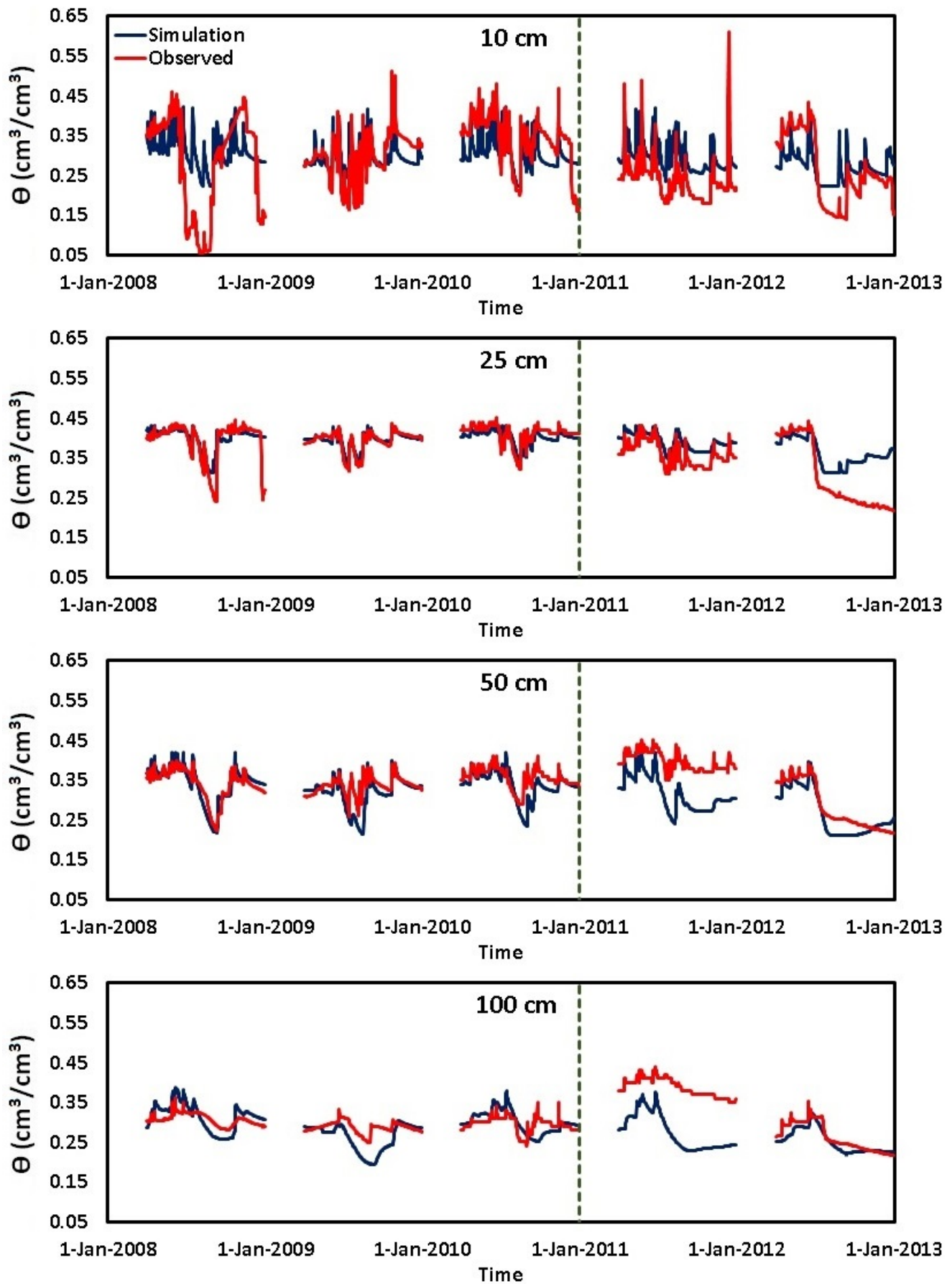
Figure S1. Daily observed and simulated SWC ( \theta ) during the calibration (2008–2010) and validation (2011–2012) periods at TP 2 location.
