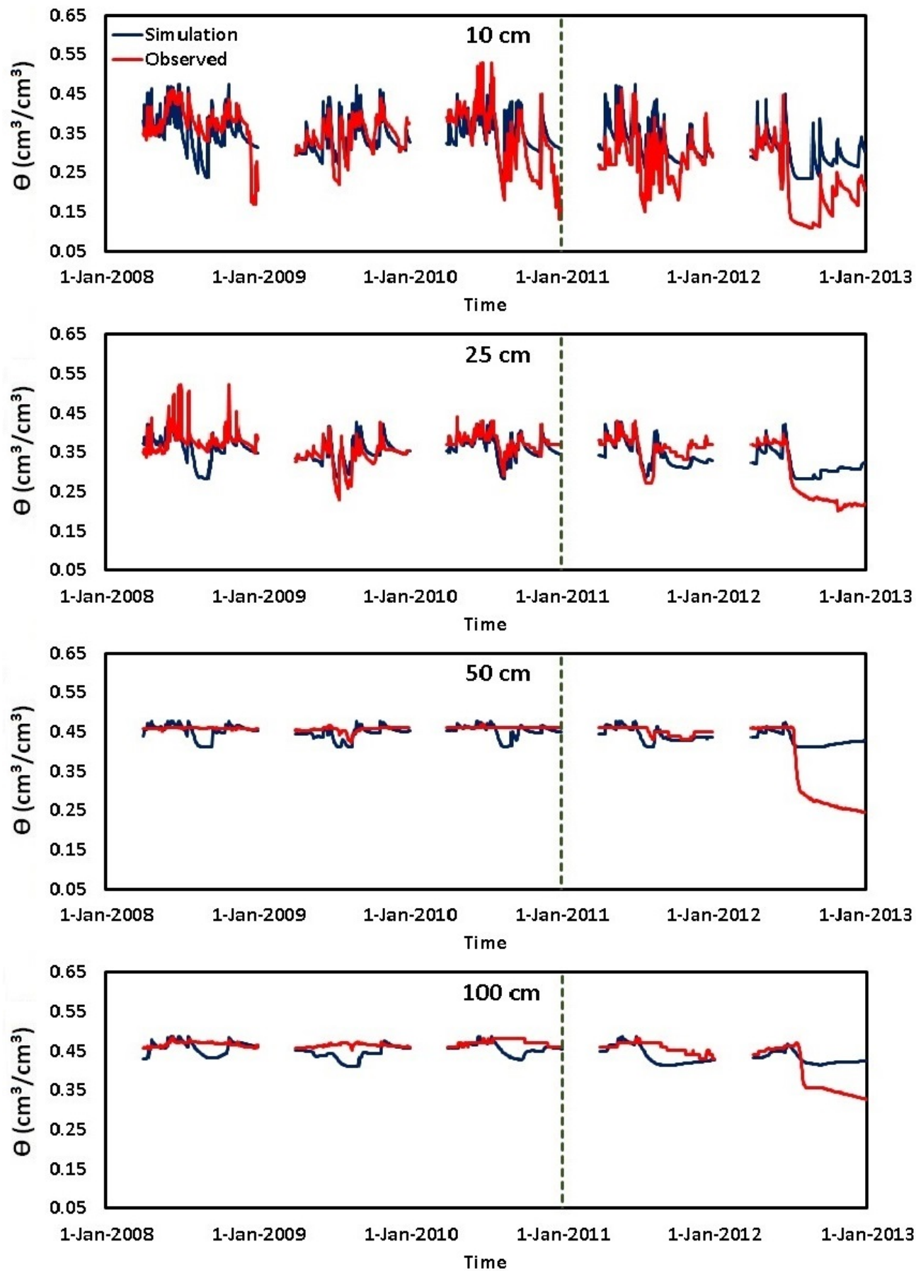
Figure S3. Daily observed and simulated SWC ( \theta ) during the calibration (2008–2010) and validation (2011–2012) periods at TP 4 location.
