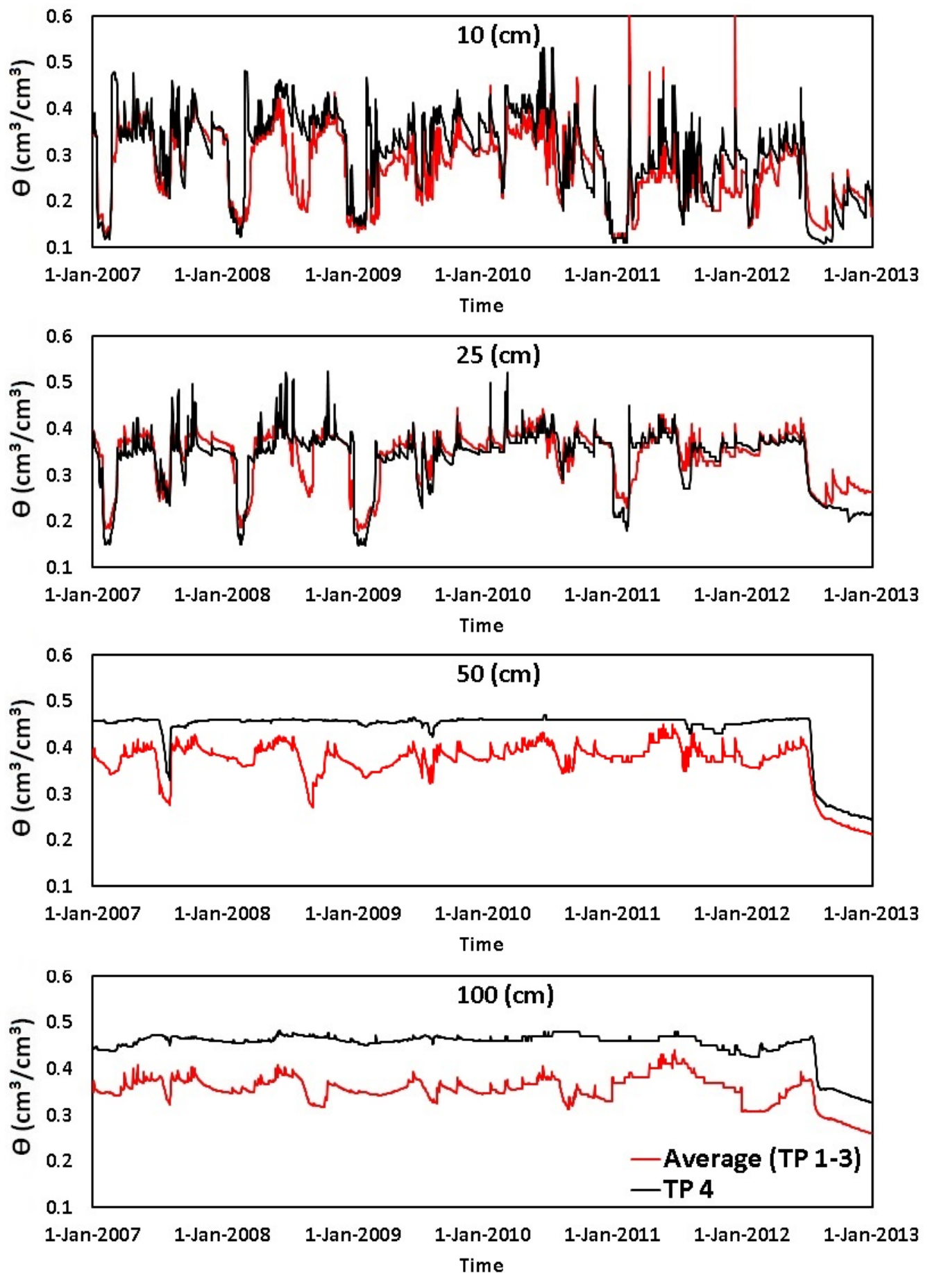
Figure S4. Daily observed SWC ( \theta ) at TP 4 location versus the average observed SWC ( \theta ) at the other three locations (TP 1-3) during study period.
