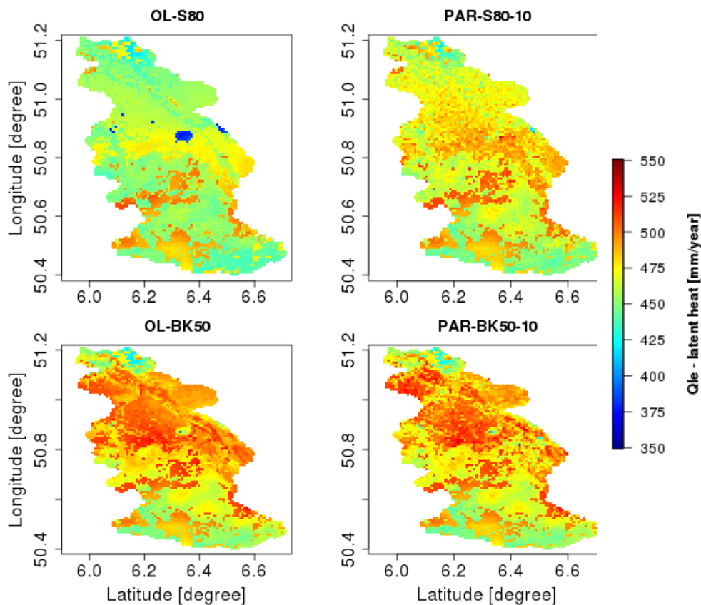
Fig. 8. Annual evapotranspiration (ET) is shown in the year 2013 (evaluation period year 2013 ) for simulations OL-S80, OL-BK50, no assimilation . This figure demonstrates the impact of parameter updates (PAR-S80-10 and PAR-BK50-10) in comparison to open loop (OL-S80) and reference soil map (OL-BK50). ET changes in the North but not as much in the South.
