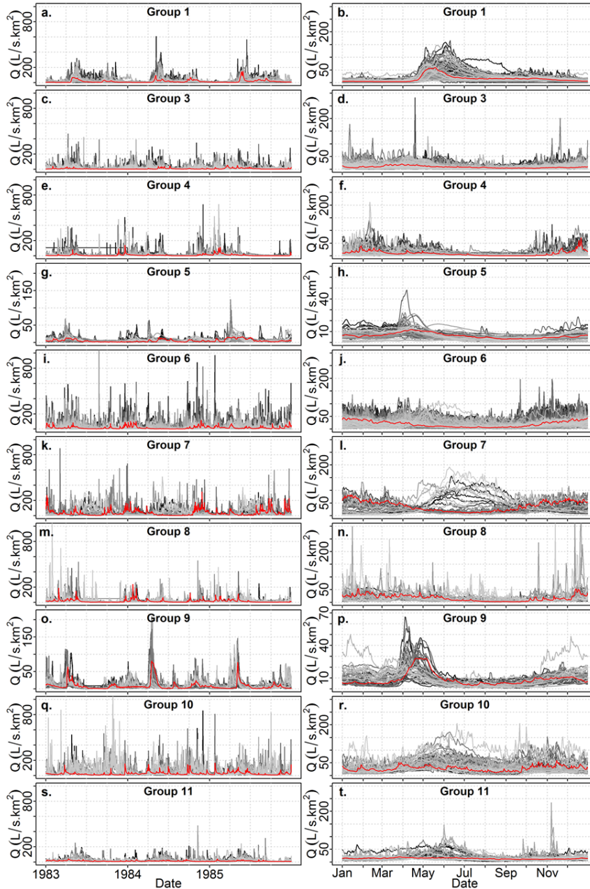
5 Figure 7. 3-years hydrographs (left) and average annual hydrographs based on > 5 years daily flows (right) at the stream gauges of the CART classification classes. Grey->black: all stream gauges belonging to the class; red: stream gauge where the flow signatures are closest to the class median flow signatures. Note that the scales are different for classes 5 and 9 and that this classification doesn't contain any class No. 2 as explained in part 3.2.
