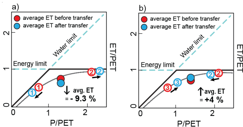
Figure 12. Budyko curve and increase or decrease of average ET when transfer of water from higher location to lower location is included. a) 500 \text{ mm yr}^{-1} of transfer from site 1 (3000 m altitude, lower aridity index) to site 2 (300 m altitude, higher aridity index) decreases the average ET by 9.3 %. b) 500 \text{ mm yr}^{-1} of transfer of water from location 2 (altitude 300 m, higher aridity index) to location 3 (altitude 10 m, lower aridity index) increases the average ET by 4 %.
