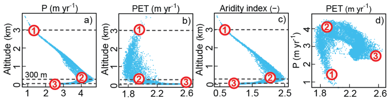
10 Figure 11. Variation of precipitation (P), potential evapotranspiration (PET), and aridity index (P/PET) with altitude in 1° by 1° grid cell of Himalayas in the extent of Fig. 4. (89-90° E, 26-27° N). P and PET for sites 1, 2 and 3 in Fig. 10 are marked in the graphs. Between locations 3 and 2, P and Aridity index increase and PET decreases with altitude. Between points 2 and 1, P and aridity index sharply decrease and PET slightly increases with altitude.
