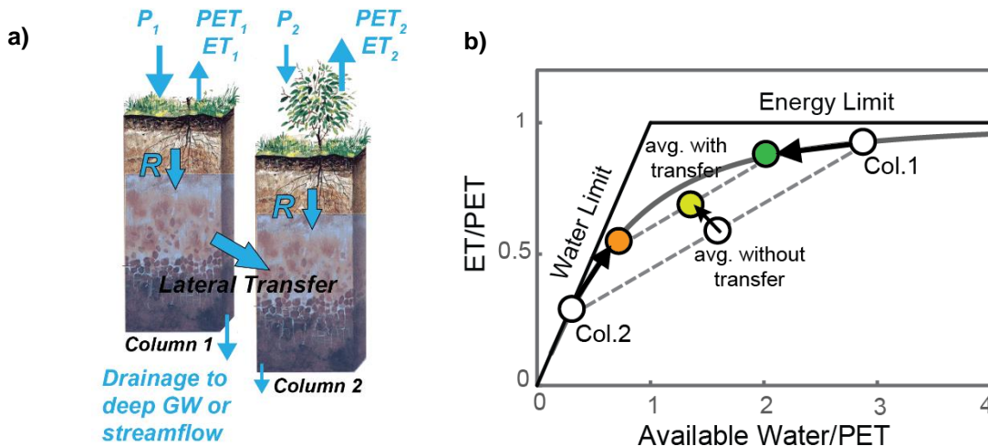
Figure 6. a) A conceptual two-column model. b) Illustration of how the two points representing the two columns shift towards each other in Budyko space if water is transferred from the upper, wetter column to the lower, drier column. Open circles represent columns without lateral transfer and solid circles represent columns with lateral transfer.
