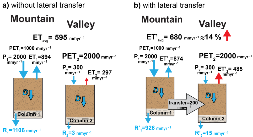
Figure 8. Hypothetical numerical experiment with conceptual two-column model, a) no lateral transfer between columns b) 200 \text{mm yr}^{-1} lateral transfer from column 1 (mountain) to column 2 (valley) increases average ET by 14 %. The magnitude of P (precipitation), PET (potential evapotranspiration), ET (actual evapotranspiration), and R (recharge) are hypothetical and D is drainage to deep groundwater or streamflow.
