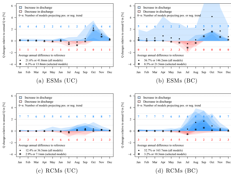
Figure 9. Monthly discharge changes of UC and BC ESM and RCM simulations in [%] under RCP 8.5 (2070-2099). Monthly changes are relative to average annual discharge in the reference period (1970-1999) at gauge El Diem.
