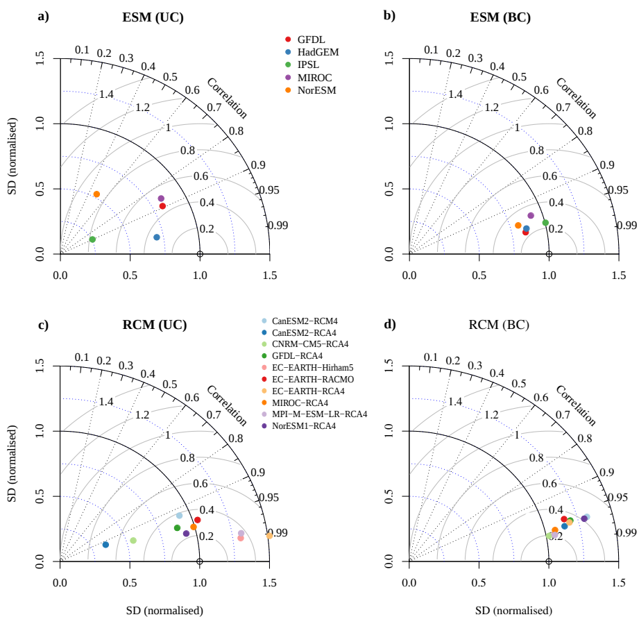
Figure 5. Taylor diagram of average daily discharges in the reference period (1970-1999). It shows R^2 , normalised standard deviation (SD), and normalised SD_D of discrepancies.
