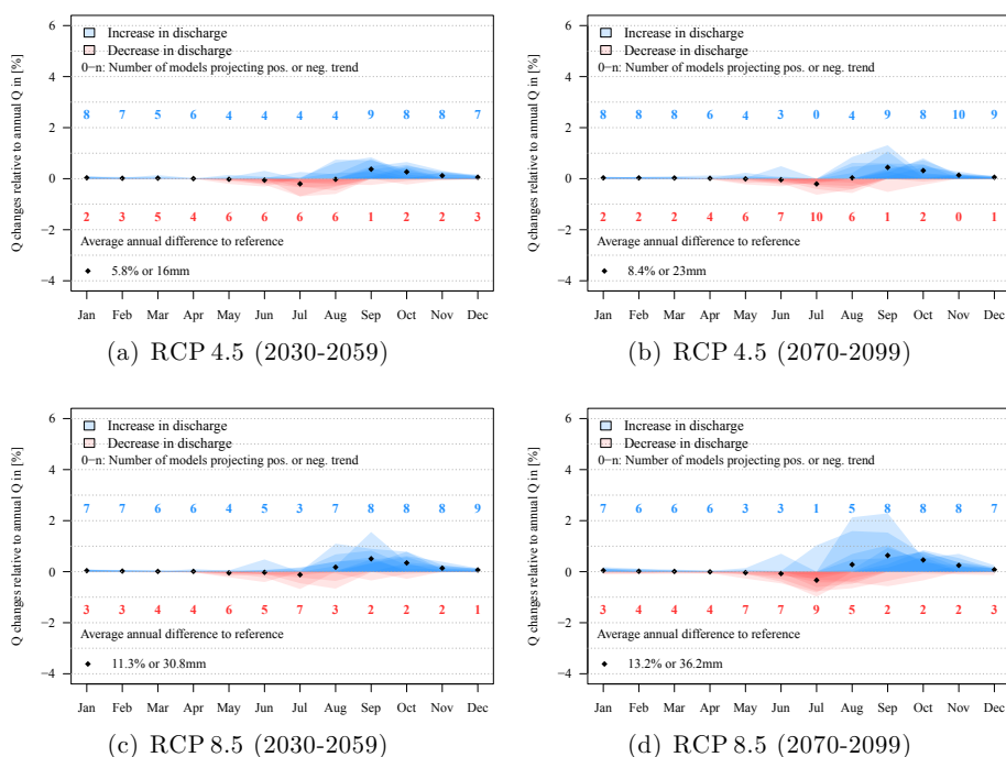
Figure 10. Monthly discharge changes of the selected model ensemble (10 models) relative to average annual discharge in the reference period (1970-1999) at gauge El Diem.
