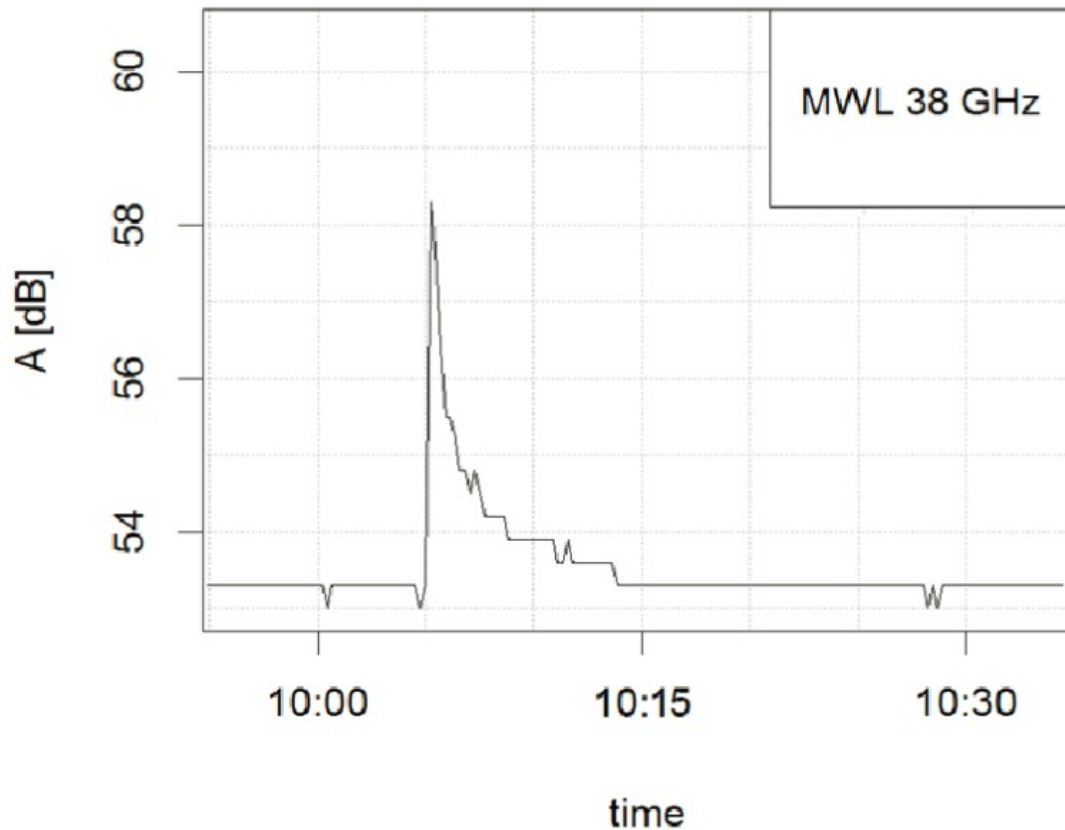
Fig. 1. Wet antenna attenuation of about 5 dB for a 38 GHz CML almost disappears within 3-4 minutes after spraying the antenna radome during dry weather.
