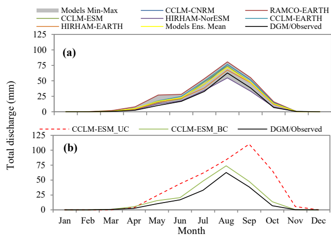
Fig. 7 Historical RCMs-GCMs based discharge simulations and observation based discharge: (a) all RCM rainfall are bias corrected, (b) simulated discharge with bias corrected and not bias corrected rainfall data are compared for CCLM-ESM.
