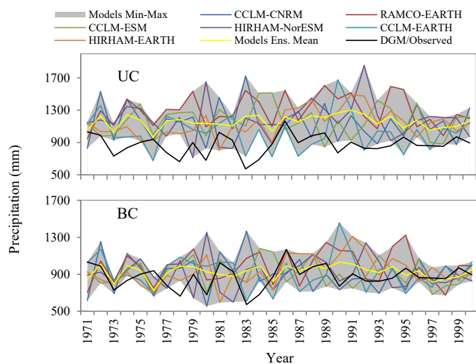
Fig. 3 Historical annual precipitation. UC refers to not bias correct, BC is bias corrected. P-factor equals 50 % and 80 % for UC and BC respectively. R-factor equals 4.3 for UC and 3.2 for BC .
