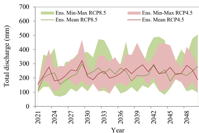
Fig. 9 Projected annual discharge for the climate models ensemble. Simulations are performed with bias corrected precipitation data.
