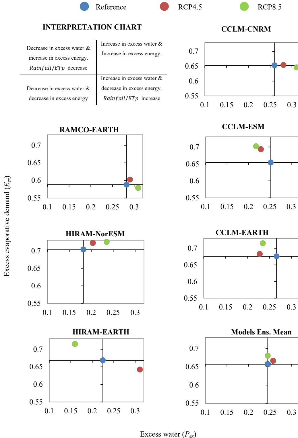
Fig. 10 Plot of excess precipitation ( P_{ex} ) versus evaporative demand ( E_{ex} ) for the reference period (1979-2000) and the emission scenarios RCP4.5 and RCP8.5 (2021-2050) for the RCMs-GCMs ensemble. The shift of RCP dots compared to the reference period's dot indicates the effects of climate change on the catchment hydrology. P_{ex} and E_{ex} for each period are calculated from the annual average rainfall, potential evapotranspiration and actual evapotranspiration.
