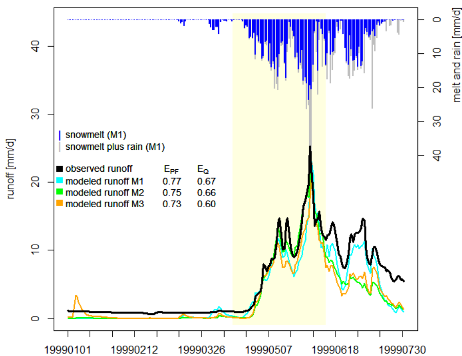
Figure 4. Observed and modeled runoff for the Dischma catchment for year 1999, as well as water input from snowmelt and rain modeled with method M1.
