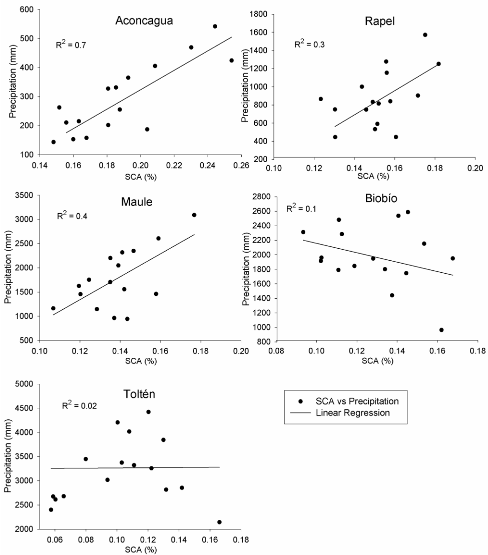
1 2 | Figure 56: Relation between % of mean annual SCA and annual precipitation at Aconcagua, Rapel, Maule, Biobío and 3 Toltén watersheds.
