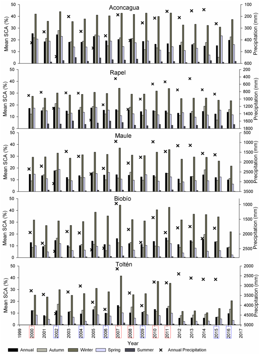
Figure 45: Mean seasonal and annual SCA (%) in Aconcagua, Rapel, Maule, Biobío and Toltén watersheds during 2000–2016. Red boxes indicate Niña years, blue ones Niño years.
