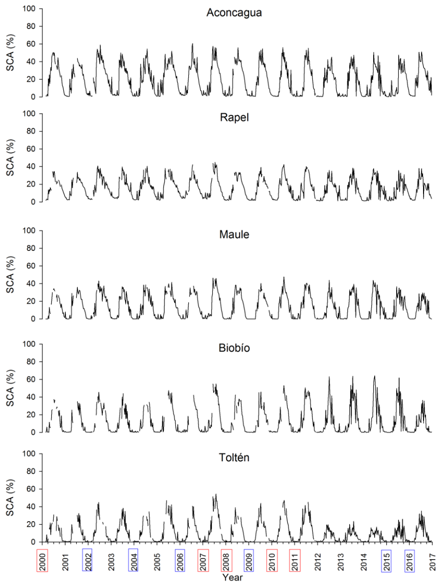
1 2 Figure 34: SCD for the period-2000—2013-2016 period at Aconcagua, Rapel, Maule, Biobío and Toltén 6 watersheds. Red 3 boxes indicate Niña years, blue ones Niño years.
