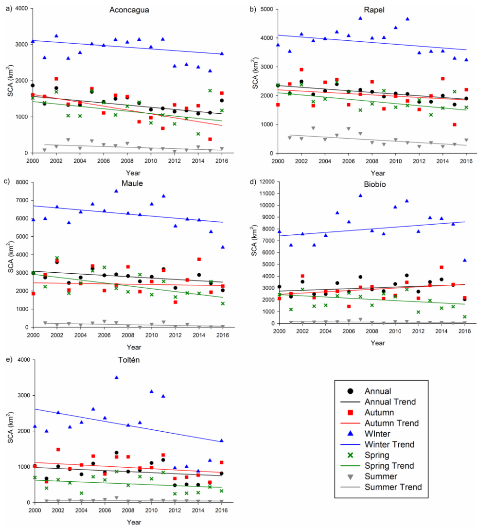
2 Figure 78: Annual and seasonal trend of SCA at Aconcagua, Rapel, Maule, Biobío and Toltén watersheds.
