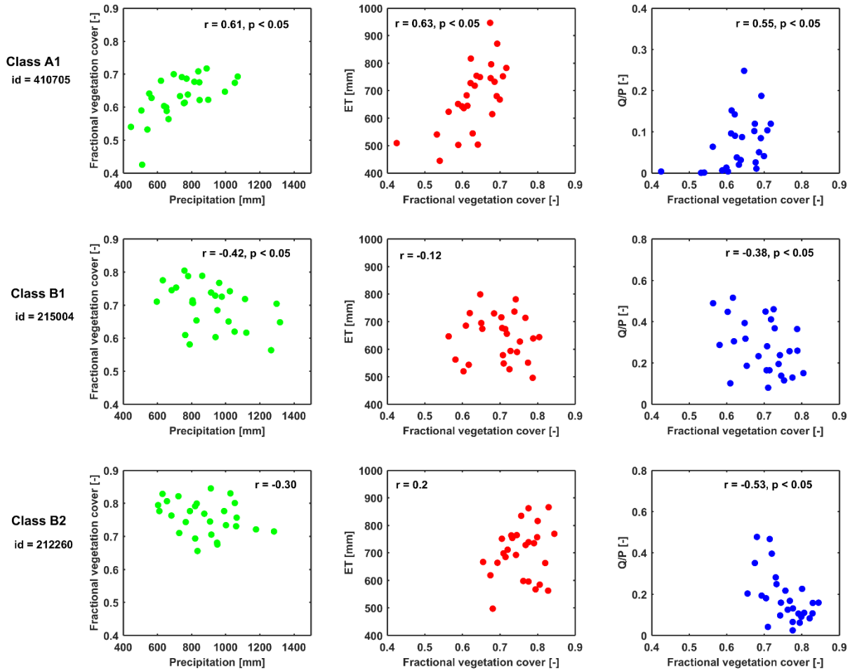
Figure 7: Relationships between catchment averaged annual fractional vegetation cover and annual precipitation (left), water balance derived annual ET (middle) and runoff ratio (right) against mean annual fractional vegetation cover (1984-2010) across three catchments representative of each class in Figure 6. The Spearman rank correlation ( r ) and p -values are shown when correlation is significant.
