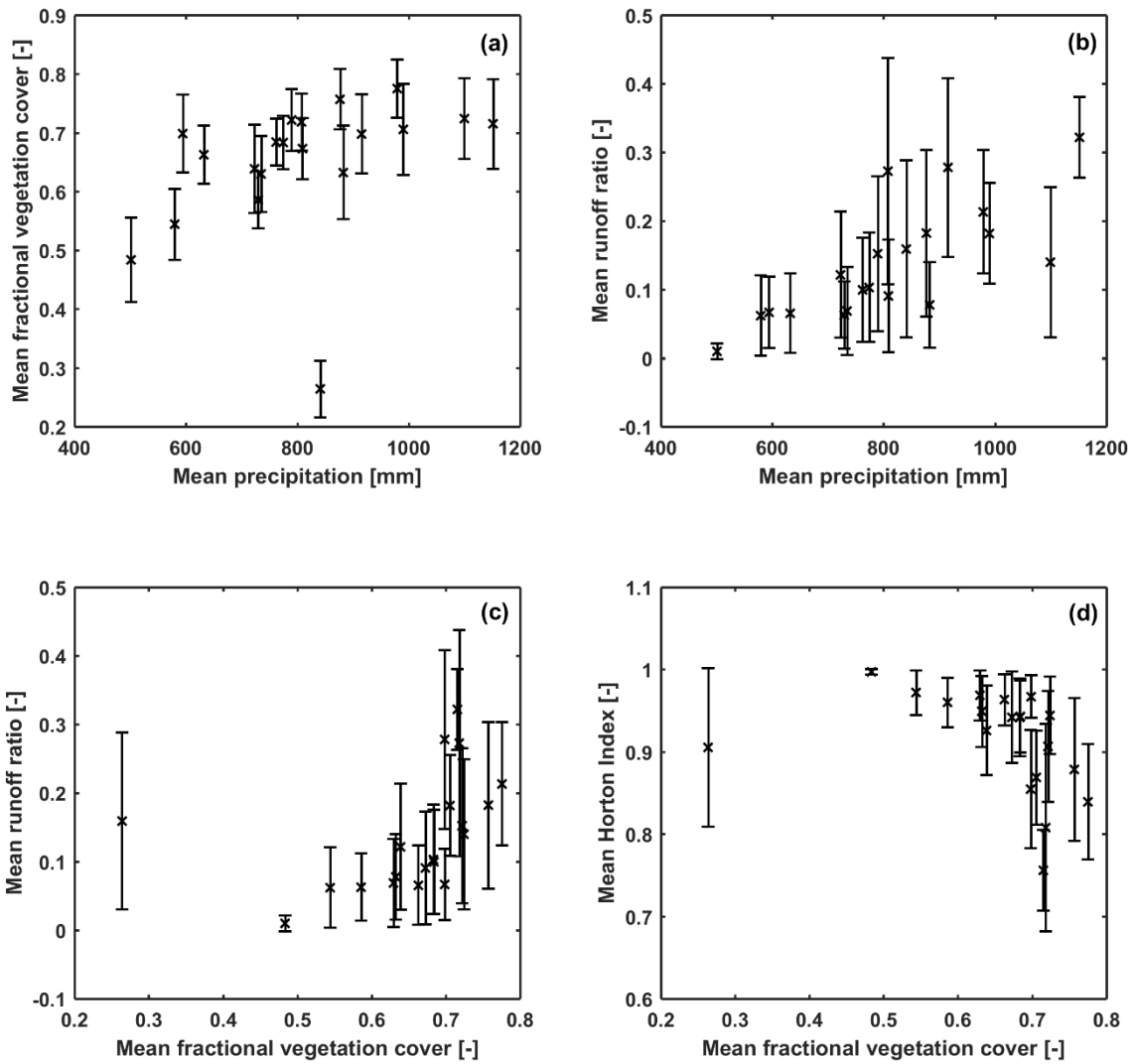
Figure 2: Mean and standard deviation of catchment averaged a) annual fractional vegetation cover, and b) annual runoff ratio, against mean annual precipitation (P) in catchments with non-stationary hydrologic response. c) mean and standard deviation of annual runoff ratio, and d) Horton Index versus catchment averaged annual fractional vegetation cover.
