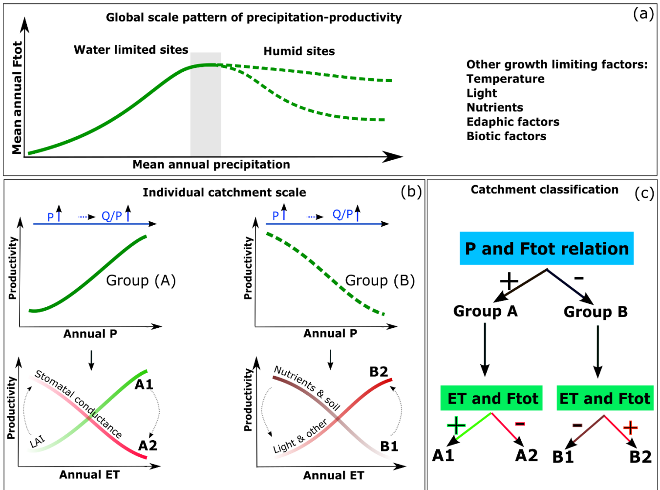
Figure 6: a) Global pattern of annual productivity ( F_{tot} ) and mean annual precipitation relationship. While precipitation is the primary factor for vegetation growth in water limited sites, productivity reaches an asymptote in humid areas or decreases (e.g. tropical forests) with increases in precipitation due to biogeochemical or edaphic constraints. The grey region corresponds to catchments in which productivity is insensitive to inter-annual precipitation variability. b) A conceptual framework for characterizing changes in runoff ratio to changes in annual precipitation and vegetation productivity ( F_{tot} ) in relation to catchment's hydroclimatic condition. In group (A) catchments a positive relationship between annual precipitation and productivity exists and annual ET changes in relation to productivity depend on the dominance of structural control (increases in LAI, class A1) versus physiological control (decreases in stomatal conductance, class A2) in controlling productivity. In group (B) catchments, an inverse relationship between precipitation and productivity exists and productivity
