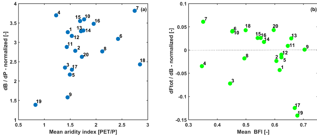
Figure 5: a) Normalized baseflow ( B ) sensitivities to annual precipitation ( P ) in each catchment with non-stationary hydrologic response against its mean aridity index (1984-2010), b) normalized annual fractional vegetation cover ( F_{tot} ) sensitivities to annual baseflow of each catchment with non-stationary hydrologic response against its mean baseflow index (BFI) (1984-2010). Data labels refer to the station identification number in Table 1. In general, annual baseflow sensitivities to mean annual precipitation decreases in wetter catchments (smaller aridity index). Positive sensitivities of fractional vegetation cover to baseflow decreases in catchments with higher baseflow index. Negative fractional vegetation cover sensitivities to baseflow become more negative in catchments with higher baseflow index indicating larger contribution of groundwater to stream flow.
