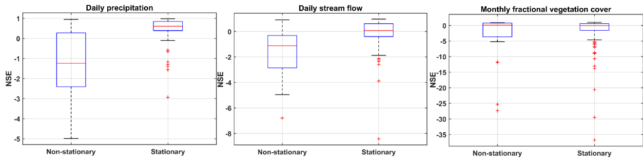
Figure 8: Box plots of NSE values calculated between the regime curves of pre-drought and drought periods in catchments with non-stationary (20 catchments) and stationary (146 catchments) hydrologic response respectively. Changes in daily precipitation and runoff and monthly fractional vegetation cover were larger in catchments with non-stationary hydrologic response.
