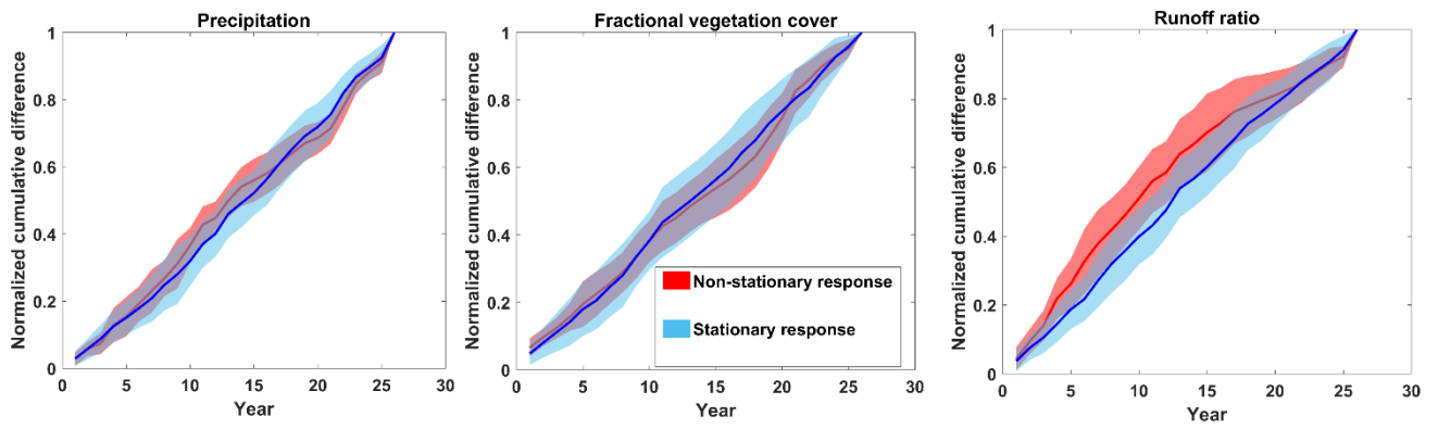
Figure 3: Mean normalized cumulative absolute differences in annual precipitation, fractional vegetation cover and runoff ratio between catchments with non-stationary (20 catchments) and stationary (146 catchments) hydrologic response. The shaded areas represent standard deviation.
