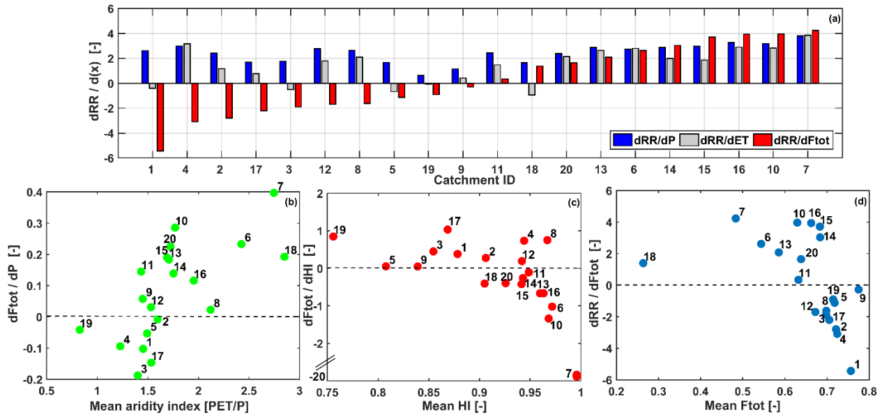
Figure 4: a) Normalized sensitivities of runoff ratio (RR) to precipitation (P), water balance ET and fractional vegetation cover (Ftot), normalized sensitivities of annual: b) fractional vegetation cover to precipitation against catchments' mean aridity index, c) fractional vegetation cover to Horton index (HI) against catchments' mean Horton Index, and d) runoff ratio to fractional vegetation cover against catchments' mean fractional vegetation cover in catchments with non-stationary hydrologic response. Data labels refer to the station identification number in Table 1.
