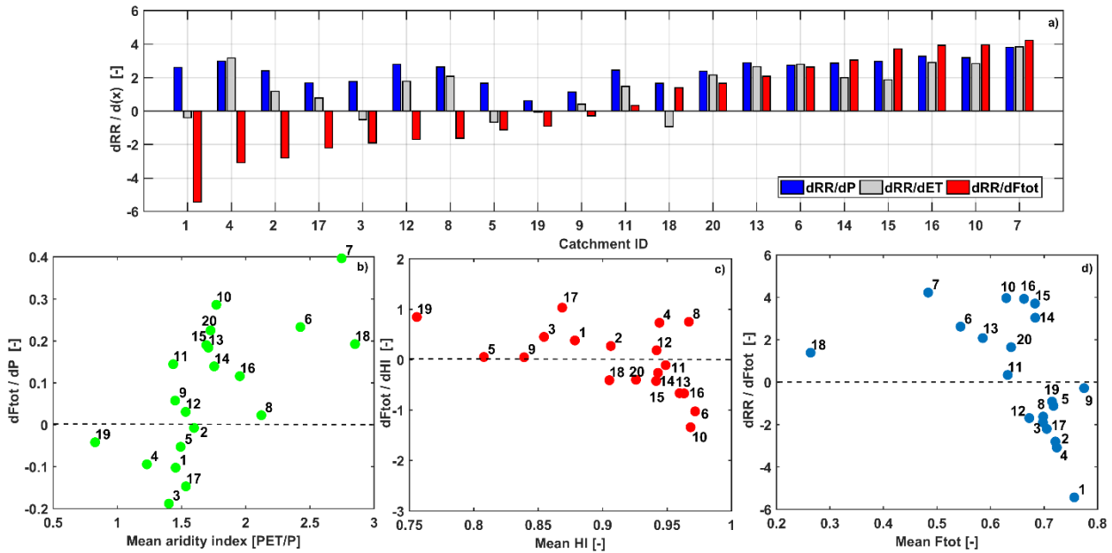
Figure 4: a) Normalized sensitivities of runoff ratio (RR) to precipitation (P), water balance ET and fractional vegetation cover (Ftot), normalized sensitivities of annual: b) fractional vegetation cover to precipitation against catchments' mean aridity index, c) fractional vegetation cover to Horton index (HI) against catchments' mean Horton Index, and d) runoff ratio to fractional vegetation cover against catchments' mean fractional vegetation cover in catchments with non-stationary hydrologic response. Data labels refer to the station identification number in Table 1.
