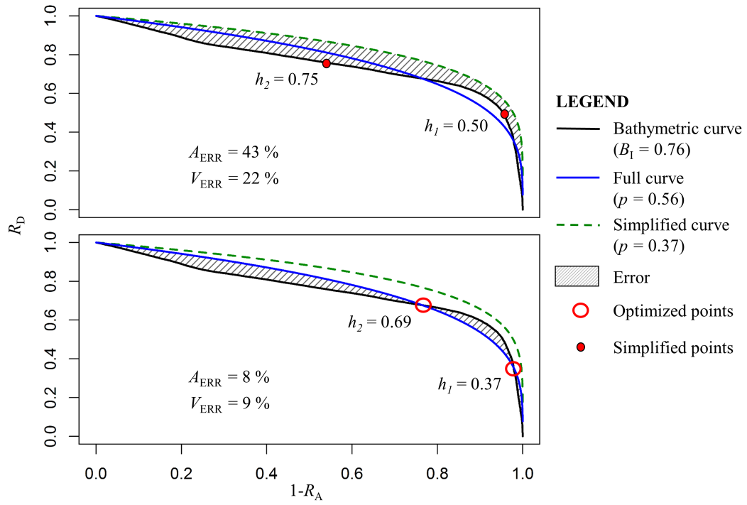
Fig. 8. Comparison of the hypsometric curve for Pond 7 with the Full and Simplified curve. The top shows the area ( A_{ERR} ) and volume ( V_{ERR} ) error associated with the Simplified curve that was calculated using Simplified depths h_1 and h_2 and the bottom shows the error associated with the Full curve and the optimum location for depths h_1 and h_2 . R_D is relative depth, R_A is relative area, B_1 is the bathymetric integral, and p is the morphometry coefficient.
