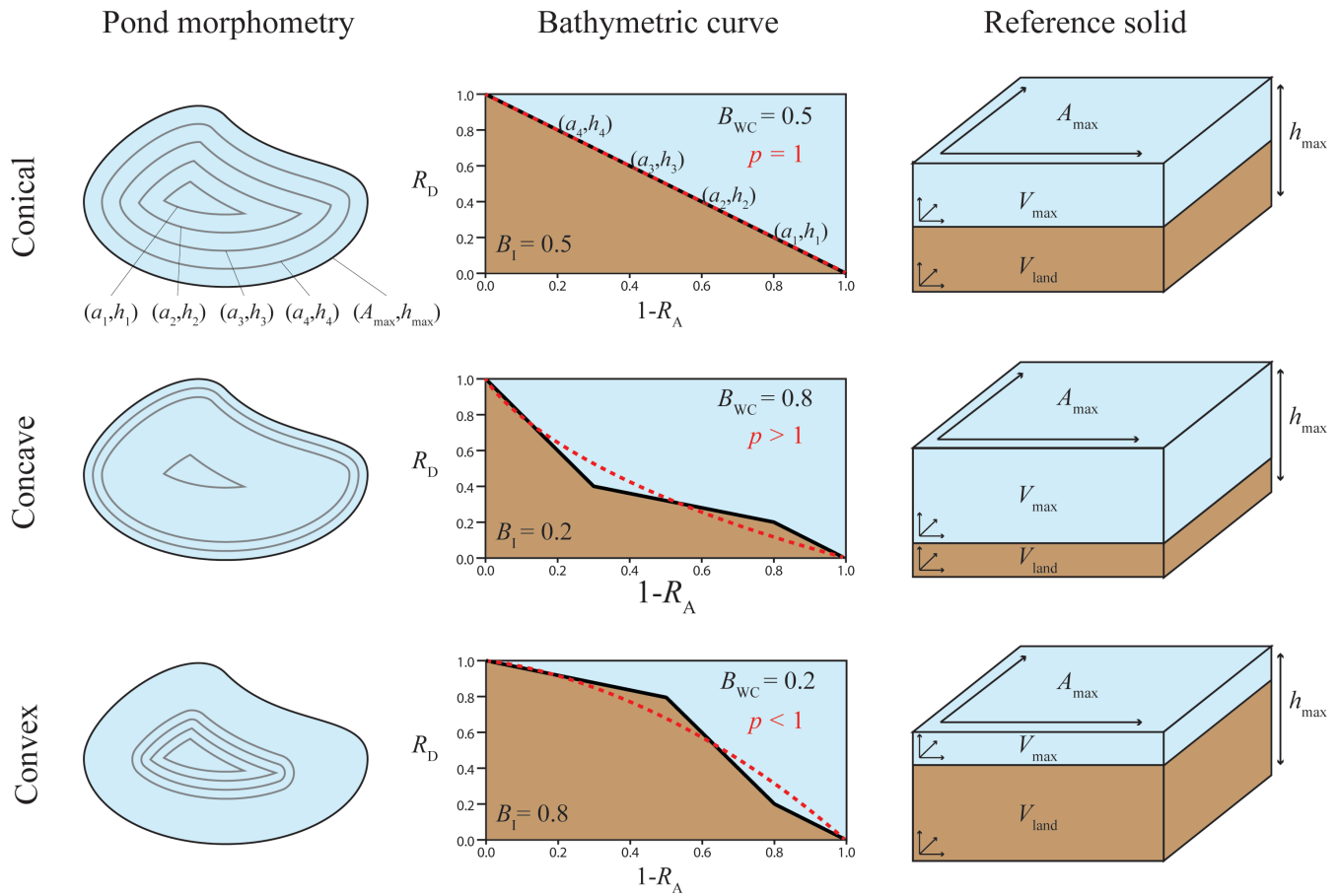
Fig. 1. Perceptual diagram of the relationship between morphometric variables. The area ( a ) at a given stage of the pond ( h ) is a point on the bathymetric curve (thick black line), where R_A is the relative area and R_D is the relative depth. The bathymetric integral ( B_I ) is the integration of everything below the bathymetric curve and the pond's capacity to store water ( B_{WC} ) is the integration of everything above the bathymetric curve. The morphology ( p ) coefficient represents the shape of the bathymetric curve in the power function equation (red-dashed line; Eq. (7)). The reference solid is the box created by multiplying the maximum height of the dam ( h_{max} ) by the maximum surface area created by the pond ( A_{max} ), and is entirely comprised of land ( V_{land} ) and/or water ( V_{max} ) proportional to B_I and B_{WC} .
