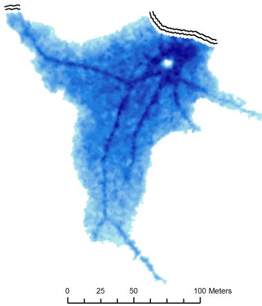
Fig. 2. Four examples of detrended beaver pond DEMs used for this study, one from each study area. ( S_I = shape index, B_I = Bathymetric integral, B_{WC} = Bathymetric water capacity, p = Morphometry coefficient, s = Scaling coefficient, D_{len} = Dam length, h_{max} = Maximum height of the dam, A_{max} = Maximum surface area of the pond, and V_{max} = Maximum volume of the pond)
