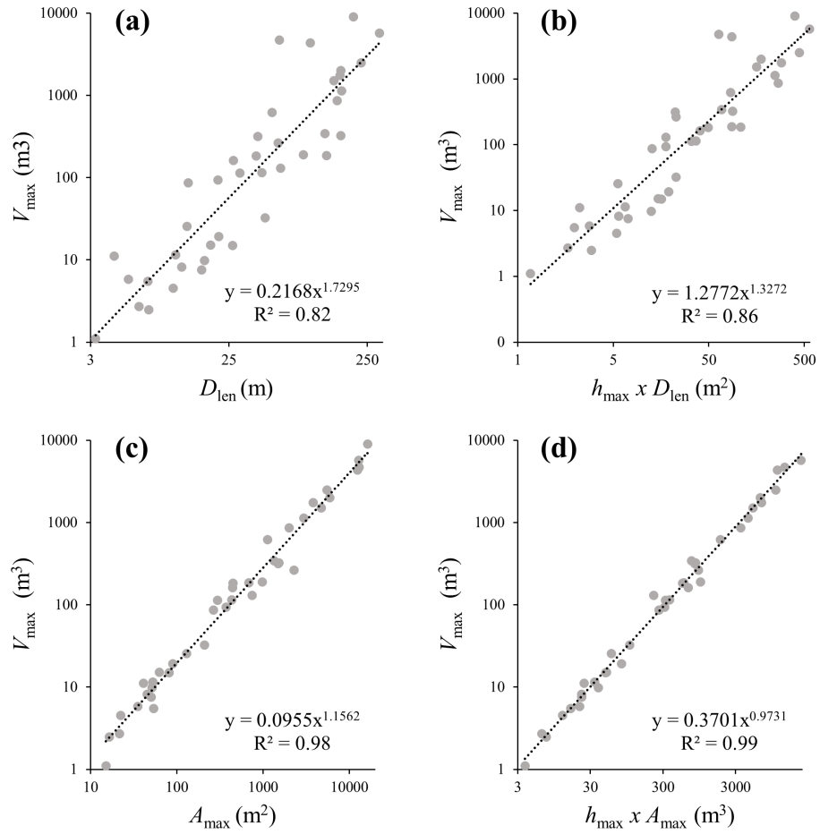
10 Fig. 3. Power regression relationships between the maximum volume of the beaver ponds ( V_{\max} ) and: (a) the length of the beaver dams ( D_{\text{len}} ); (b) the product of the maximum depth of the ponds ( h_{\max} ) and the length of the beaver dams; (c) the maximum surface area ( A_{\max} ) of the ponds; and, (d) the product of the maximum surface area and maximum depth of the pond.
