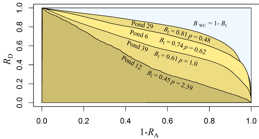
Fig. 5. Bathymetric curves for ponds shown in Figure 1. R_D is relative depth, R_A is relative area, B_1 is the bathymetric integral, B_{WC} is the bathymetric water capacity, and p is the morphometry coefficient.
