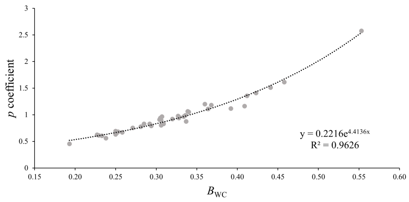
Fig. 6. Relationship between the morphometry ( p ) coefficient and the bathymetric water capacity ( B_{WC} ).
