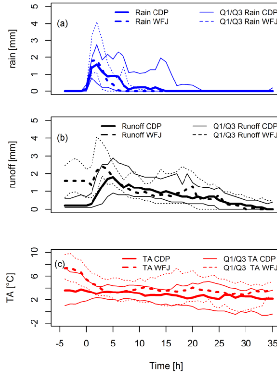
5 Figure 7: (a) Temporal course of median rain (a), measured snowpack runoff (b) and air temperature (c) for WFJ (dotted) and CDP (solid) aggregated over all 40 and 61 events respectively. The thinner lines represent the lower and upper quartiles, respectively. The displayed period is extended by 5 hours prior to event beginning according to the event definition (0 h).
