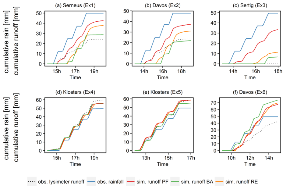
Figure 4: Cumulative rain and snowpack runoff displayed for the six sprinkling events. Ex1 (a) - Ex3 (c) were conducted during winter conditions, Ex4 (d) – Ex6 (f) were conducted during spring conditions.
