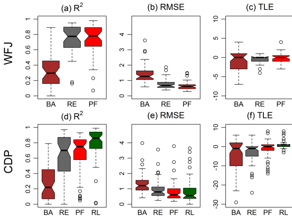
5 Figure 8: RMSE, R^2 and TLE for simulations of 61 ROS events at the CDP site and of 40 ROS events at the WFJ site for all models (BA, RE, PF) and the reference lysimeter (RL) available only for CDP.
