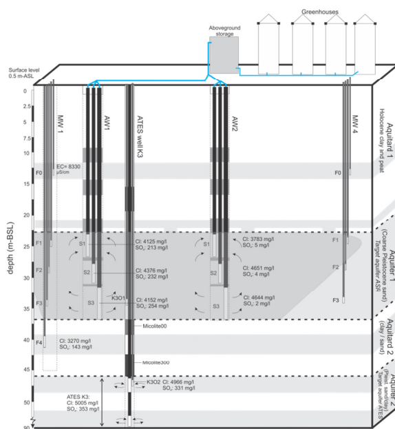
15 Figure 1: Cross-section of the Westland ASR site to schematize the geology, ASR wells, ATEs well, and the typical hydrochemical composition of the native groundwater. Horizontal distances not to scale.
