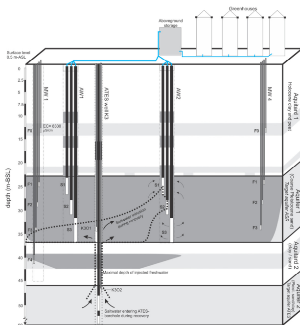
Figure 11: Deep saltwater intrusion via the current ATEs K3 borehole during shallow recovery of injected freshwater at the Westland ASR site at the start of Cycle 2.
