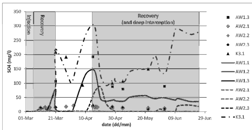
Figure 9: Modelled and observed \text{SO}_4 -concentrations at the most relevant well screens.
