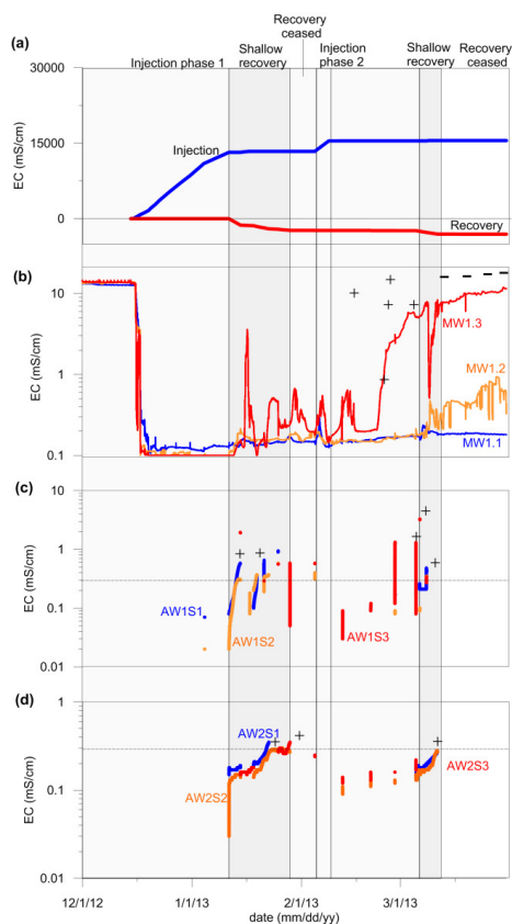
10 Figure 5: Pumping of the ASR system during cycle 1 (2012/2013), EC observations at MW1 (5 m from AW1), and the EC in the recovered water at AW1 and AW2. MW= monitoring well, AW= ASR well.
