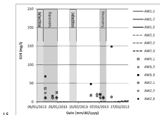
15 Figure 6: Modelled (solid lines) and observed (data points) \text{SO}_4 concentrations without borehole leakage. High concentrations indicate admixing of deeper saltwater. Observed \text{SO}_4 concentrations by far exceed the modelled concentrations.
