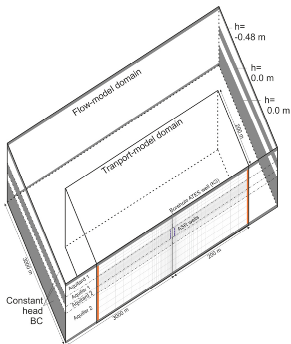
Figure 3: Set-up of the Westland ASR groundwater transport model (half-domain).
