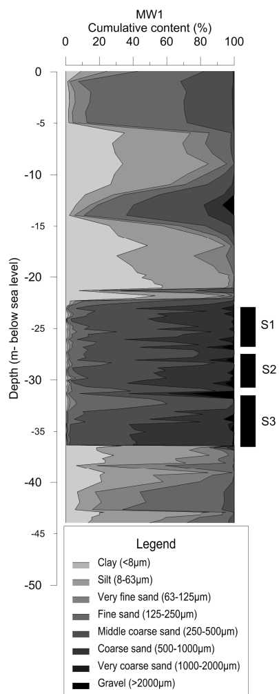
5 Figure 4: Cumulative grain size contents observed at MW1 (at 5 m from ASR well 1) in this study. S1-S3 mark the depth intervals of the ASR well screens.
