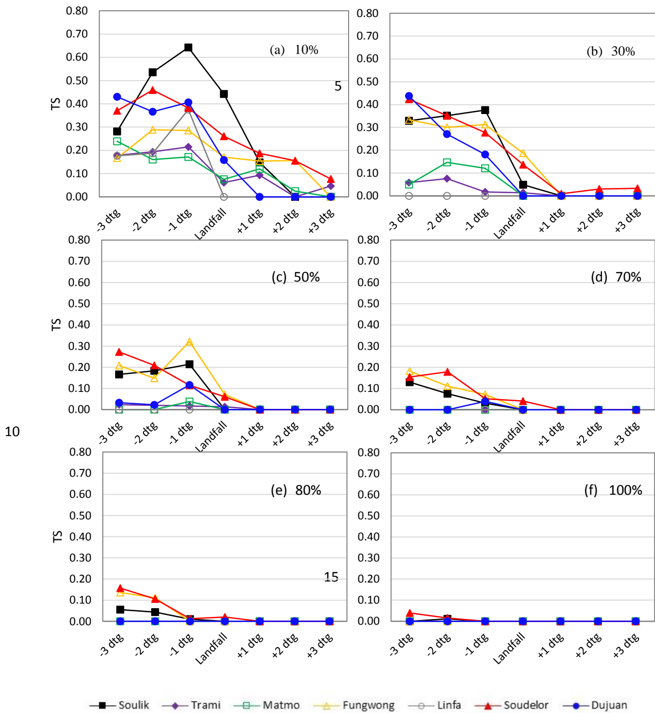
Figure 7: Comparisons of TS performance with a 1- to 24-h lead time considering various probability thresholds without a data assimilation technique.
