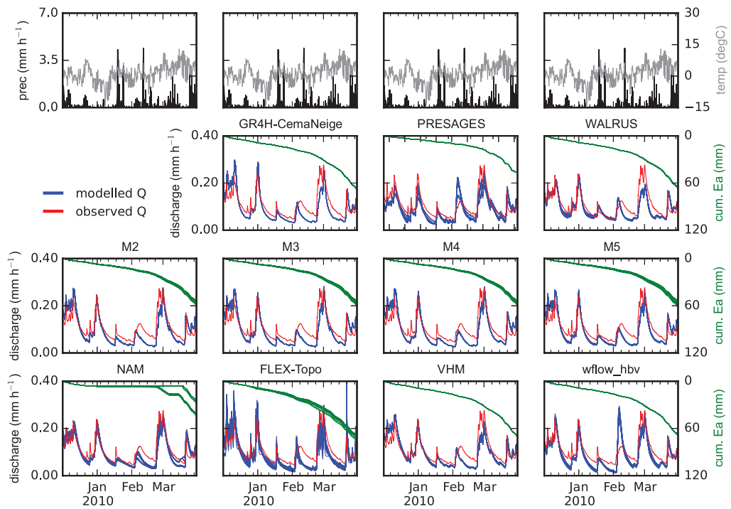
Figure 38: Ourthe Occidentale at Ortho
