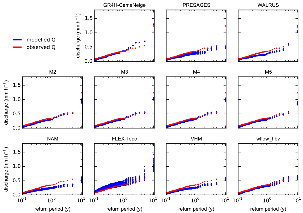
Figure 13: Ourthe Occidentale at Ortho
