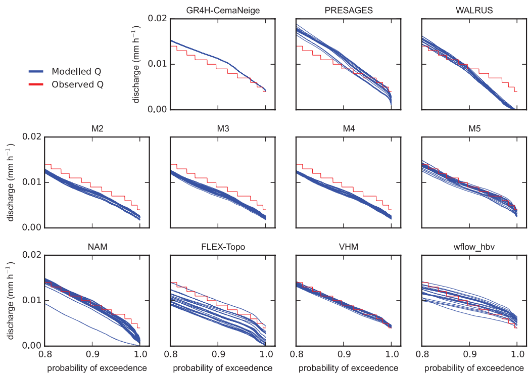
Figure 18: Ourthe Occidentale at Ortho
