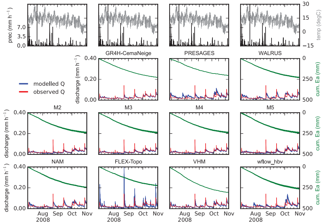
Figure 23: Ourthe Occidentale at Ortho
