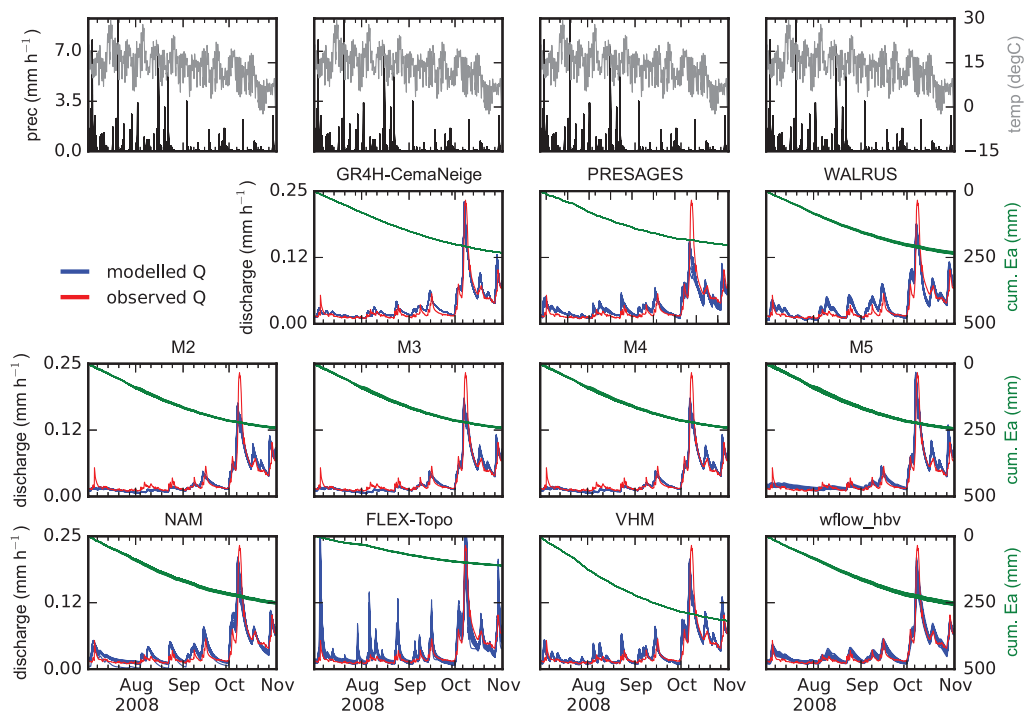
Figure 25: Semois at Membre
