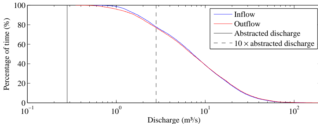
Figure 42: Flow duration curves of inflow and outflow discharge at the dam.
