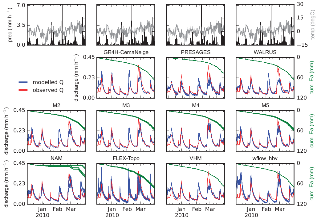
Figure 37: Ourthe Orientale at Mabompré
