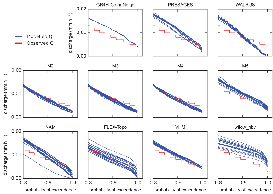
Figure 17: Ourthe Orientale at Mabompré
