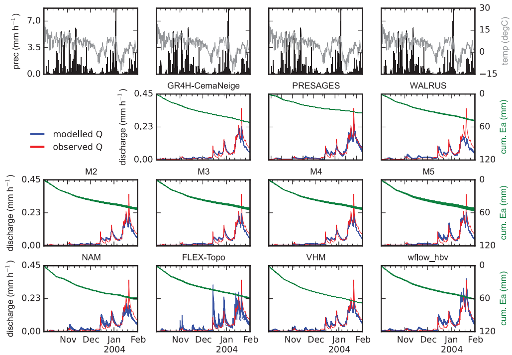
Figure 28: Ourthe Occidentale at Ortho
