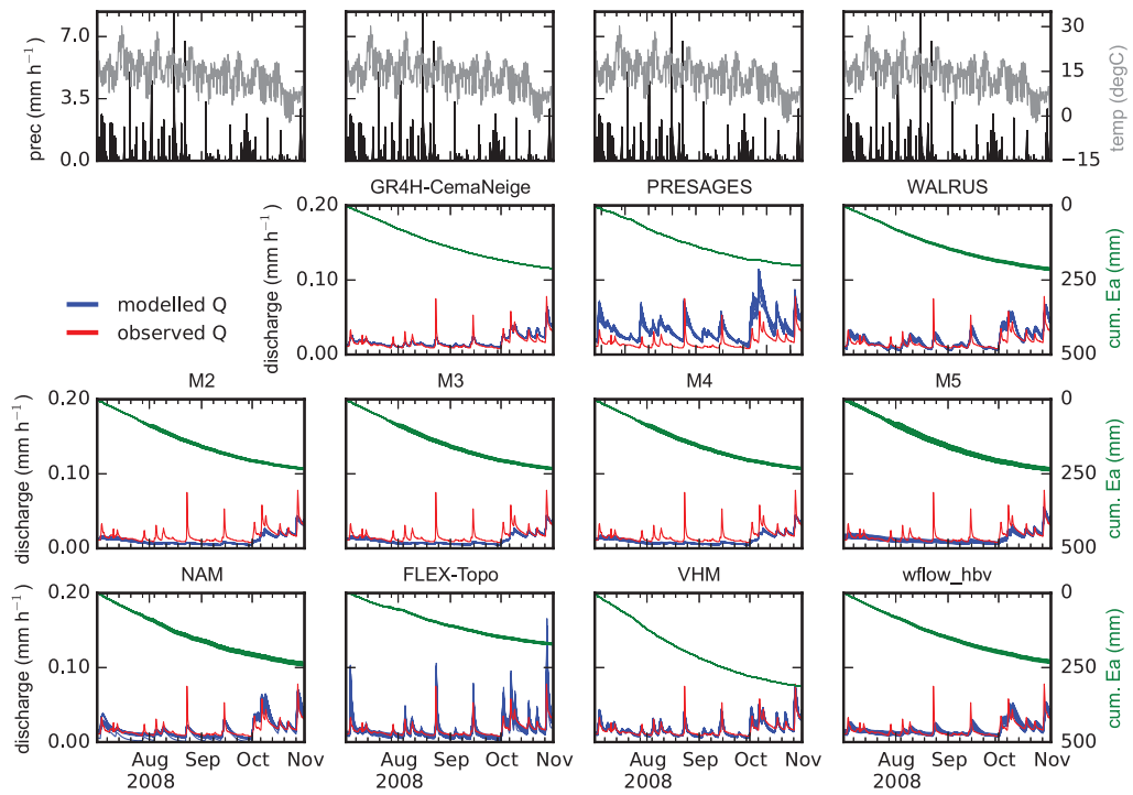
Figure 24: Lesse at Gendron
