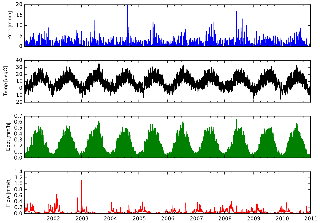
Figure 2: Ourthe Orientale at Mabompré
