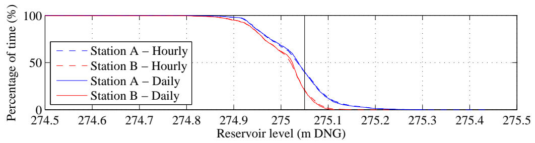
Figure 45: Percentage of time during which the reservoir level exceeds the indicated value.
