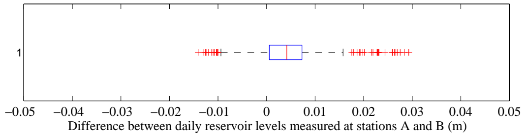
Figure 46: Boxplot of the difference between the daily measurements of the reservoir level at stations A and B.
