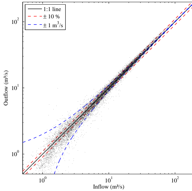
Figure 43: Daily outflow discharge vs inflow discharge at Nisramont reservoir.
