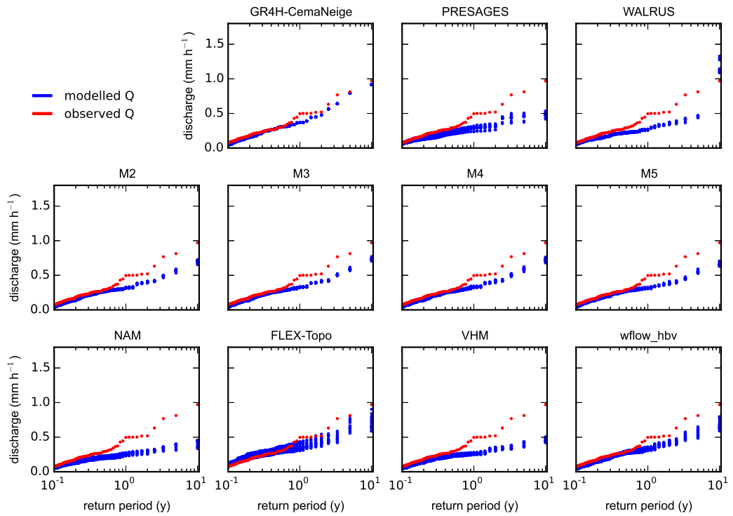
Figure 14: Lesse at Gendron; note that the y-axis deviate from the figure in the paper, to make it similar to the other plots in this section
