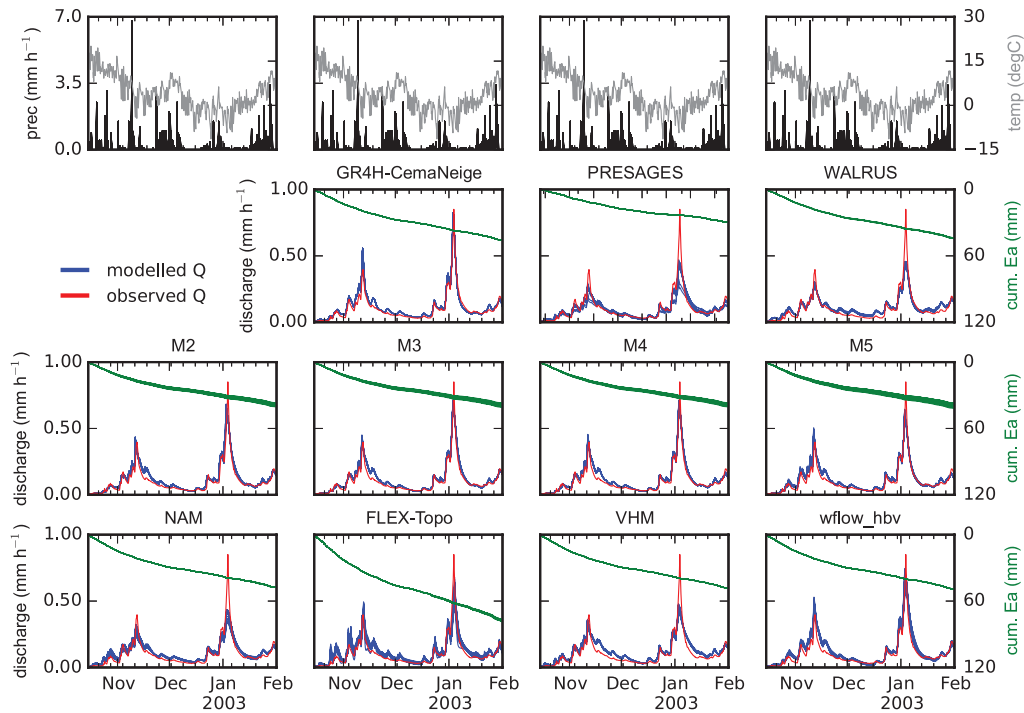
Figure 31: Ourthe at Tabreux
