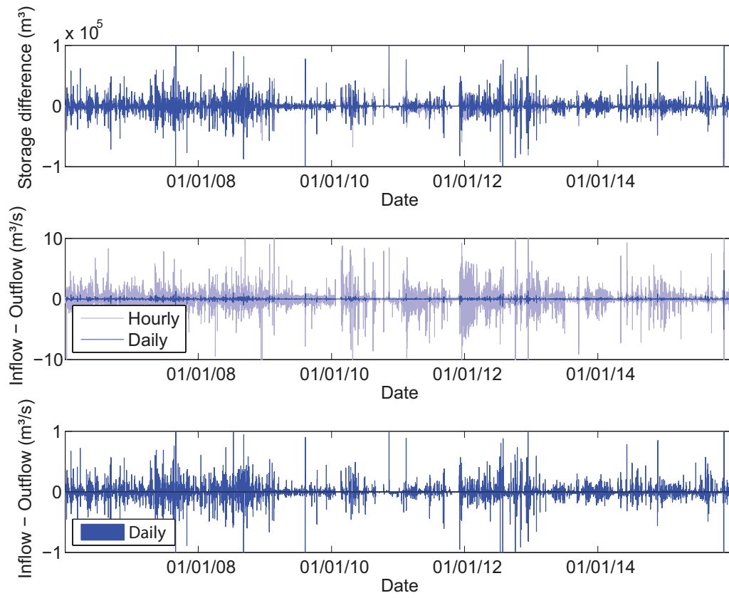
Figure 48: Hourly and daily storage variations in Nisramont reservoir (top) and corresponding differences between upstream and downstream of the reservoir (middle and bottom).
