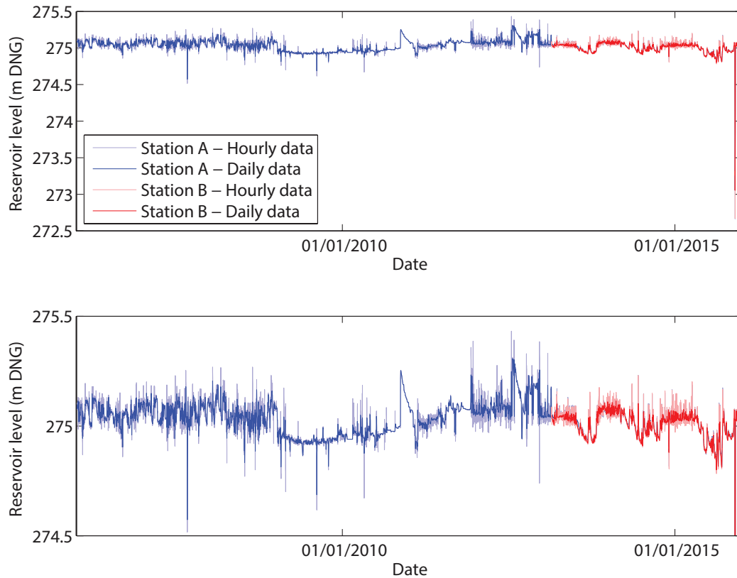
Figure 44: Hourly evolution of the level in Nisramont reservoir.
