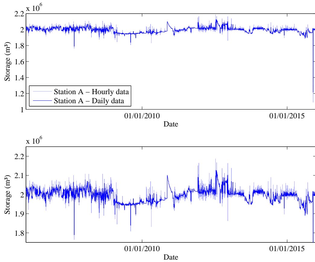
Figure 47: Hourly evolution of storage in Nisramont reservoir.
