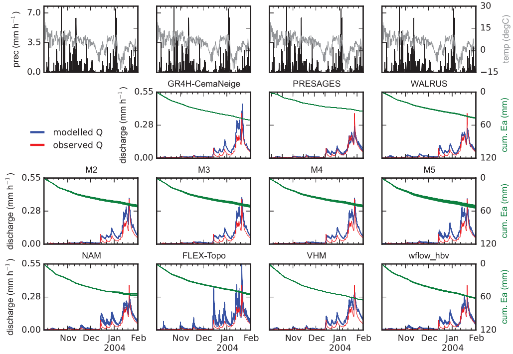
Figure 27: Ourthe Orientale at Mabompré
