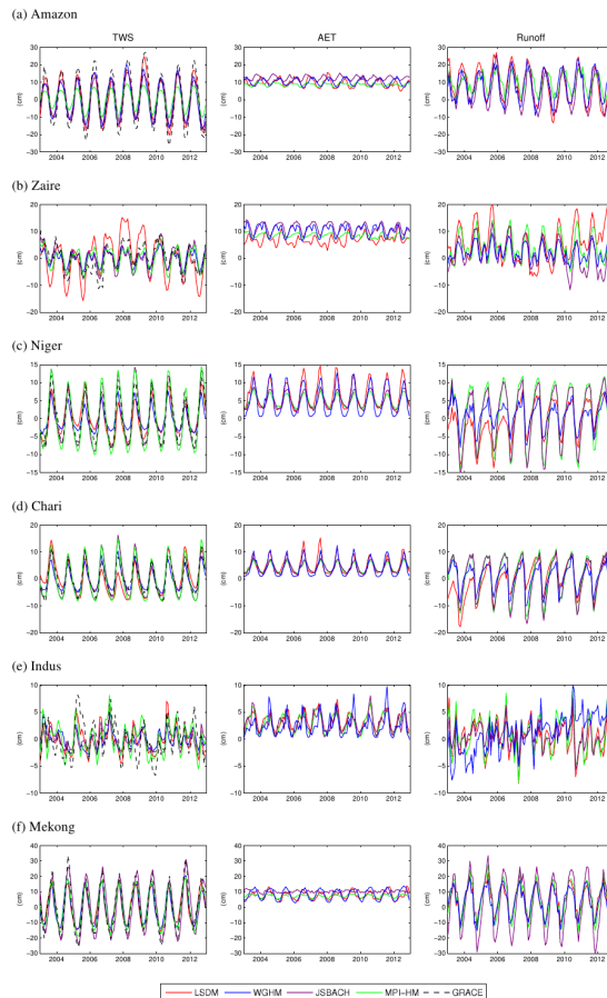
Fig. 3. Time series of TWS from GRACE and models, model simulated AET time series and model simulated runoff time series; each for six different catchments: Amazon, Zaire, Niger, Chari, Indus and Mekong.
