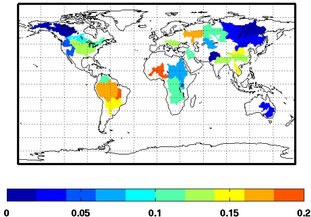
Fig. 1. The differences between the explained variance values from WGHM with and without groundwater.
