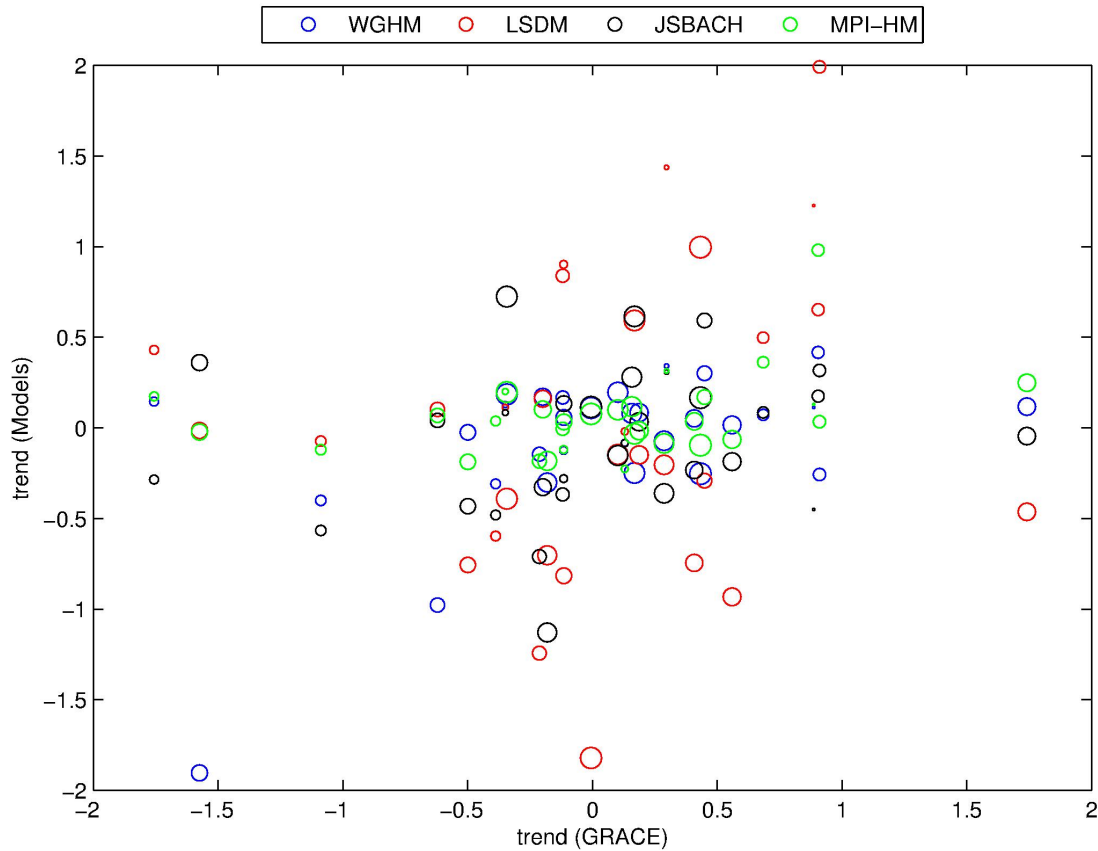
Fig. 2. The scatter plot comparing trends from the models and those from GRACE in the 31 basins. Symbol size varies with river basin area.
