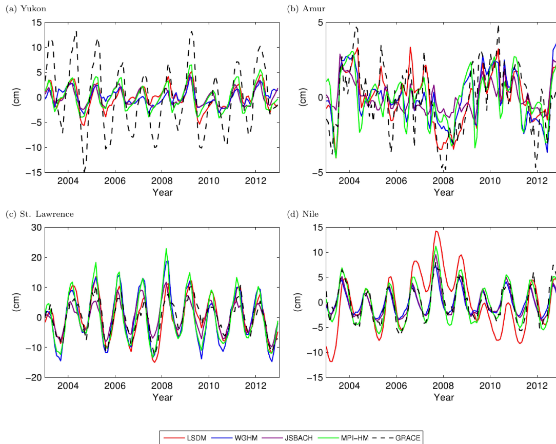
Fig. 4. Examples of monthly TWS time series from GRACE and models for the basins with the largest deviation between model and GRACE in each of the four metrics.
