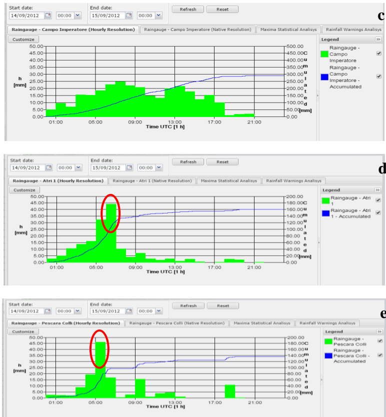
Figure 3: Rain gauges time series of some selected stations in Marche (a, Fermo and b, Pintura di Bolognola) and Abruzzo (c, Campo Imperatore, d, Atri and e, Pescara Colli) regions during the event of 14 September 2012. The green histogram represents the hourly accumulated precipitation (scale on the left); the blue line represents the incremental accumulation within the 24h (scale on the right). (courtesy of Italian Civil Protection Department)
