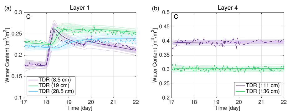
Figure 4. Forecast at the measurement positions of the top and bottom layer during time period C. The solid lines show the mean value of a total of 100 different forecasts. The pale colors show the results from 25 of these with soil parameters, Miller scaling parameters and boundary condition sampled from the distributions estimated with the Standard EnKF and the initial condition, that was actually used for the estimation itself. The dashed line shows the measurements.
