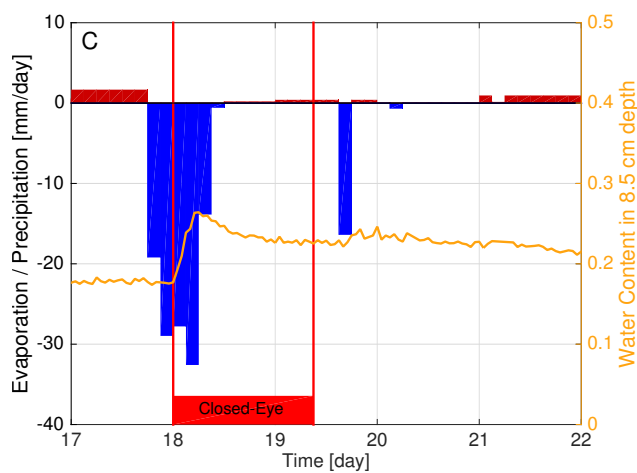
Figure 8. Boundary condition along with the topmost TDR water content measurements during time period C. The closed-eye time period was determined based on the changes in parameter K_0 . During this time the dynamics cannot describe the water content measurements any more, most likely because of the violation of the local equilibrium assumption.
