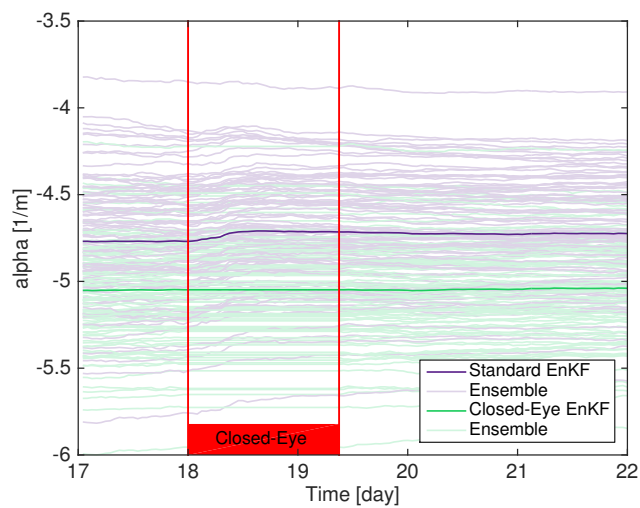
Figure 6. Parameter \alpha during the last iteration of the Standard EnKF and the Closed-Eye EnKF.
