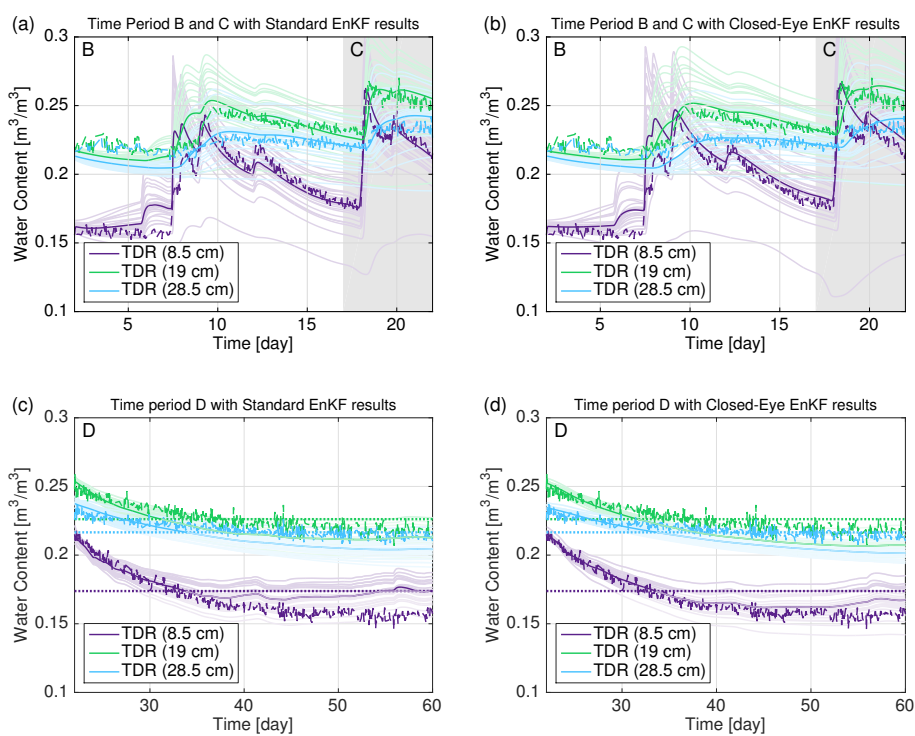
Figure 10. Forecast at the measurement positions of the first layer during time period B and C (a,b) as well as D (c,d). The solid lines show the mean value of a total of 100 different forecasts. The pale colors show the results from 25 of these with soil parameters and Miller scaling parameters sampled from the distributions estimated with the Standard EnKF (a,c) and Closed-Eye EnKF (b,d). The dashed line shows the measurements, the dotted line the lowest water content measured during time period C, indicating the lower limit of the water content range, for which the parameters are deemed valid.
