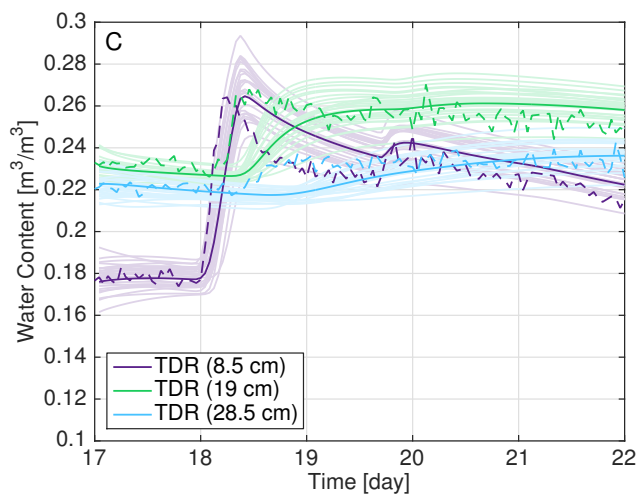
Figure 9. Forecast at the measurement positions of the first layer during time period C with the results from the Closed-Eye EnKF. The solid lines show the mean value of a total of 100 different forecasts. The pale colors show the results from 25 of these with soil parameters, Miller scaling parameters and boundary condition sampled from the distributions estimated with the Closed-Eye EnKF and the initial condition, that was actually used for the estimation itself. The dashed line shows the measurements.
