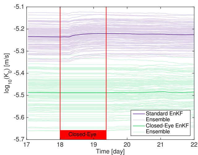
Figure 5. Saturated conductivity K_0 during the last iteration of the Standard EnKF and the Closed-Eye EnKF.
