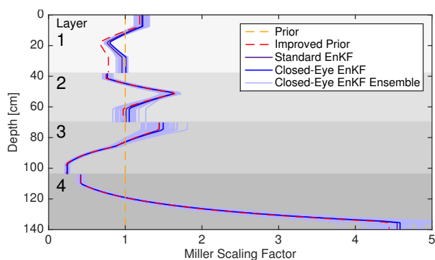
Figure 3. Mean values of the Miller scaling field. Soil layers are indicated by different gray scales. The heterogeneity is a priori unknown and the according prior is set to 1. The natural logarithm of the scaling factors is estimated at the measurement locations and interpolated linearly between (with constant extrapolation to layer boundaries). Already the improved prior can describe the main features. The further estimations with the Standard and Closed-Eye EnKF lead to further small changes mainly in the first layer. For the Closed-Eye EnKF the actual ensemble indicating the uncertainties is additionally shown.
