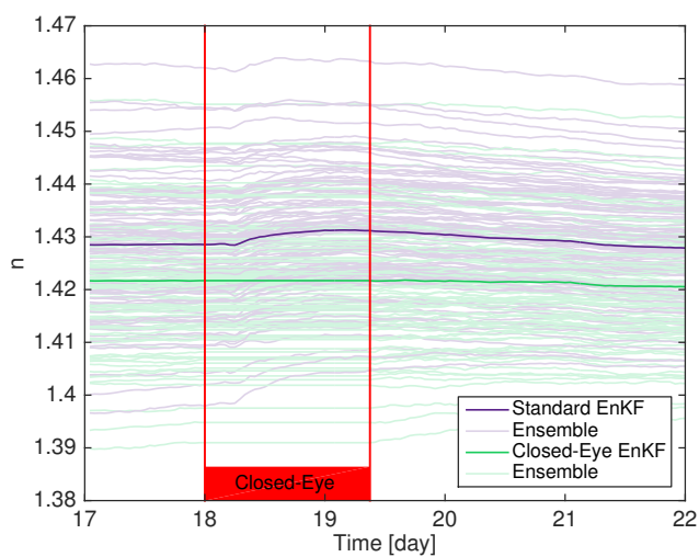
Figure 7. Parameter n during the last iteration of the Standard EnKF and the Closed-Eye EnKF.
