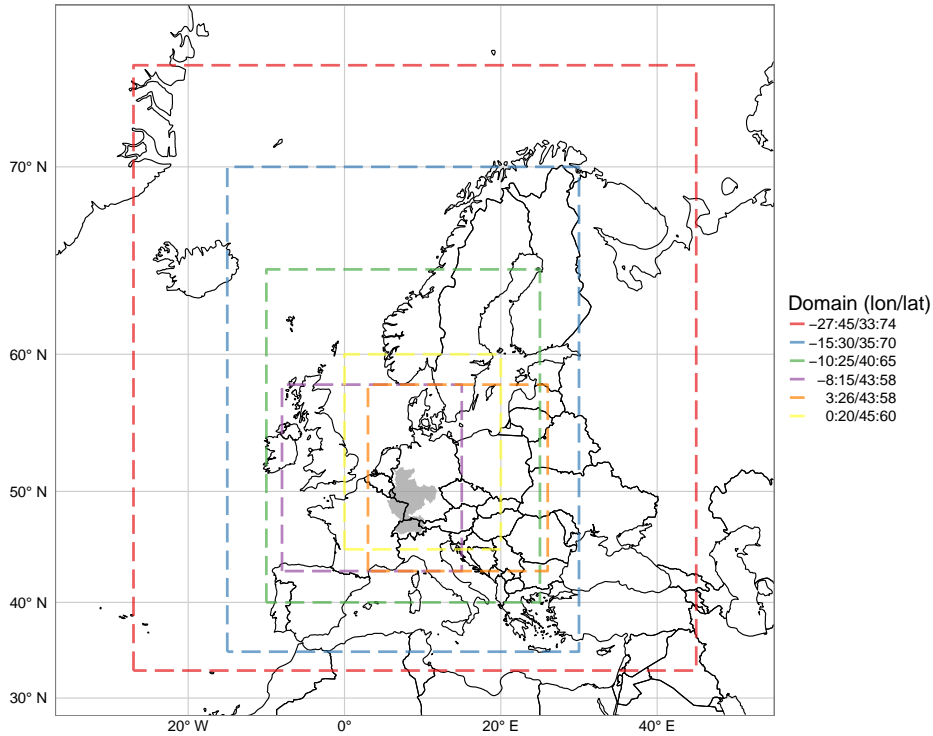
Figure 2. Spatial domains of weather pattern classifications in degree of geographic longitude/latitude . Dark grey polygon shows location of Rhine catchment. Domain 3 : 26 / 43 : 58 as in Philipp et al. (2010), region D07; -15 : 30 / 35 : 70 as in Nied et al. (2014).
