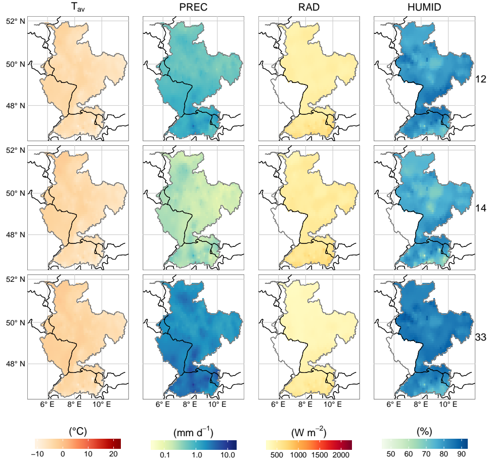
Figure 3. Average daily values of meteorological variables for selected-pattern example patterns 12, 14, and 33 to emphasise the need of multi-variate evaluation of weather pattern classifications ( T_{av} – average temperature, PREC – precipitation, RAD – global radiation, HUMID – relative humidity).
