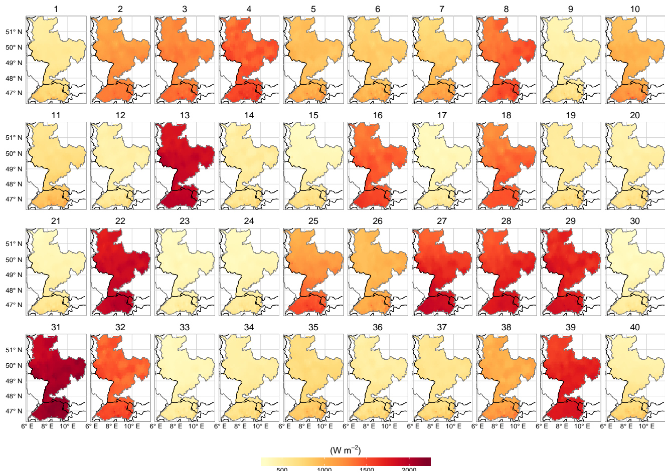
Figure 13. As in Figure 11, but for global radiation.
