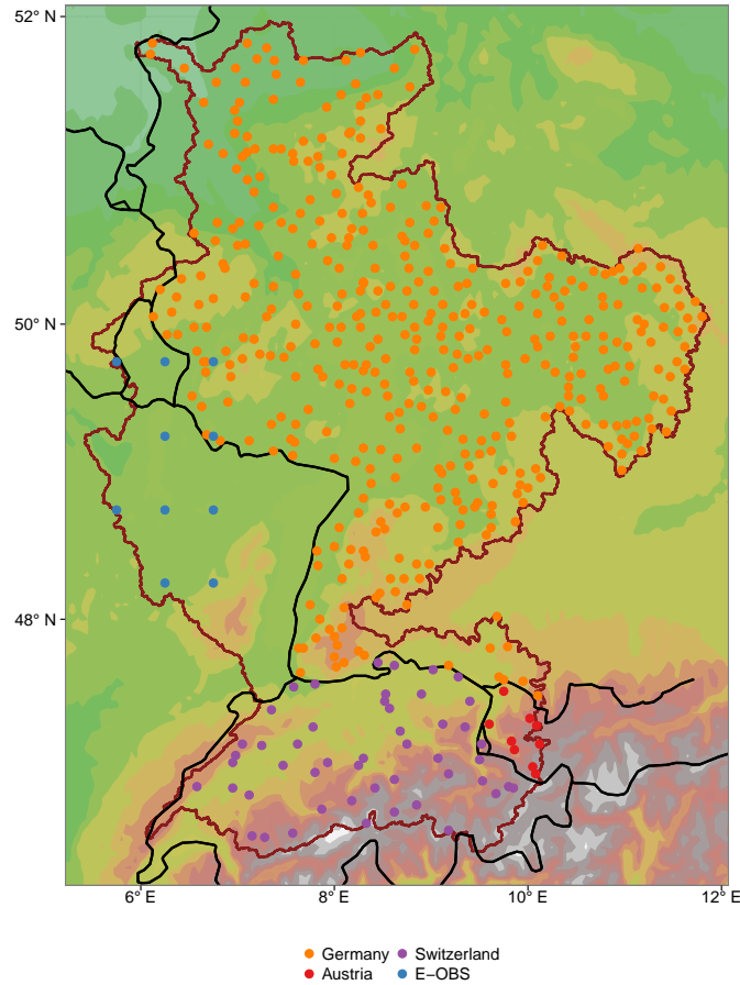
Figure 1. Locations of climate data stations used. See text for more details on single data sets. Dark red line shows Rhine catchment, black lines denote state borders.
