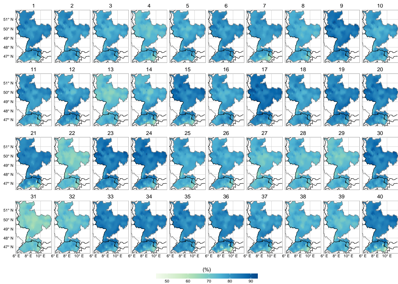
Figure 14. As in Figure 11, but for relative humidity.
