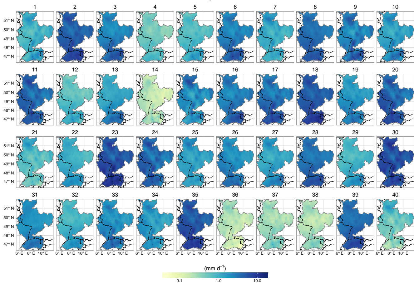
Figure 12. As in Figure 11, but for daily precipitation.
