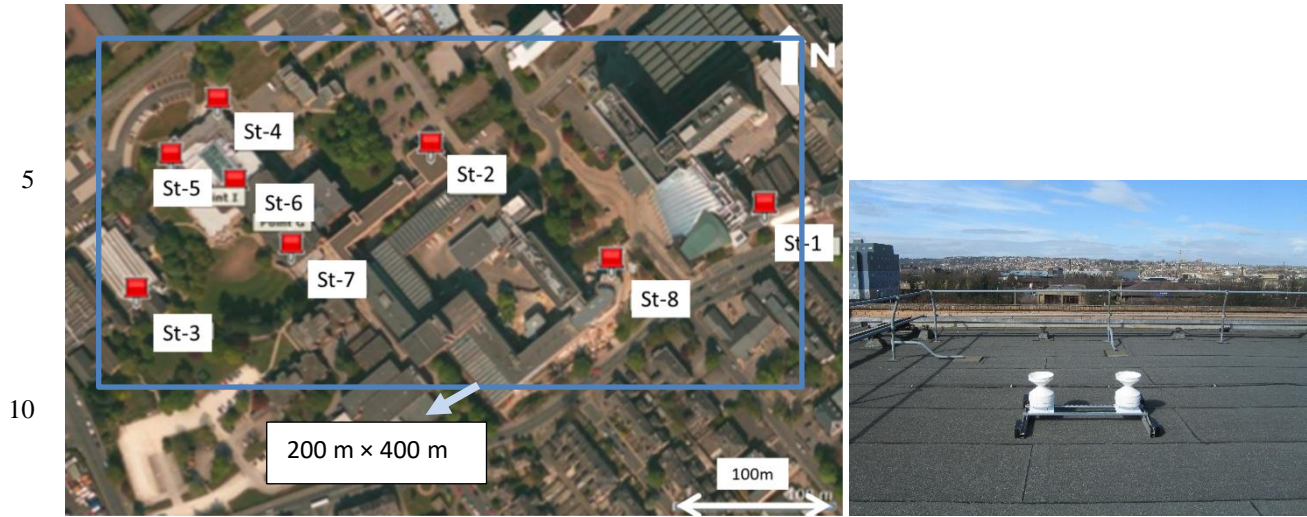
Figure 1: (Left) Aerial view of - rain gauge network covering an area of 200 \times 400 \text{ m}^2 at Bradford University, UK. (Right) A photograph of paired rain gauges at station 6.
