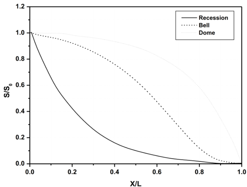
Figure 17. Three types of salt intrusion curves, in which L is the salt intrusion length, x is the distance from the mouth, S is the salinity at the mouth and S_0 is the salinity corresponding with the distance.
