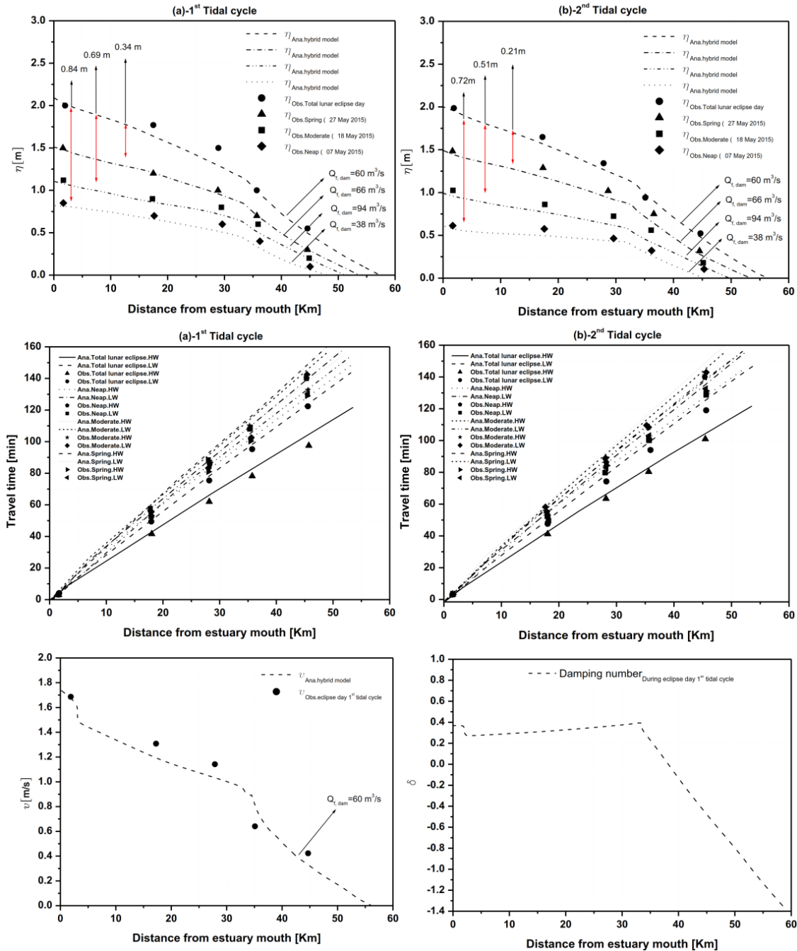
Figure 9. Analytically computed tidal amplitude, travelling time, velocity amplitude and damping number along the Sebou estuary at total lunar eclipse day (tidal amplitude, travelling time and velocity amplitude are compared against observations).
