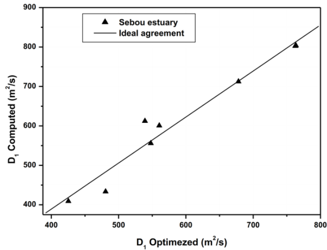
Figure 12. Comparison of computed and optimized dispersion D_1 coefficient at HWS in the spring-neap and eclipse day tides.
