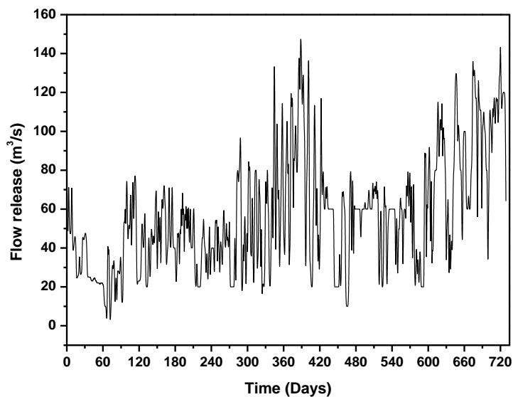
Figure 4. Flow release by Lalla Aicha dam (from 01-01-2014 to 01-01-2016).
