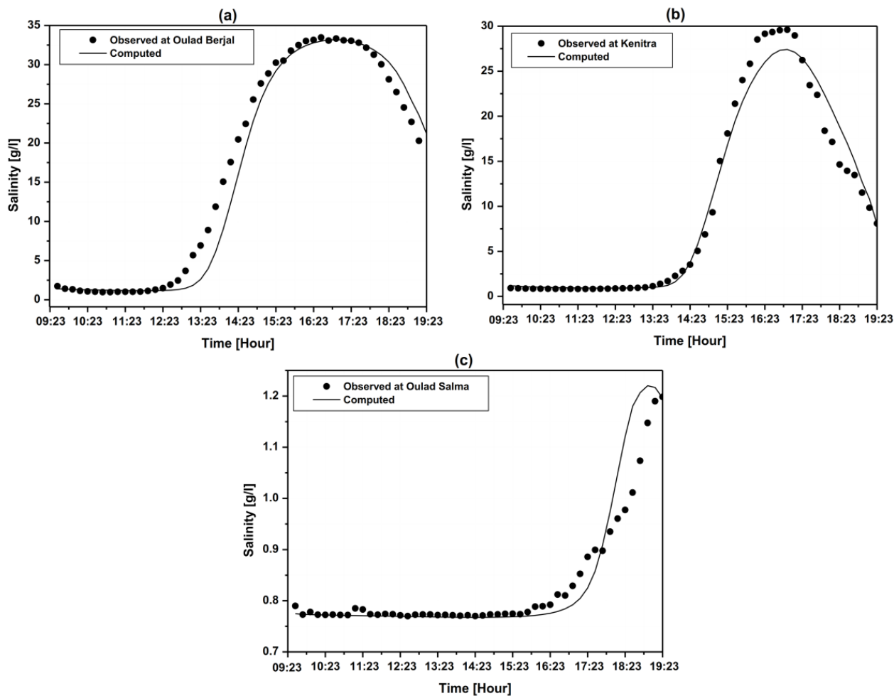
Figure 15. Salinity comparisons at Oulad Berjal (a), Kenitra (b) and Oulad Salma (c) in calibration.
