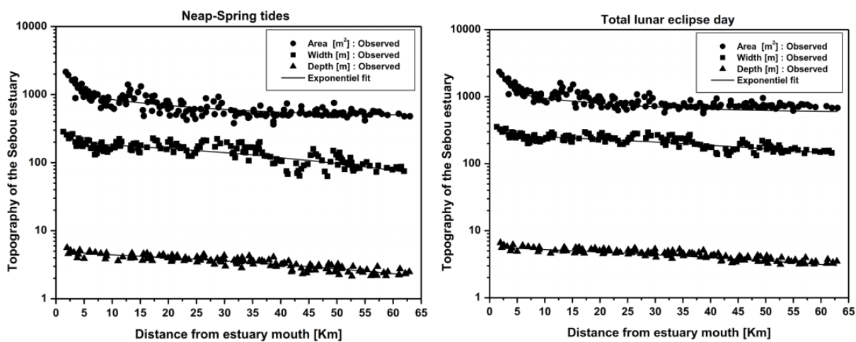
Figure 5. Geometry of the Sebou estuary, showing the cross-sectional area A ( m^2 ), the width B (m), and the estuary depth h (m) during neap-spring and total lunar eclipse tides.
