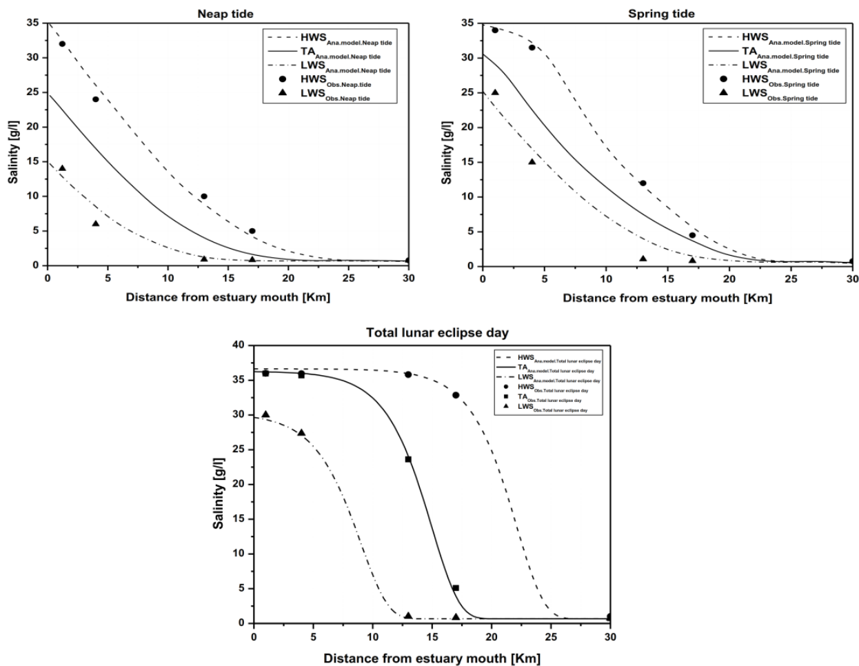
5 Figure 16. Salinity distributions in the Sebou estuary during spring tide, neap tide and total lunar eclipse day.
