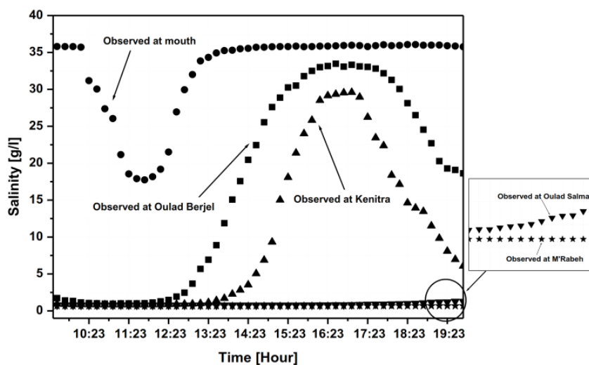
Figure 6. Salinity evolution in the Sebou river estuary during 12-h (Surveyed on 28 September 2015).
