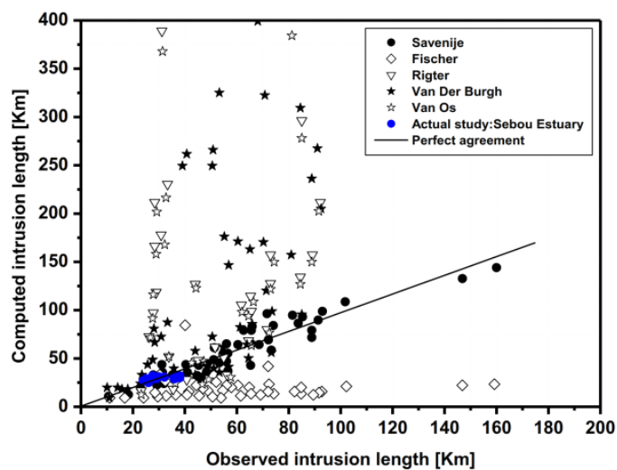
Figure 13. Comparison of different methods to compute the intrusion length at HWS and actual study (Sebou estuary)
