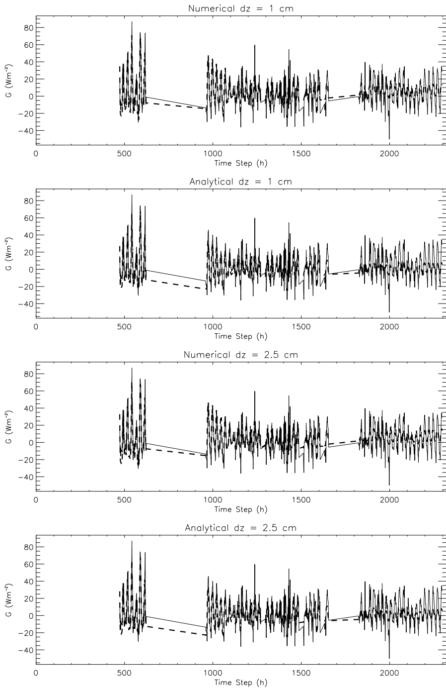
Figure 1: Comparison of the modeled ground heat flux to the observations. Observations are in solid lines, simulations in thick dashed lines.
