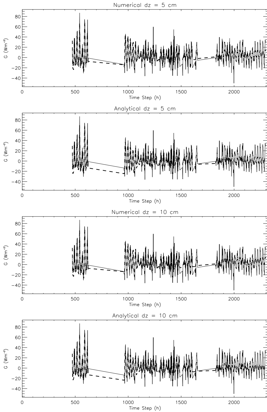
Figure 2: Comparison of the modeled ground heat flux to the observations. Observations are in solid lines, simulations in thick dashed lines.
