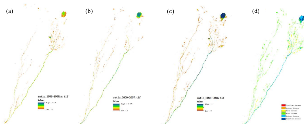
Figure 5: Frequency of inundation for (a) period 1 (1988–1998), (b) period 2 (2000–2007) and (c) period 3 (2008–2015); and (d) the changes of rate between periods 1 and 3.
