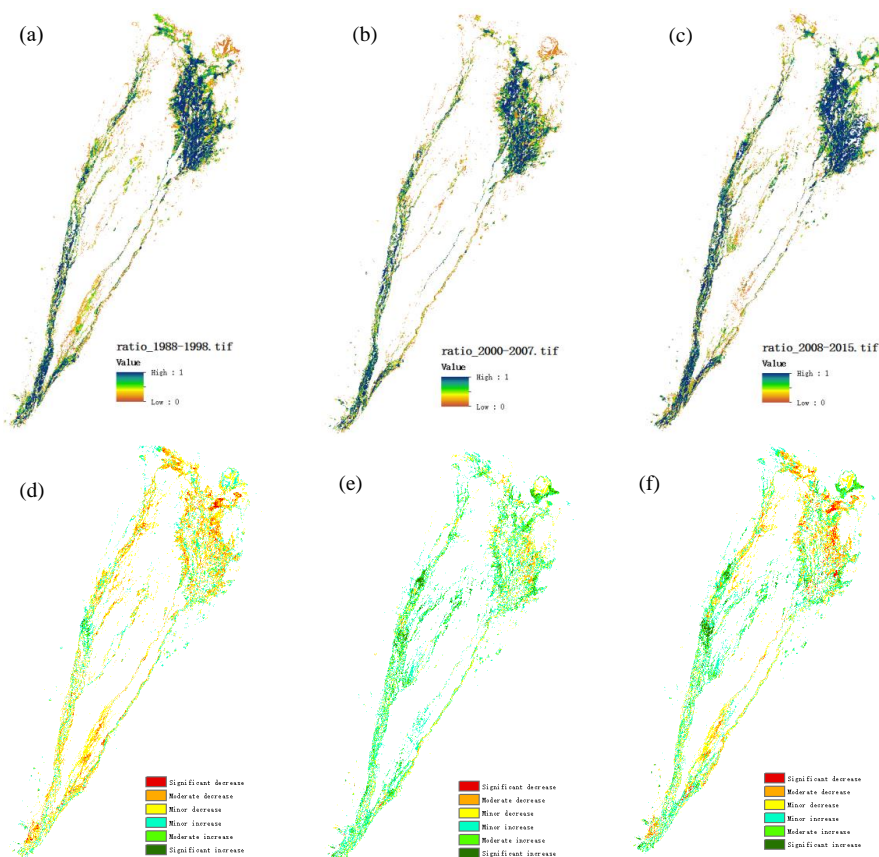
Figure 4: Spatial distribution of vegetation covered regions in Ejina Oasis. The upper row shows the frequency of vegetation distribution for the three periods: (a) period 1 (1988–1998), (b) period 2 (2000–2007) and (c) period 3 (2008–2015). The lower row shows the corresponding changes between the pairs of periods: (d) changes between periods 1 and 2, (e) changes between periods 2 and 3 and (f) changes between periods 1 and 3.
