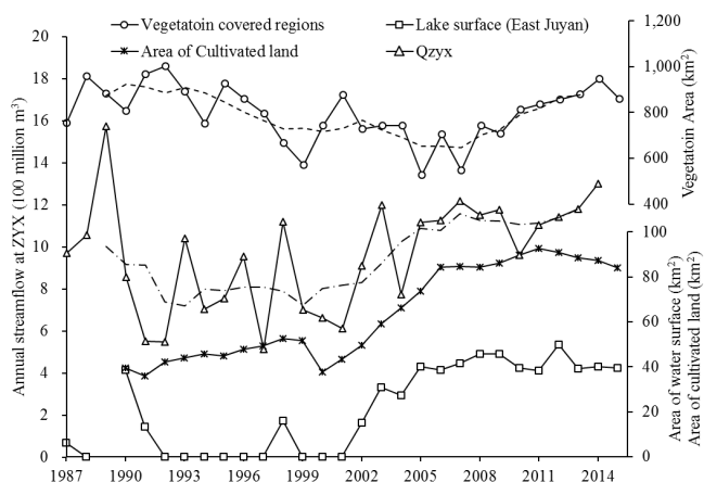
Figure 3: Temporal variations in river discharge at ZYX (triangle), annual total vegetation covered regions (circle), East Juyan Lake surface area (square) and cultivated lands (cross) from 1987 to 2015. The dash line and dash-dot line denote the 5-year moving average values for vegetation areas and streamflow at ZYX respectively.
