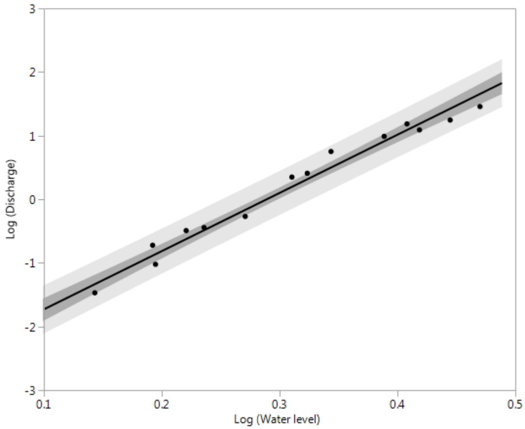
Figure 2: Discharge rating curve plotted on the log-transformed scale showing 95% confidence interval for the regression line (dark grey) and for new predictions (light grey). Stage-discharge rating curve: \log(\text{discharge}) = (9.0819 \cdot \log(\text{water level})) - 2.6423 ( n=15 , R^2=0.98 )
