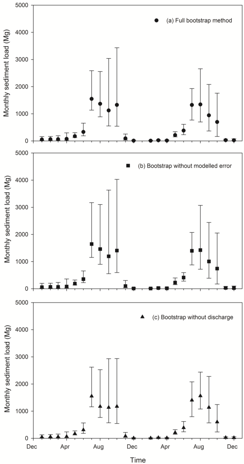
730 Figure 6: Monthly sediment load estimates (in Mg per year) for the two years of the study with 95% confidence interval limits for the three different bootstrap methods: (a) the full method shown in Figure 1, (b) the method without modelled error (i.e. leaving out Step 3 in Figure 1) and (c) the method without bootstrapping discharge (i.e. leaving out Step 1 in Figure 1). In January 2011, discharge was zero; therefore no sediment load was transported during this month.
