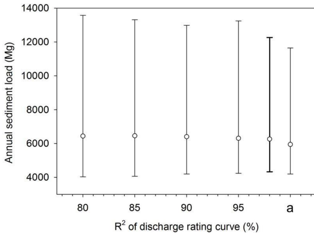
745 Figure 9: Change in median and 95% confidence intervals for the sediment load estimate of 2010 (in Mg) when decreasing the coefficient of determination of the discharge rating curve. The bold line indicates the CI width of the real (Q,h) dataset. The letter “a” corresponds to not bootstrapping the (Q,h) pairs.
